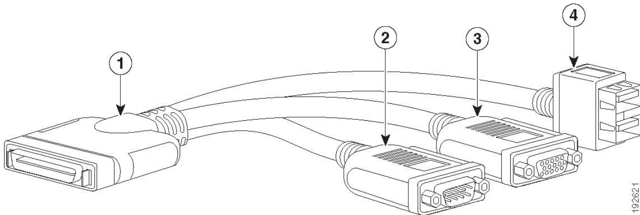
Figure 18 KVM Cable
