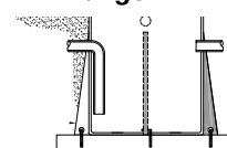
+ RAF Reinforcing Anchor Flange
