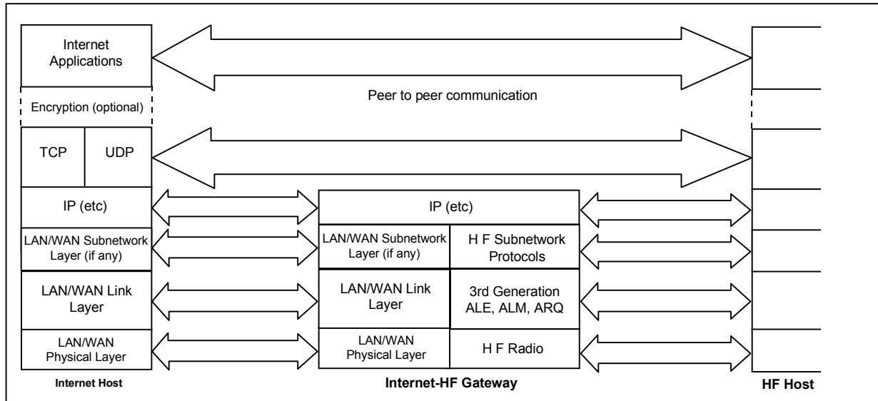
FIGURE E-2. Application interoperation via internet gateway.
