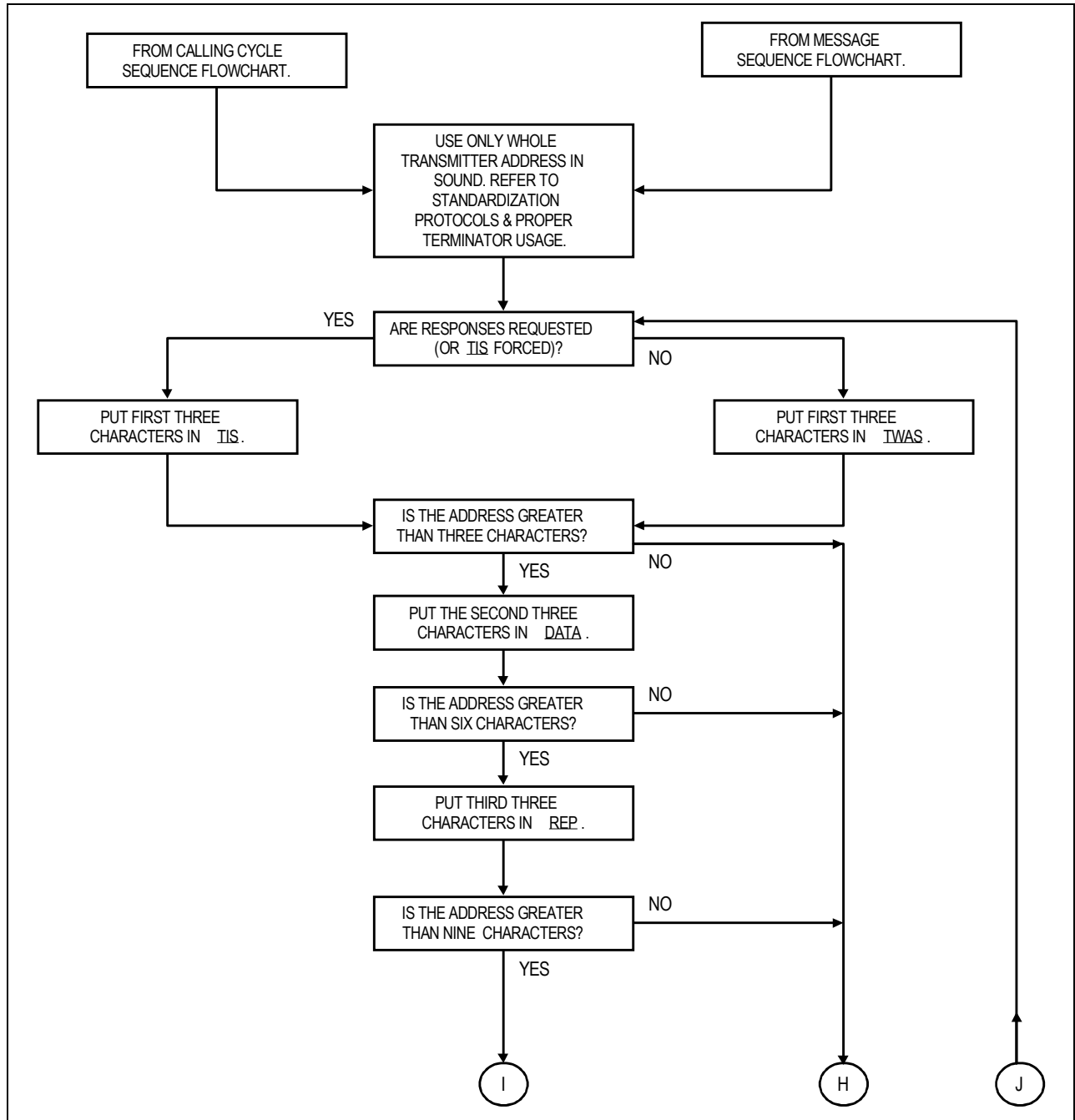
FIGURE A-17. Conclusion (terminator) sequences.
