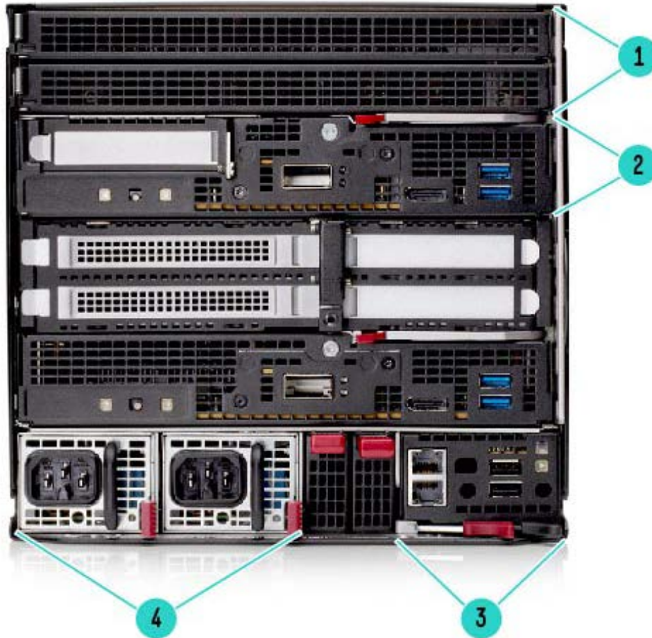
HPE ProLiant DX8000 5U Front Cabling Chassis View
