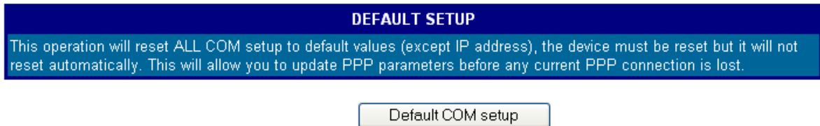
Figure 30: eWON Reset to default page
