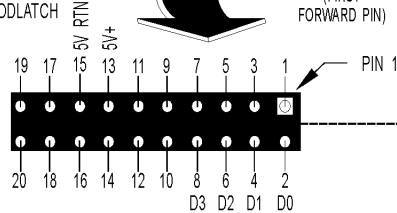
SNAP DIGITAL MODULE BASE CONTROL CONNECTOR (BOTTOM VIEW)
