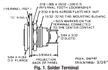
Fig. 1. Solder Terminal
