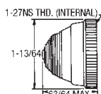
Fig. 3. Torpedo Lens
