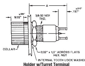
Holder w/Turret Terminal
