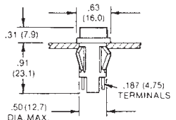
Fig. 3 Wire Leads Q.C. Terminals Shown
