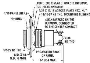
Fig. 2. Screw Terminal
