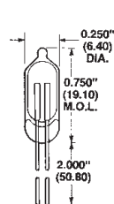
Fig. 1 Wire Leads
