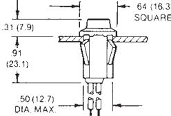
Fig. 4 Wire Leads Shown Q.C. Terminals
