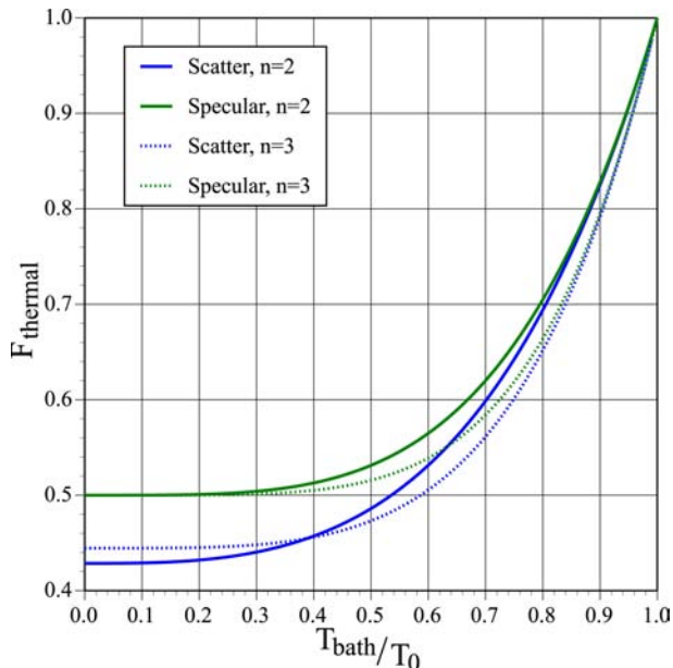
Figure 4. Thermal link functions as given by equations for specular- or scattering-dominated links in Dan McCammon’s review [43].
