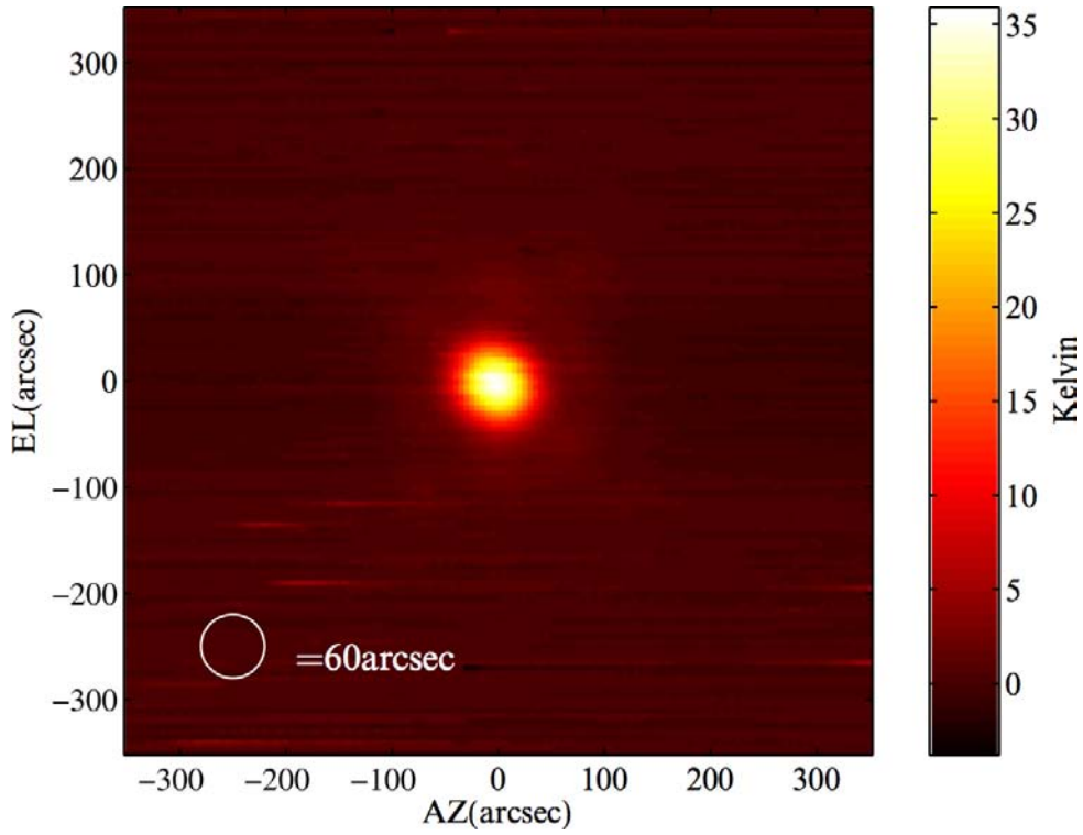
Figure 8. TES bolometer array 2 mm wavelength image of Jupiter using APEX-SZ (from Dobbs et al. [73]).
