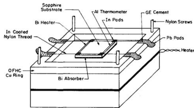
Figure 2. Superconducting bolometer demonstrated by Clarke et al. [9].
