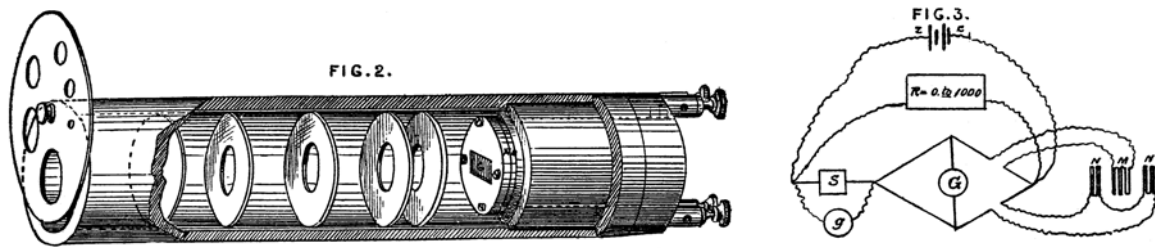
Figure 1. Bolometric instrument of S.P. Langley.
