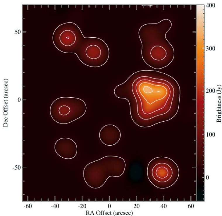
Figure 7. TES bolometer array 350 m image of the high-mass star formation region G34.3+0.2 (Benford et al. [55]).
