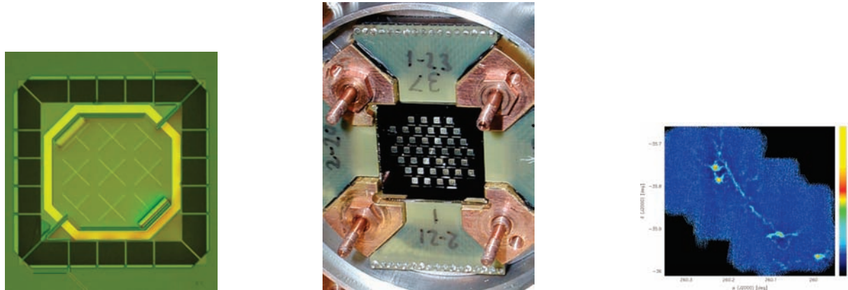
Figure 13. (Left) photos of the 39-element horn-coupled array of TES bolometers fabricated at IPHT/Jena for the MPIfR SABOCA instrument. (Right) A 350\ \mu\text{m} image of the NGC6334 star forming region.
