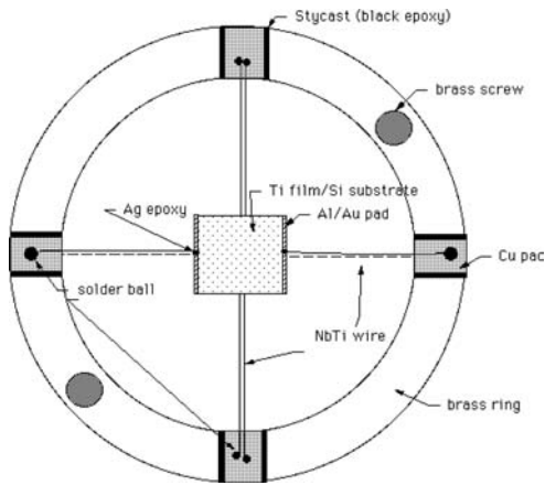
Figure 5. (Left) The layout of an early voltage-biased superconducting bolometer (e.g., [12]) is reminiscent of that in Figure 2 . (Right) The all-lithographic version (e.g., [45]) made large-format arrays possible.
