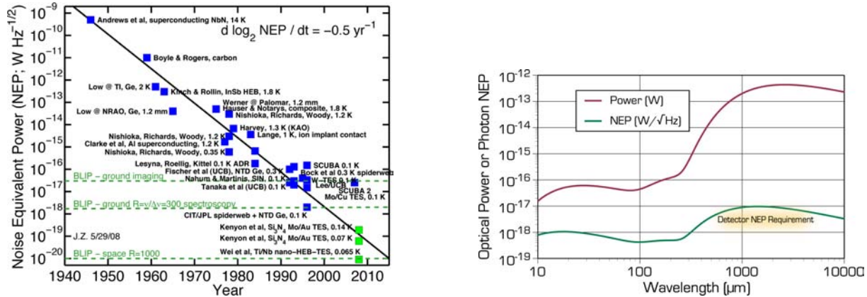
Figure 15. (Left) The NEP of bolometers has improved a factor of two every two years for more than half a century (figure courtesy of Jonas Zmuidzinas). (Right) The natural sky backgrounds in space require detectors of a sensitivity that is now easily reached by bolometers. Larger format arrays continue to improve the effective mapping speed of fielded instruments where background-limited sensitivity has been achieved.
