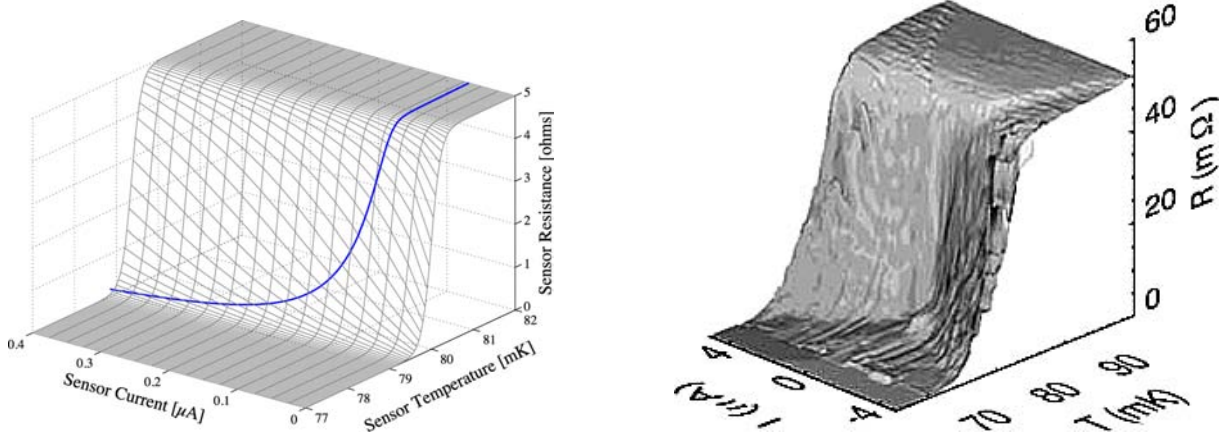
Figure 3. (Left) A modeled resistance function R(T, I) , showing the path followed during a bias sweep; adapted from a figure by Blas Cabrera [40]; (Right) Measurements of the R(T, I) surface by Lindeman et al. [41], showing the shape of the transition in detail; note the similarity to the gross features of the model, given that the data have bipolar current.
