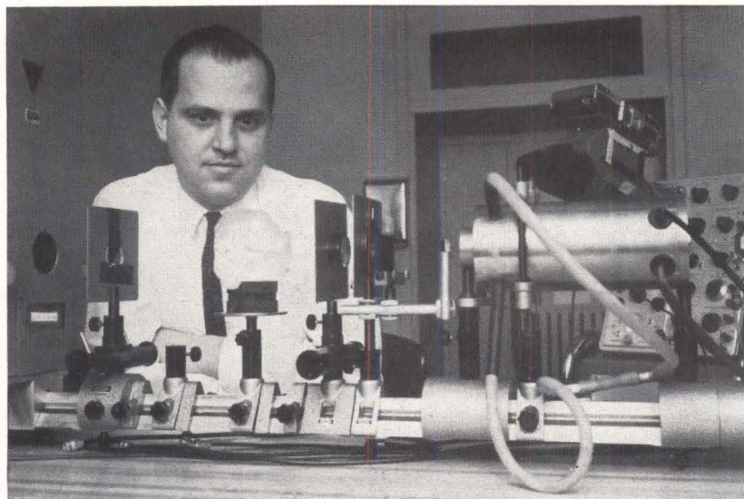
EXPERIMENTAL SETUP, shown with R. W. Terhune, consists of giant pulse ruby laser, right, ammonium dihydrogen phosphate crystal, center, and a grating spectrometer with photomultiplier to analyze the beam
