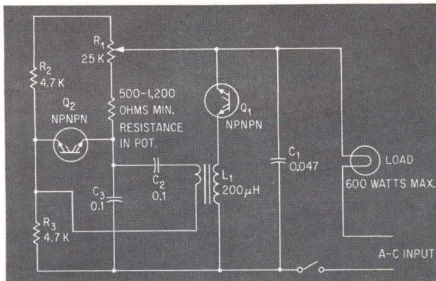
LIGHT DIMMER for fluorescent or incandescent lamps, by Hunt Electronics—Fig. 1
