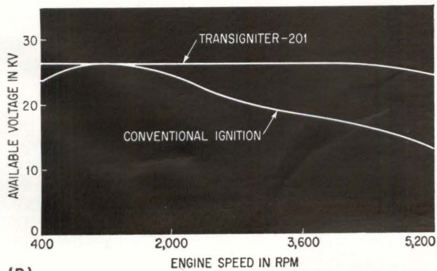
son of available voltages (B); secondary energy versus engine speed (C), with shaded area indicating the excess restrikes, which contribute to accelerated aging of the ignition system—Fig. 3
