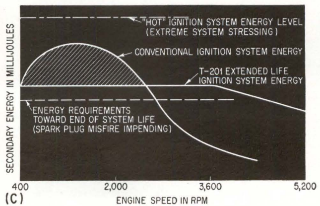
son of available voltages (B); secondary energy versus engine speed (C), with shaded area indicating the excess restrikes, which contribute to accelerated aging of the ignition system—Fig. 3
