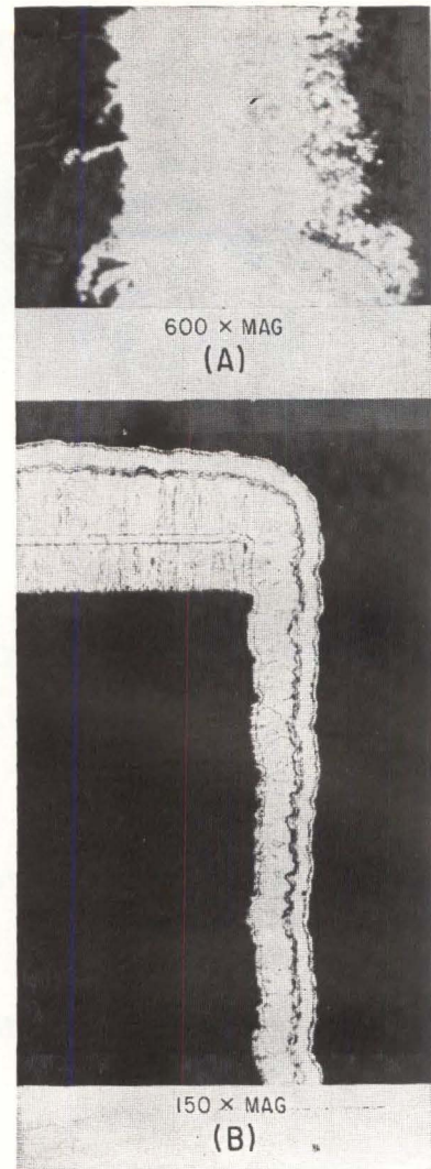
ELECTROLESS plating of copper (shown in A) is used to accept final electrolytic plating of copper. Electroplated copper with solder overplate is shown lying over electroless copper (B)—Fig. 2
