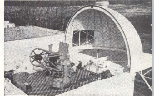
MAIN TELESCOPE. Mounted beneath it are 12-inch tracking telescope (left) and radiometer
