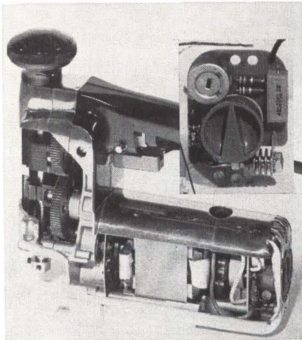
SABRE SA W cutaway view shows ser circuit board at right end, inset shows ser heat sink, cooled by motor air. By Diehl for Sears, Roebuck.
