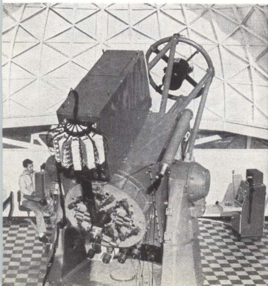
MOUNTED atop the telescope are the 30-channel spectrometer covering visible spectra from 0.3 to 0.6 micron, and the 10-channel one for 0.6 and 4 micron
