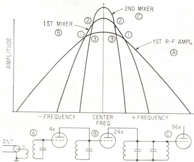
FRONT-END receiver selectivity curves considering stage-by-stage amplification—Fig. 2
