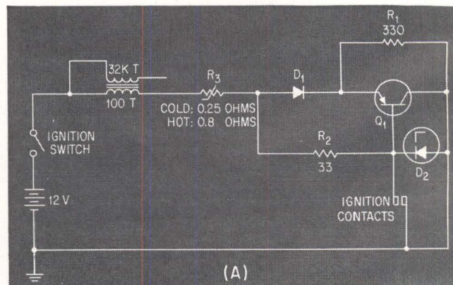
TRANSISTOR IGNITION by Prestolite (A); compari-energy region that creates excess spark trailing and
