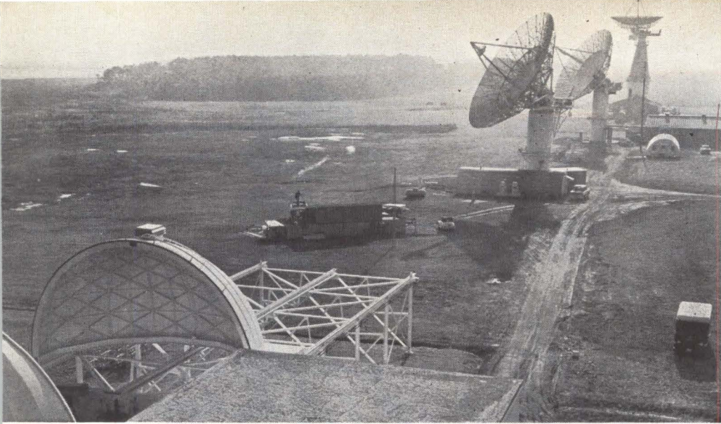
ARBUCKLE NECK site includes, from left, houses for the telescope and meteor cameras, S-band tracking radar, combined uhf and X-band radars, and a trajectory and range safety radar. Trailblazer reentry rockets are fired from nearby Wallops Station.
