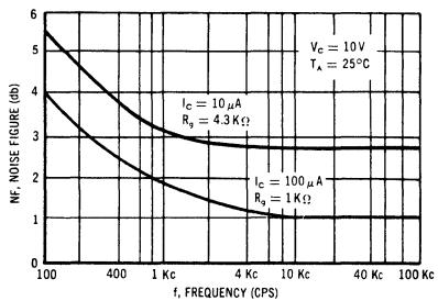
NOISE FIGURE versus FREQUENCY
