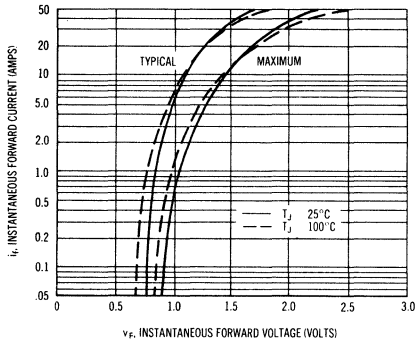
FORWARD CONDUCTING CHARACTERISTICS (ALL TYPES)
