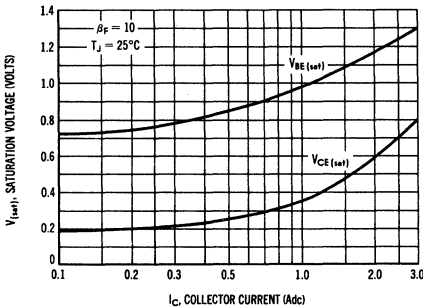
SATURATION VOLTAGES
