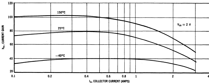
CURRENT GAIN VARIATIONS
