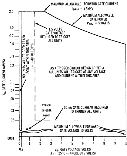
GATE TRIGGER CHARACTERISTICS
