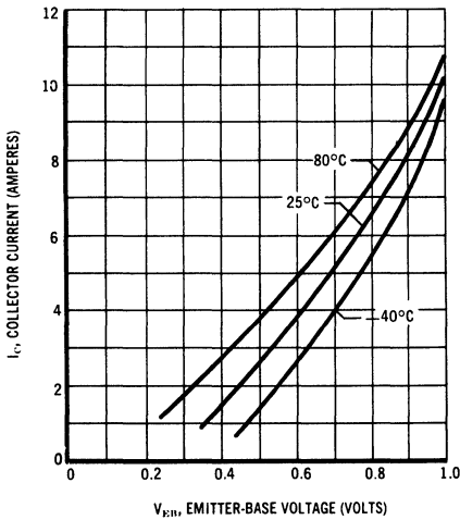
TRANSCONDUCTANCE CHARACTERISTICS
