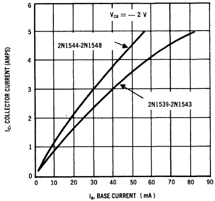
COLLECTOR CURRENT versus BASE CURRENT
