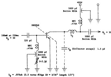
250 MC POWER GAIN TEST CIRCUIT (2N3137)
