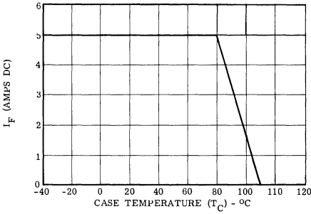
CURRENT RATING
