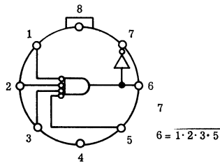
NEGATIVE LOGIC
