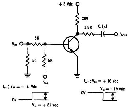
TURN-ON AND TURN-OFF TIME TEST CIRCUIT
