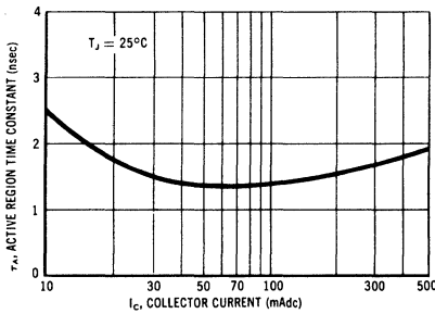
ACTIVE REGION TIME CONSTANT
