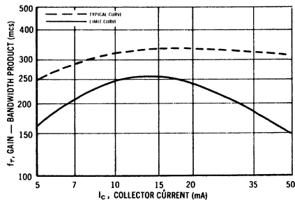
GAIN-BANDWIDTH PRODUCT CHARACTERISTICS
