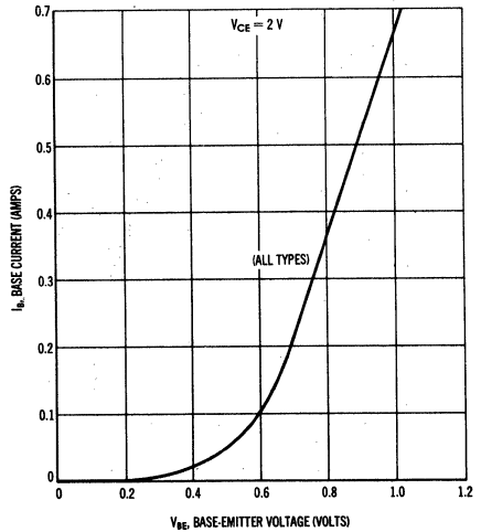
BASE CURRENT versus BASE-EMITTER VOLTAGE
