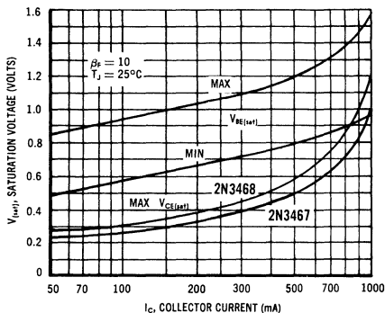
LIMITS OF SATURATION VOLTAGE
