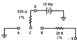
TERMINAL TEST CONNECTIONS DIFFERENTIAL VOLTAGE
