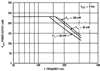
POWER OUTPUT versus FREQUENCY
