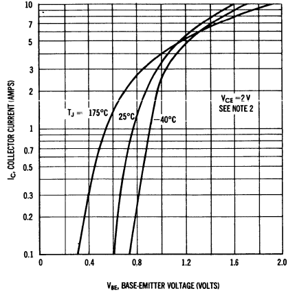
COLLECTOR CURRENT-VOLTAGE VARIATIONS
