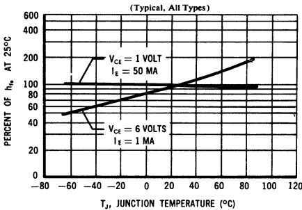
SMALL SIGNAL CURRENT GAIN( h_{fe} ) versus TEMPERATURE
