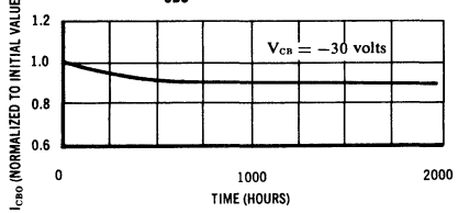
I_{CBO} VARIATION WITH TIME
