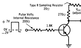
SWITCHING TIME TEST CIRCUIT
