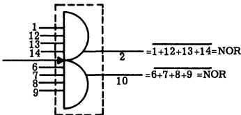
NOR GATE
