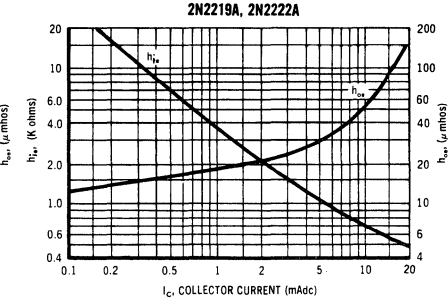
SMALL SIGNAL INPUT IMPEDANCE AND OUTPUT CONDUCTANCE versus COLLECTOR CURRENT ( V_{CE} = 10\text{ V} @ 1\text{ Kc} )
