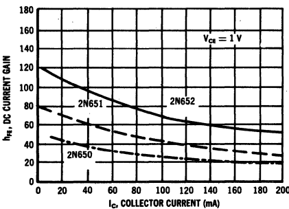
h_{FE} versus COLLECTOR CURRENT
