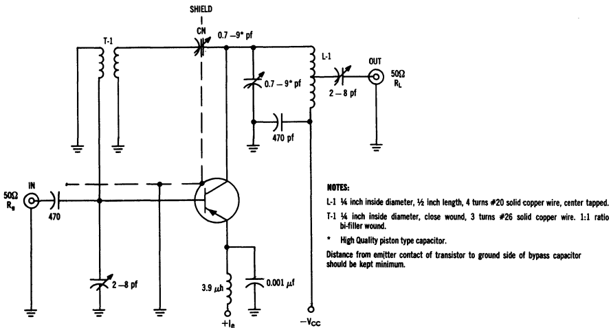
200 MC POWER GAIN AND NOISE FIGURE TEST CIRCUIT
