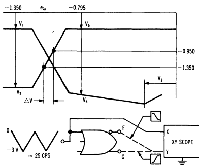
DEFINITION OF TRANSFER CHARACTERISTIC POINTS
