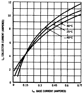
CURRENT TRANSFER CHARACTERISTICS
