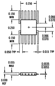
14-LEAD FLAT PACKAGE CASE 83
