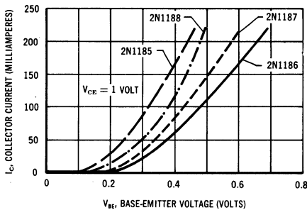
OUTPUT CURRENT versus BASE DRIVE VOLTAGE
