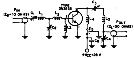
RF AMPLIFIER CIRCUIT FOR 2N3553 POWER-OUTPUT TEST (260-Mc Operation)
