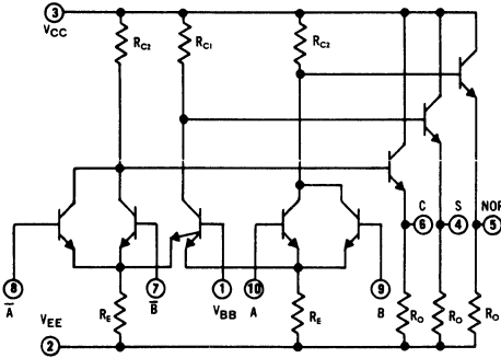
CIRCUIT SCHEMATIC
