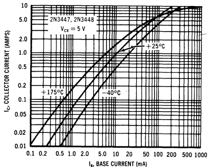
COLLECTOR CURRENT versus BASE CURRENT
