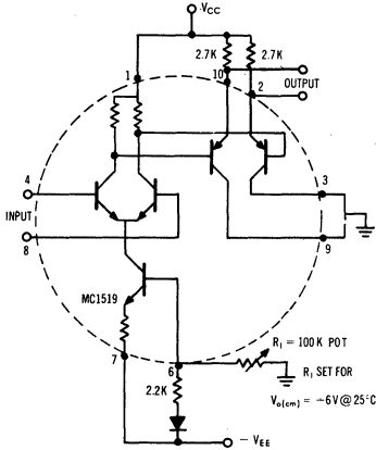
CIRCUIT B COMMON COLLECTOR OUTPUT
