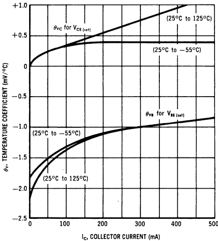
TEMPERATURE COEFFICIENTS
