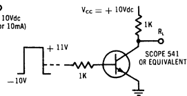
MEASUREMENT CIRCUIT
