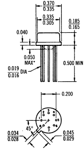
8-LEAD TO-5 PACKAGE CASE 96, 96A
