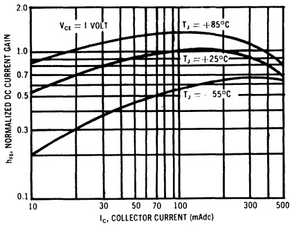
NORMALIZED CURRENT GAIN CHARACTERISTICS
