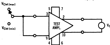
COMMON MODE REJECTION
