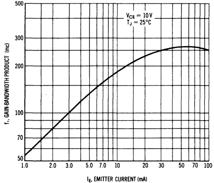
GAIN-BANDWIDTH PRODUCT
