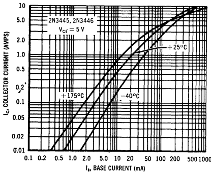
COLLECTOR CURRENT versus BASE CURRENT
