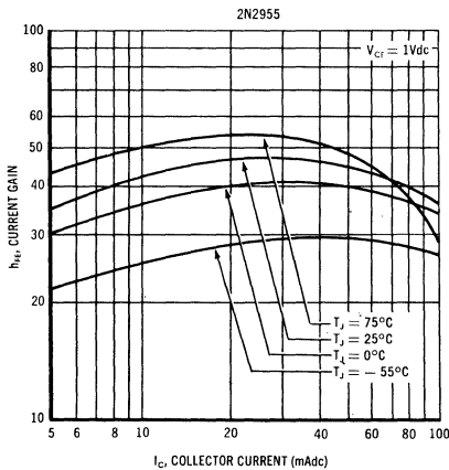
CURRENT GAIN CHARACTERISTICS
