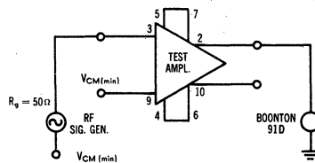
BANDWIDTH
