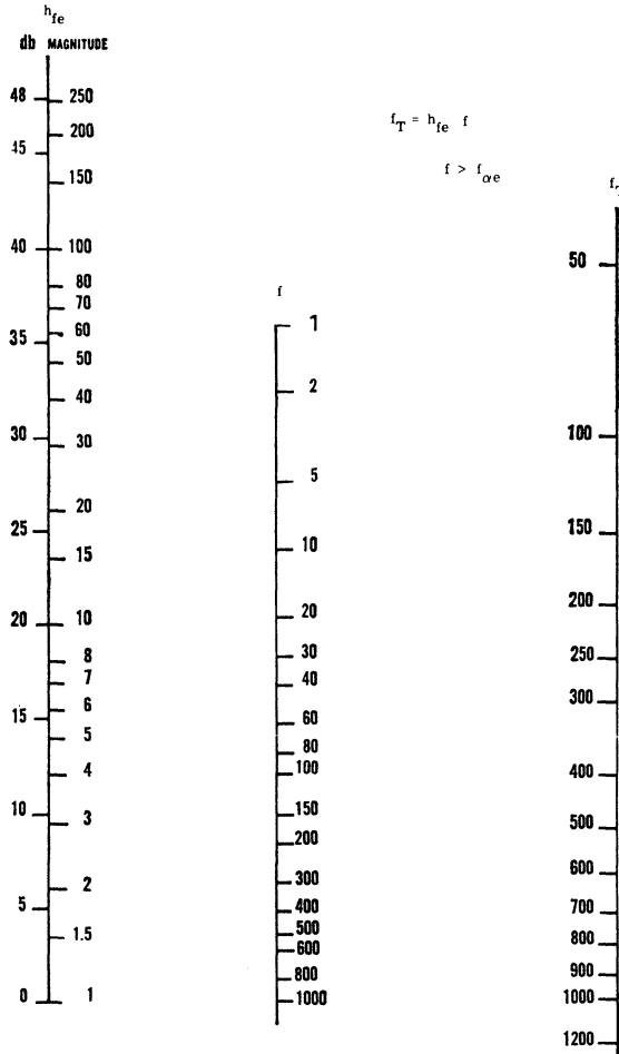
Fig. 4. This nomogram is useful in finding h_{fe} when a frequency f > f_{\alpha e} .
