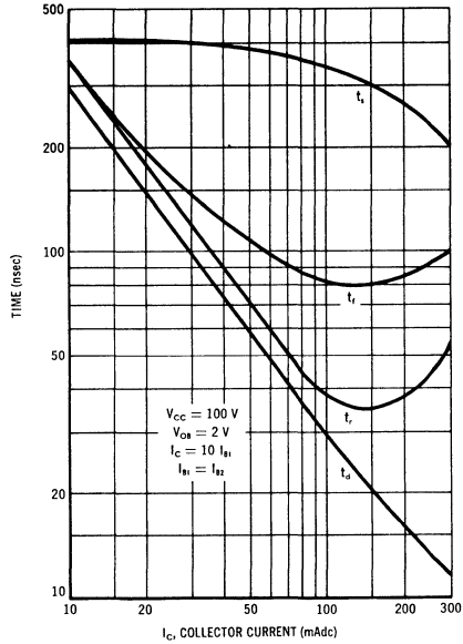
SWITCHING TIMES
