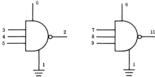
3-3 NAND/NOR GATE
