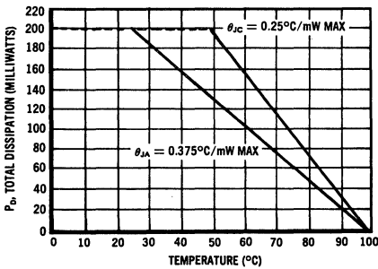
POWER-TEMPERATURE DERATING CURVE
