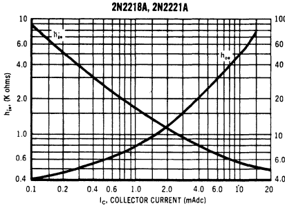
SMALL SIGNAL INPUT IMPEDANCE AND OUTPUT CONDUCTANCE versus COLLECTOR CURRENT ( V_{CE} = 10\text{ V} @ 1\text{ Kc} )
