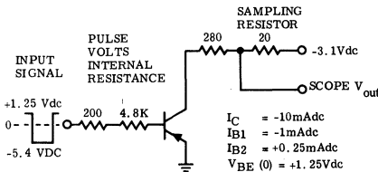
10mA SWITCHING TIME TEST CIRCUIT FIGURE 1
