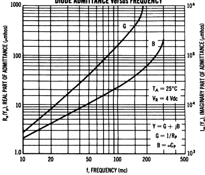
PARALLEL EQUIVALENT DIODE ADMITTANCE versus FREQUENCY
