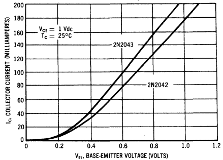
COLLECTOR CURRENT versus BASE-DRIVE VOLTAGE
