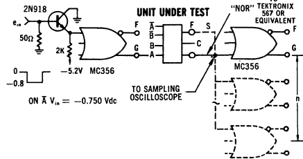
PROPAGATION DELAY TIME
