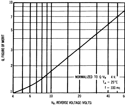
FIGURE OF MERIT versus REVERSE VOLTAGE
