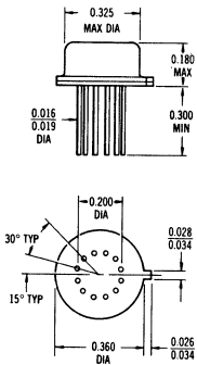
CASE 87
