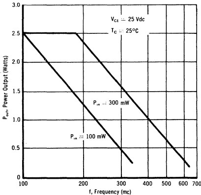
POWER versus FREQUENCY
