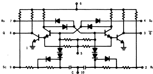
BINARY ELEMENT MC209
