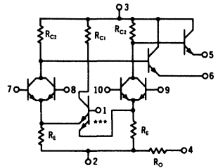
MC312G DUAL "NOR"
