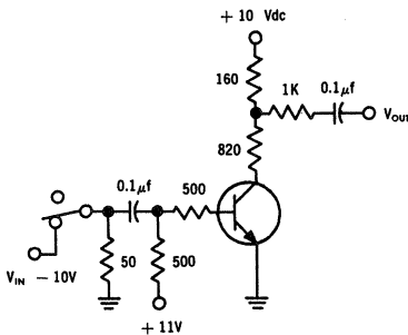
CHARGE STORAGE TIME CONSTANT TEST CIRCUIT
