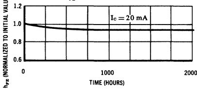
h_{FE} VARIATION WITH TIME
