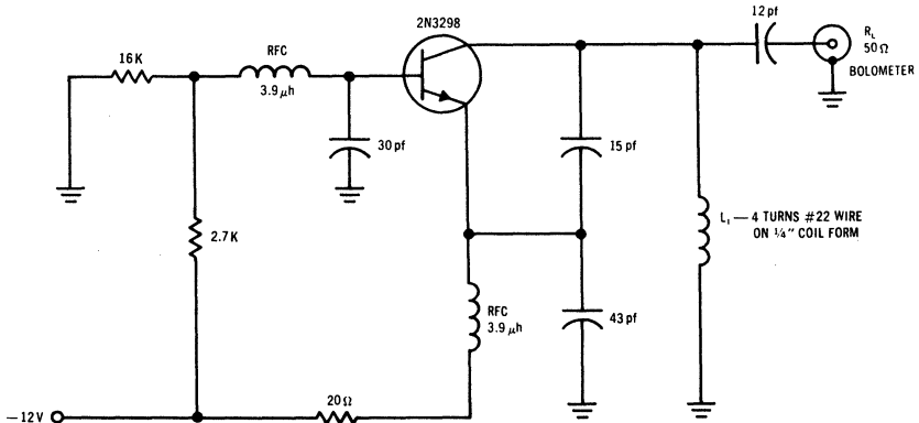
80 MC OSCILLATOR POWER OUTPUT TEST CIRCUIT
