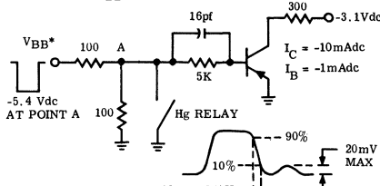
10mA TOTAL CONTROL CHARGE TEST CIRCUIT FIGURE 3
