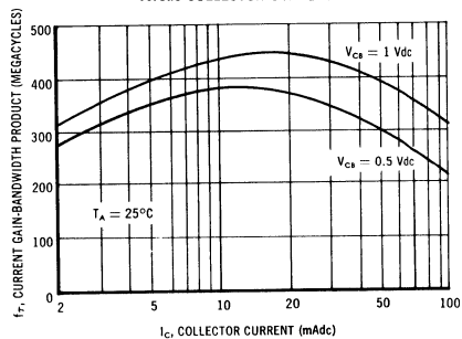
CURRENT GAIN-BANDWIDTH PRODUCT ( f_T ) versus COLLECTOR CURRENT
