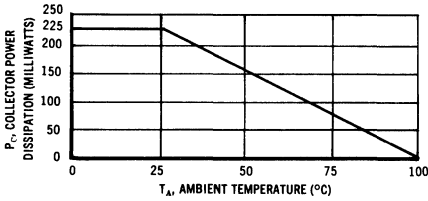
POWER-TEMPERATURE DERATING CURVE
