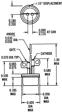
CASE 87
