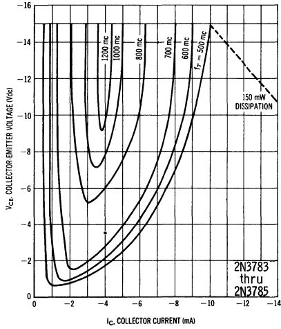
CONTOURS OF CURRENT-GAIN BANDWIDTH PRODUCT — f_T
