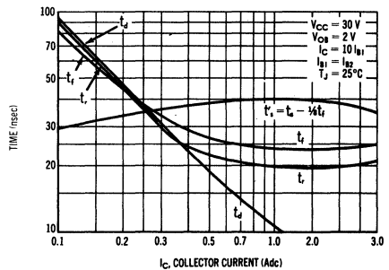
SWITCHING TIMES
