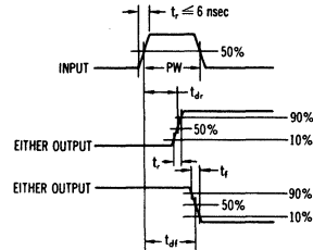
SWITCHING WAVEFORMS
