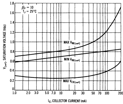
LIMITS OF SATURATION VOLTAGES
