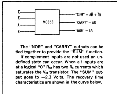
LOGIC SPECIFICATIONS
