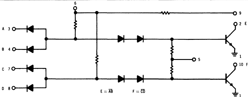
2-2 NAND/NOR GATE
