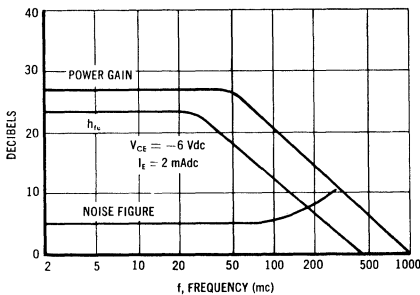
POWER GAIN, CURRENT GAIN, & NOISE FIGURE vs. FREQUENCY
