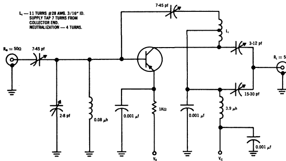
FIGURE 2: 10MC POWER GAIN TEST CIRCUIT — 2N3324
