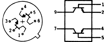
PIN CONNECTIONS BOTTOM VIEW
