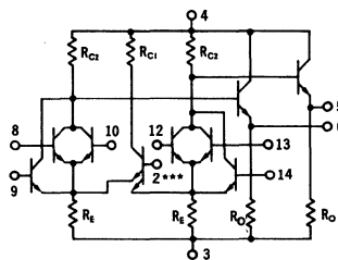
MC312F DUAL "NOR"
