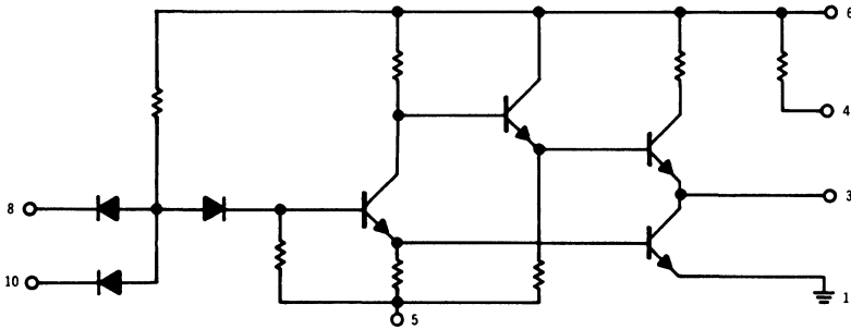
LINE DRIVER MC205
