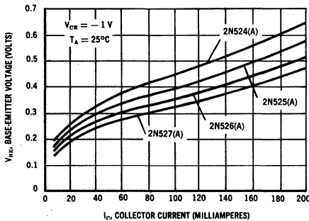
COMMON EMITTER INPUT VOLTAGE versus COLLECTOR CURRENT
