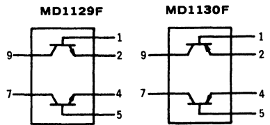
PIN CONNECTIONS BOTTOM VIEW
