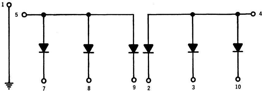
DUAL DIODE ARRAY
