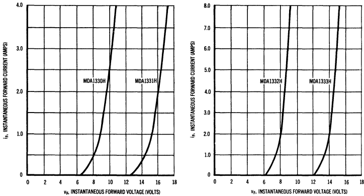
TYPICAL FORWARD CHARACTERISTICS ( T_J = 25^\circ\text{C} )
