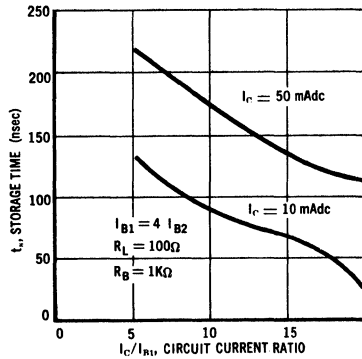
STORAGE TIME versus CIRCUIT CURRENT RATIO
