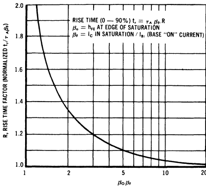
RISE TIME FACTOR
