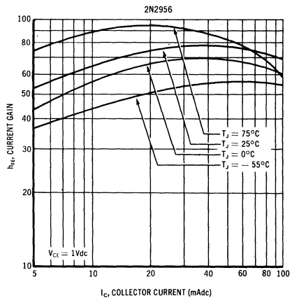
CURRENT GAIN CHARACTERISTICS
