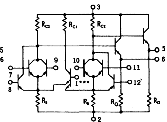
MC312G DUAL "NOR"
