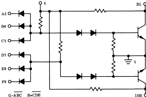
3-3 NAND/NOR GATE
