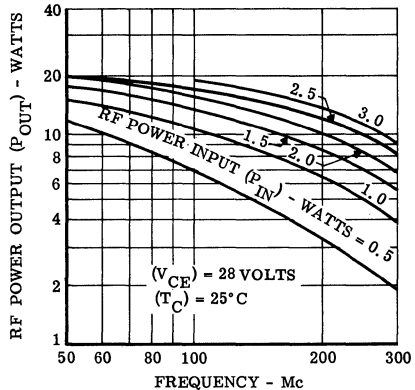
POWER OUTPUT versus FREQUENCY
