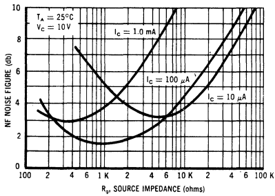
1KC NOISE FIGURE versus SOURCE IMPEDANCE
