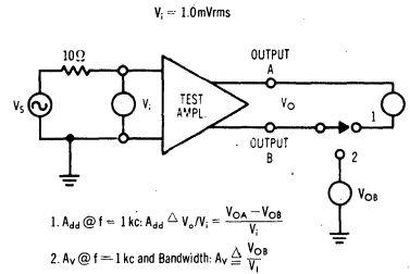
DIFFERENTIAL VOLTAGE GAIN SINGLE ENDED VOLTAGE GAIN AND BANDWIDTH
