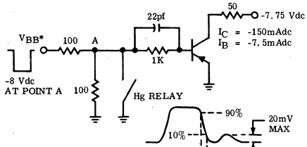
150mA TOTAL CONTROL CHARGE TEST CIRCUIT FIGURE 4
