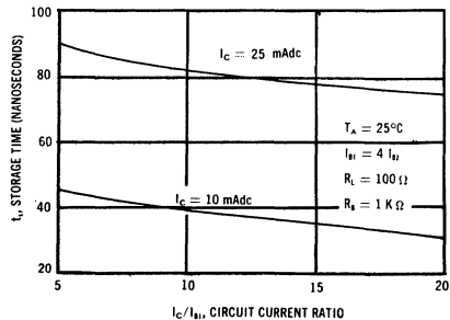
STORAGE TIME versus CIRCUIT CURRENT RATIO
