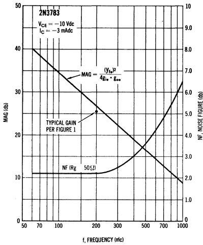
MAG & MAXIMUM NF versus FREQUENCY
