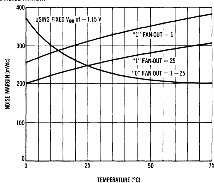
WORST CASE NOISE MARGIN
