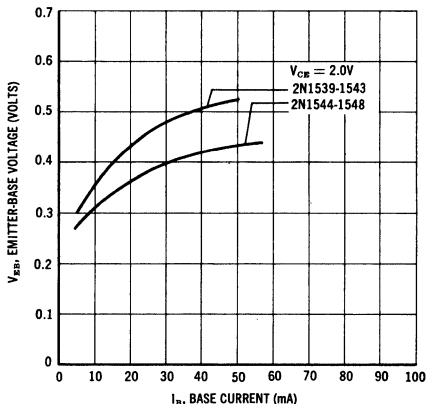
Figure 5 — Emitter-Base Voltage versus Base Current
