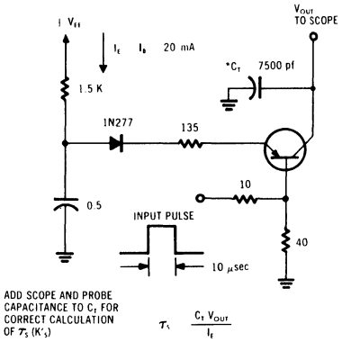
CARRIER STORAGE TIME CONSTANT TEST CIRCUIT
