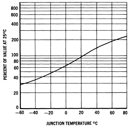
SMALL SIGNAL CURRENT GAIN versus TEMPERATURE
