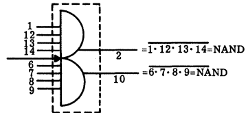
NAND GATE
