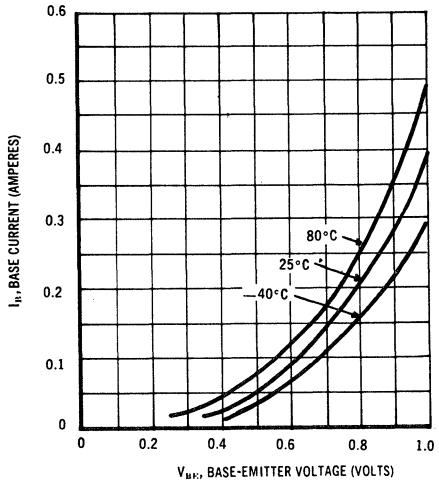
INPUT CHARACTERISTICS
