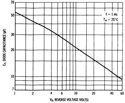
DIODE CAPACITANCE versus REVERSE VOLTAGE
