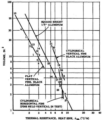
Figure 7 - Volume vs. \theta_{SA} .
