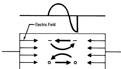
Figure 6 — When a forward voltage is applied, carriers are injected across the junction. However, before they can combine and result in a dc current flow, the applied voltage reverses and the carriers are returned to the point of origin in a bunch. This results in an abrupt cessation of reverse current and the waveform is rich in harmonics.
