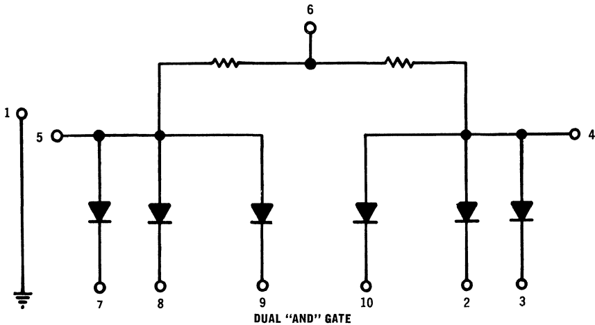
CIRCUIT SCHEMATIC
