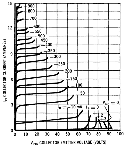
OUTPUT CHARACTERISTICS
