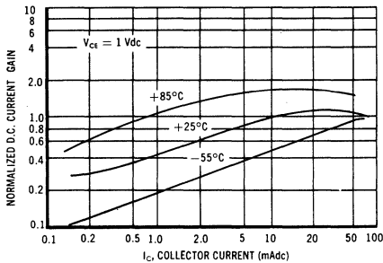
NORMALIZED D.C. CURRENT GAIN versus COLLECTOR CURRENT
