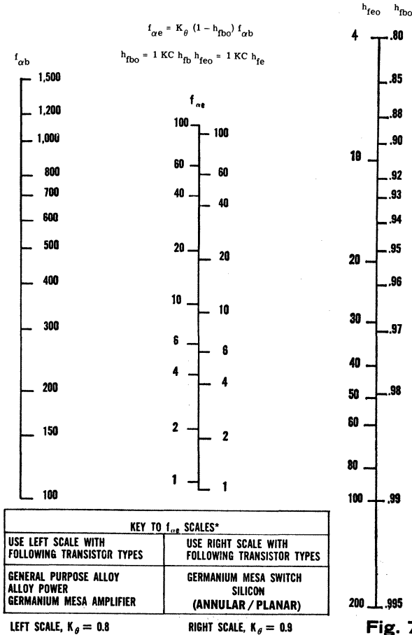
Fig. 7. Once f_{\alpha b} is known this nomogram is used to find f_{\alpha e} .
