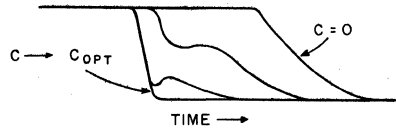
TURN-OFF WAVEFORM (PNP TRANSISTOR)
