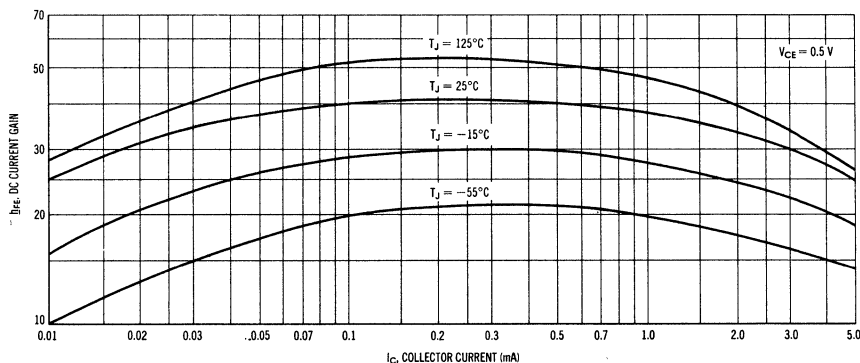
MINIMUM CURRENT GAIN CHARACTERISTICS
