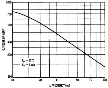
FIGURE OF MERIT versus FREQUENCY
