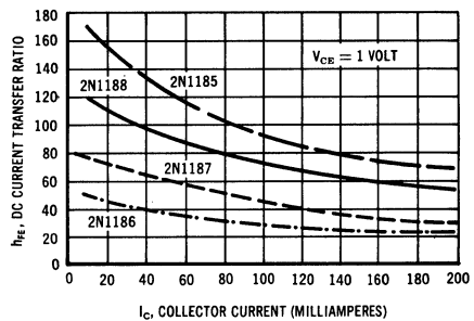
DC CURRENT TRANSFER RATIO versus COLLECTOR CURRENT
