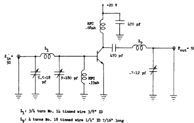
250 MC POWER GAIN TEST CIRCUIT (MM1803)
