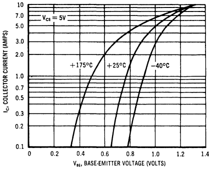
COLLECTOR CURRENT-VOLTAGE VARIATIONS
