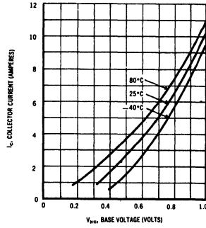
TRANSCONDUCTANCE CHARACTERISTICS
