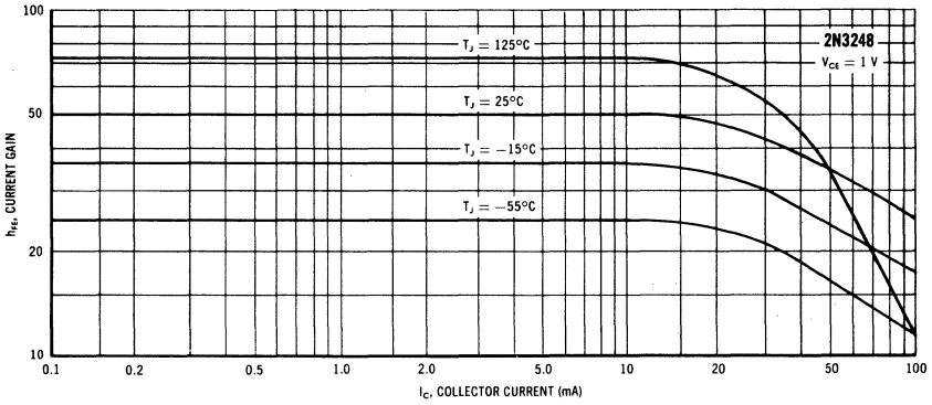
MINIMUM CURRENT GAIN
