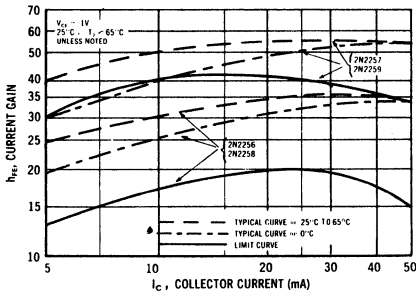
CURRENT GAIN CHARACTERISTICS
