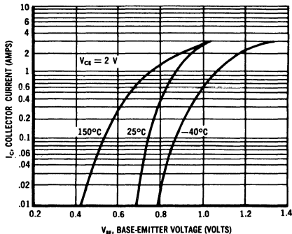
COLLECTOR CURRENT vs BASE-EMITTER VOLTAGE
