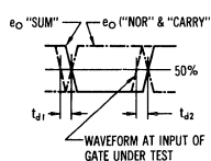
PROPAGATION DELAY TIME
