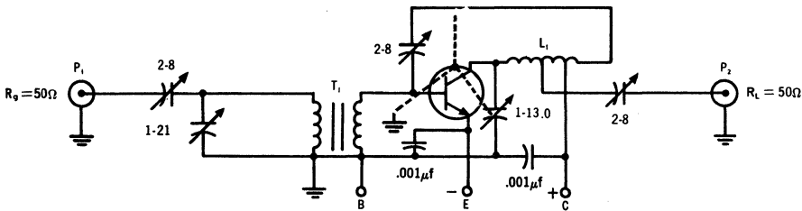
200 MC TEST CIRCUIT: POWER GAIN, NOISE FIGURE, & AGC
