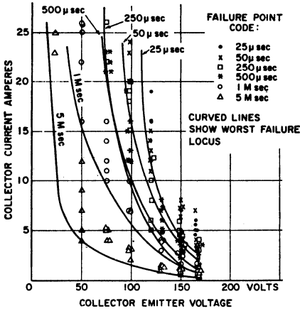
Fig. 3. Graph shows typical failure points for 2N2526 transistor.
