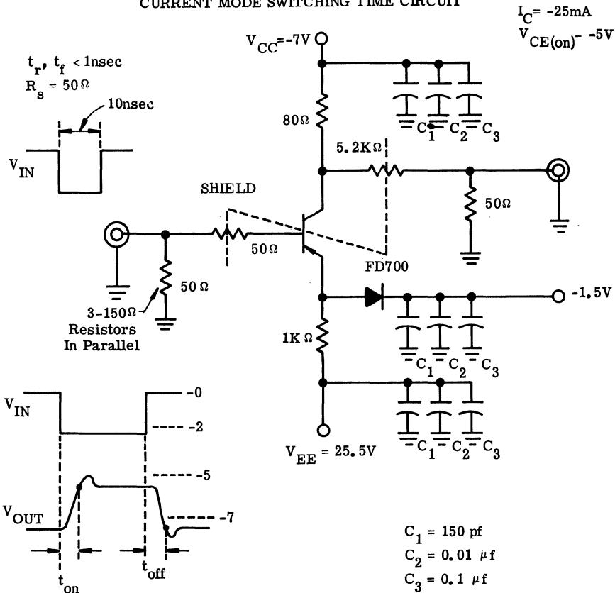
CURRENT MODE SWITCHING TIME CIRCUIT
