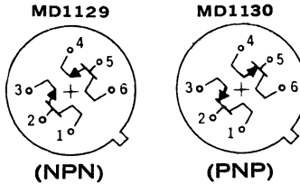
PIN CONNECTIONS BOTTOM VIEW
