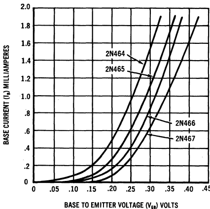
Input Current versus Emitter-Drive Voltage
