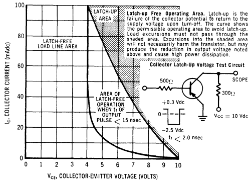
AREA OF PERMISSIBLE LOAD LOC1
