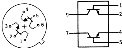
PIN CONNECTIONS BOTTOM VIEW
