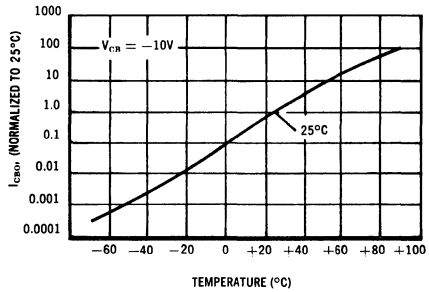
COLLECTOR CUTOFF CURRENT versus TEMPERATURE
