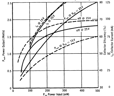
OUTPUT CHARACTERISTICS (250 mc)
