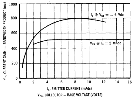
CURRENT-GAIN-BANDWIDTH PRODUCT vs CURRENT AND VOLTAGE
