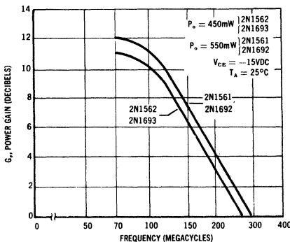
POWER GAIN versus FREQUENCY
