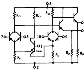
MC309 DUAL "NOR"
