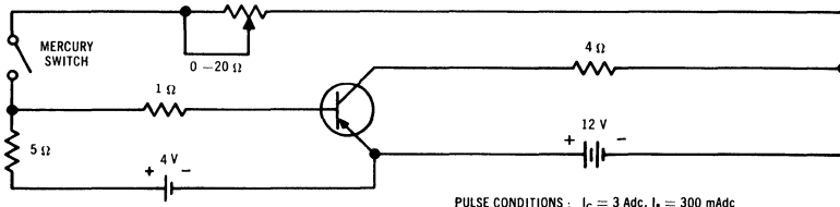
SWITCHING TEST CIRCUIT
