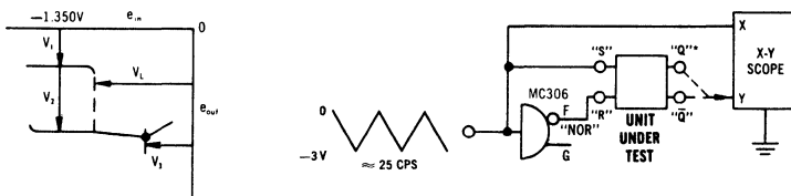
*FOR "Q" TESTS REVERSE "S" & "R" CONNECTIONS
