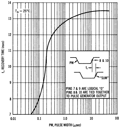
RECOVERY CHARACTERISTICS WITH SIMULTANEOUS "0" ON ALL INPUTS
