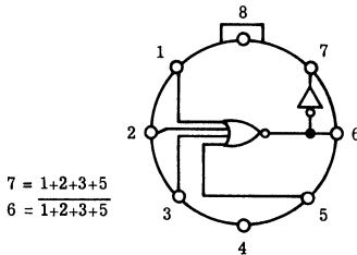
POSITIVE LOGIC
