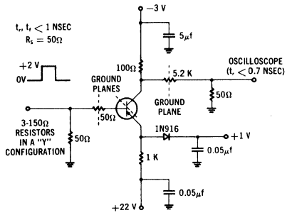
PNP SWITCHING TIME TEST CIRCUIT
