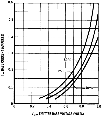
INPUT CHARACTERISTICS
