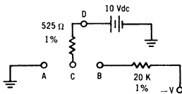
TERMINAL TEST CONNECTIONS DIFFERENTIAL VOLTAGE
