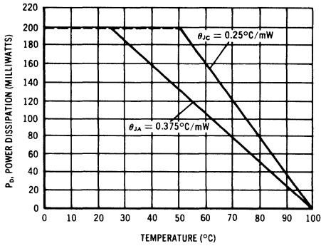
POWER-TEMPERATURE DERATING CURVE
