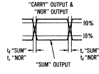
RISE AND FALL TIMES
