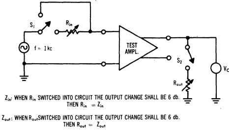
DIFFERENTIAL INPUT IMPEDANCE AND SINGLE ENDED OUTPUT IMPEDANCE
