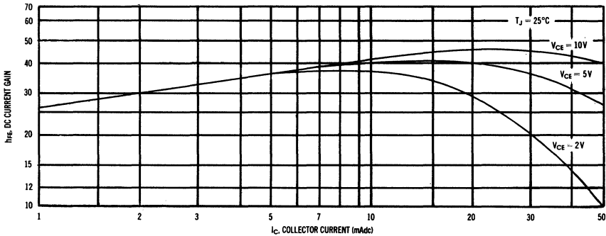
CURRENT GAIN CHARACTERISTICS versus COLLECTOR EMITTER VOLTAGE
