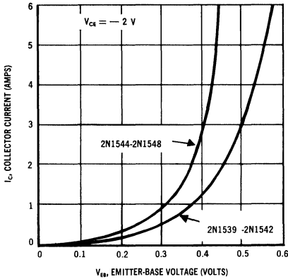
COLLECTOR CURRENT versus EMITTER BASE VOLTAGE
