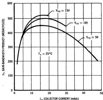
f T versus COLLECTOR CURRENT
