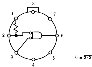
NEGATIVE LOGIC
