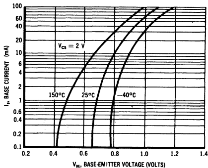
BASE CURRENT - VOLTAGE VARIATIONS
