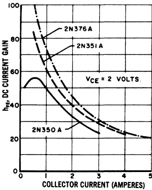
CURRENT GAIN versus COLLECTOR CURRENT (COMMON EMITTER)
