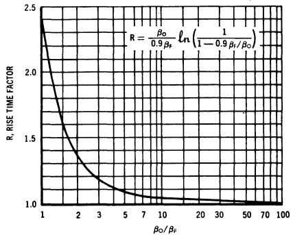
RISE TIME FACTOR
