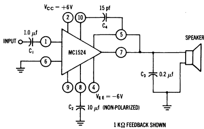
AC COUPLED CIRCUIT
