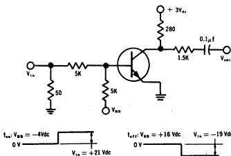
TURN-ON AND TURN-OFF TIME MEASUREMENT CIRCUIT
