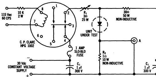
FIGURE 4 — t r TEST CIRCUIT
