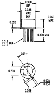
5-LEAD TO-5 PACKAGE CASE 89
