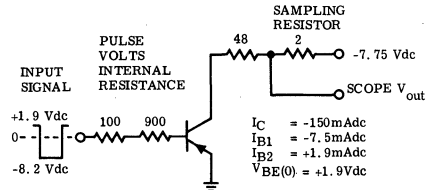
150mA SWITCHING TIME TEST CIRCUIT FIGURE 2
