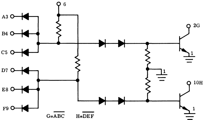
3-3 NAND/NOR GATE
