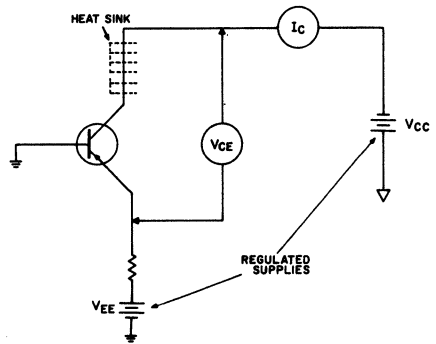
Figure 4 — Electrical circuit.
