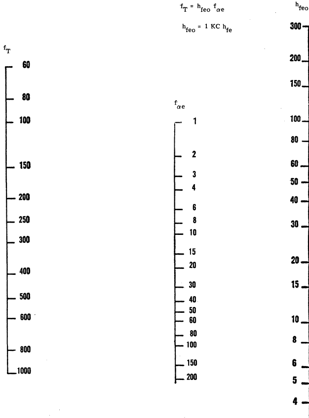
▲ Fig. 5. The quantity f_T is found from this nomogram once f_{\alpha e} and h_{fe0} are known.
