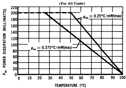
POWER-TEMPERATURE DERATING CURVE
