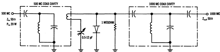
FIGURE 1 — HARMONIC DOUBLER EFFICIENCY TEST CIRCUIT
