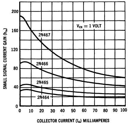
Small Signal Current Gain versus Collector Current (common emitter 1 kc)
