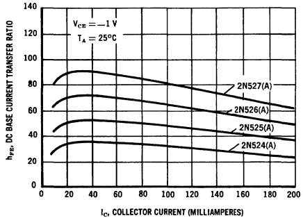
D-C BASE CURRENT GAIN versus COLLECTOR CURRENT
