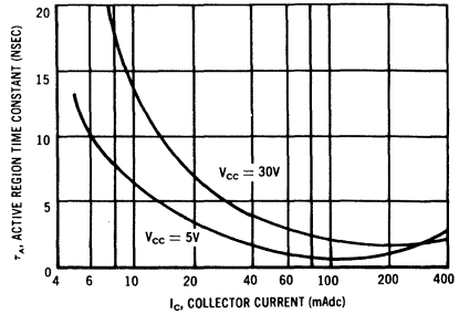
ACTIVE REGION TIME CONSTANT versus COLLECTOR CURRENT
