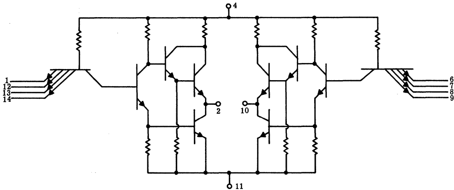
NOR GATE
