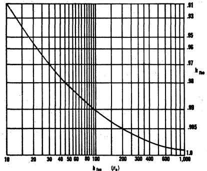
Fig. 3. The relationship between h_{fe0} and h_{fb0} is given by the graph shown.
