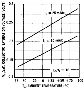
COLLECTOR SATURATION VOLTAGE versus AMBIENT TEMPERATURE
