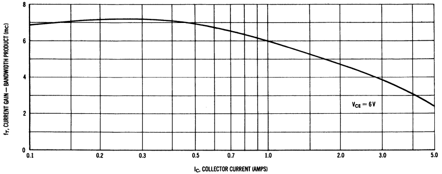
CURRENT GAIN - BANDWIDTH PRODUCT versus COLLECTOR CURRENT
