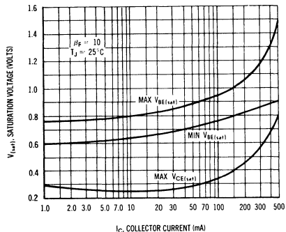
LIMITS OF SATURATION VOLTAGE
