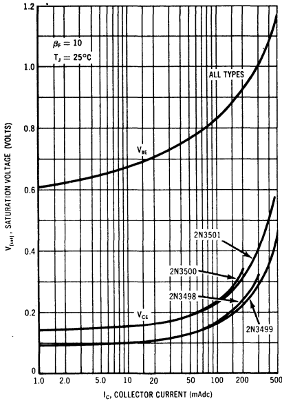
SATURATION VOLTAGES
