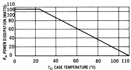
POWER - TEMPERATURE DERATING CURVE
