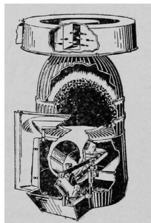
Cut Out View New-Feed UNDERFEED Furnace.
