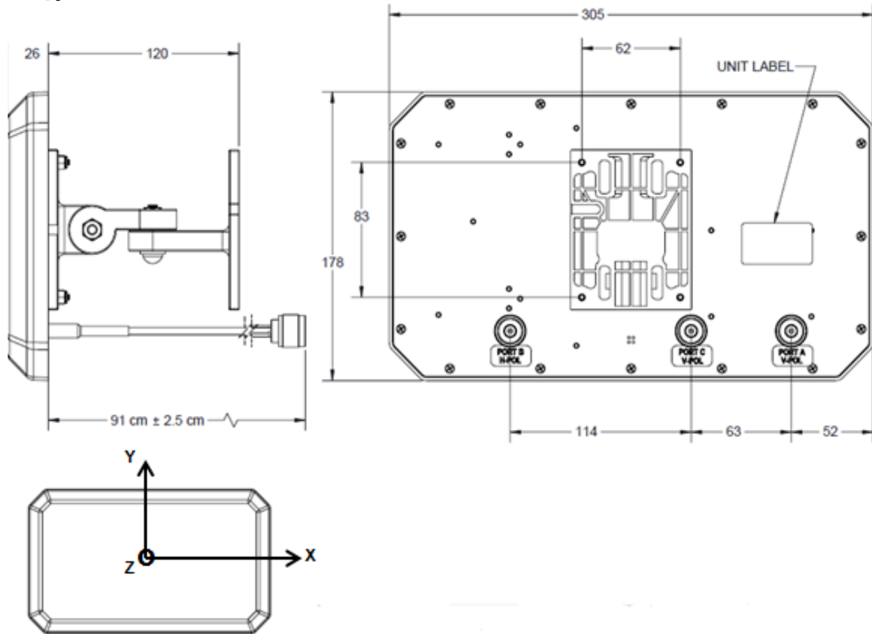
FRONT VIEW 1:4 SCALE
