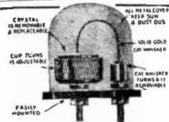
SPECIALY ADAPTED FOR REFLEX WORK
