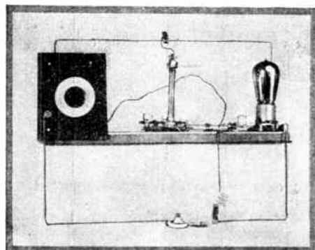
On the left is the transmitter using a 5-watt tube. Above is the top view of the receiving circuit. Copper tubing ¼ inch in diameter was used to form the 2-turn inductances. Note the arrangement of apparatus for shortness of connections. On the right is another transmitter that employs a 50-watt tube. ¼-inch copper tubing is used for the loop, which is also employed as connections for the instruments.
