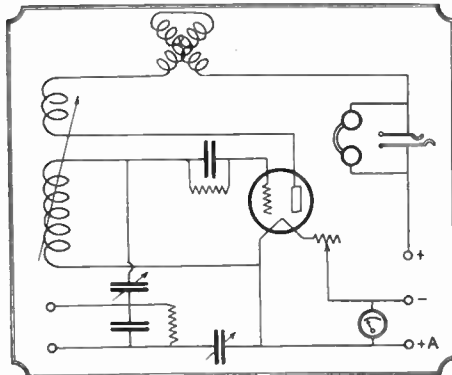
The schematic diagram of the Kiro-vox. With a little juggling it would make a good radio receiver.
