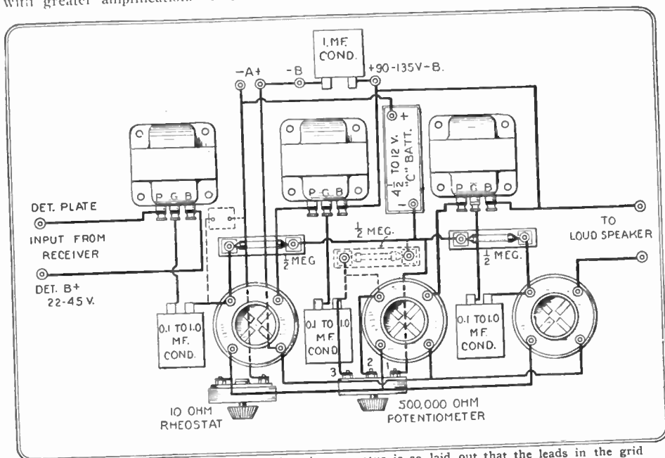
It will be noticed from the diagram that the apparatus is so laid out that the leads in the grid and plate circuits are as short as possible.
