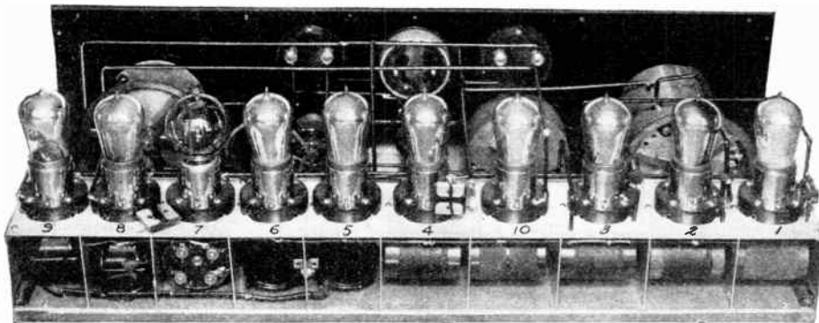
How "the makin's" of the E.I.S. super-heterodyne look when put together. All the sockets are on a metal panel or a strip. General Radio No. 271 I.F. transformers and filter were used. Note vertical shields between each unit.
