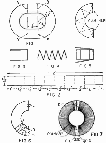
Constructional data for building toroidal coils.
