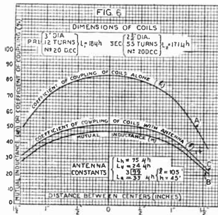
The effect of the antenna on the coefficient of coupling is clearly shown in this diagram.
