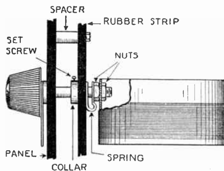
This method of mounting rotor coil keeps it exactly in the desired plane without deviation.
