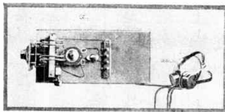
On the left is the transmitter using a 5-watt tube. Above is the top view of the receiving circuit. Copper tubing ¼ inch in diameter was used to form the 2-turn inductances. Note the arrangement of apparatus for shortness of connections. On the right is another transmitter that employs a 50-watt tube. ¼-inch copper tubing is used for the loop, which is also employed as connections for the instruments.
