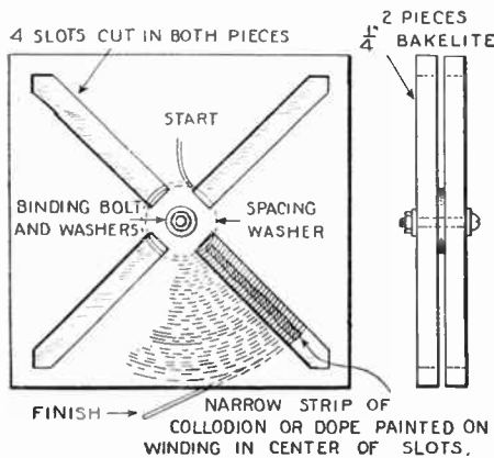
Two pieces of bakelite cut as shown make an excellent winding form for pancake coils.
