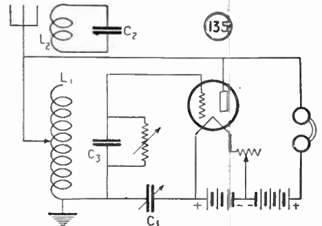
The variation of the ultra-audio circuit shown above will prove to be popular with one's neighbors, as it will not radiate.
