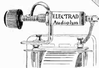
"ELECTRAD" AUDIOHM—A necessary tone and quality controlling device. Placed across secondary of first audio transformer it eliminates distortion and transformer noises. Requires no drilling, soldering or tools to attach. Fits any transformer. $1.50 each.
