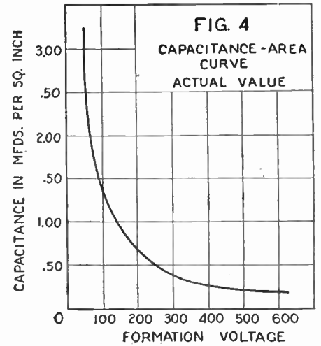
Curve showing actual capacity per unit area for different formation voltages.
