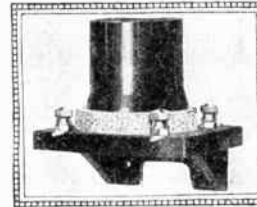
FROST-RADIO BAKELITE CUSHION SOCKETS Single, $1.25 3-gang, $3.75
