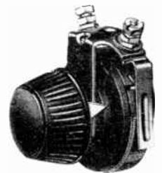
The Perfected C-H Rheostat Designed to radio engineers' specifications. Revolving drum type with one hole mounting. All spring tensions adjusted at factory and undisturbed by mounting. Instrument cannot turn on panel. Very small size—less than 1/4 inch back of panel and narrower than standard socket. Operation smooth and quiet. 6 ohms, 15 ohms, and 30 ohms—perfect control for all tubes and their combinations.
