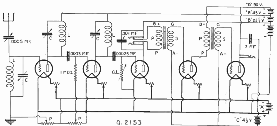
Tuned Impedance. The standard schematic circuit for a receiver using "tuned impedance" coupling. Each tuned unit, when adjusted for a given signal, "rejects" that signal, causing the signal to charge the blocking condenser and, in turn, operate the grid of the amplifier tube. Undesired signals are "accepted" and do not operate the amplifier tubes. The circuit shown is very selective.
