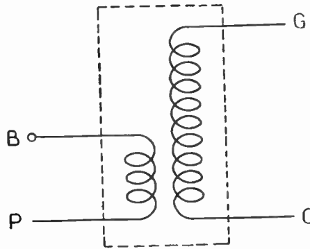
Fig. 5. The coil terminals must be connected as shown for proper operation of the set.
