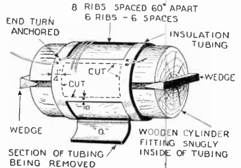
Coils constructed by this method will be perfectly cylindrical and wound on a minimum of insulation.
