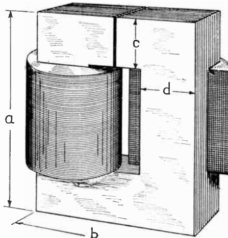
FIG. 7 Dimensions are given in the accompanying table for two different sizes of choke coils; one for receiving and the other for transmitting purposes.
