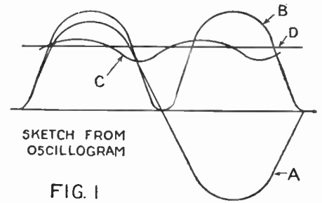
FIG. 1 A, is a pure A.C. wave; B, a rectified wave; C, a filtered rectified wave and D, a wave having a condenser and coil in the circuit.
