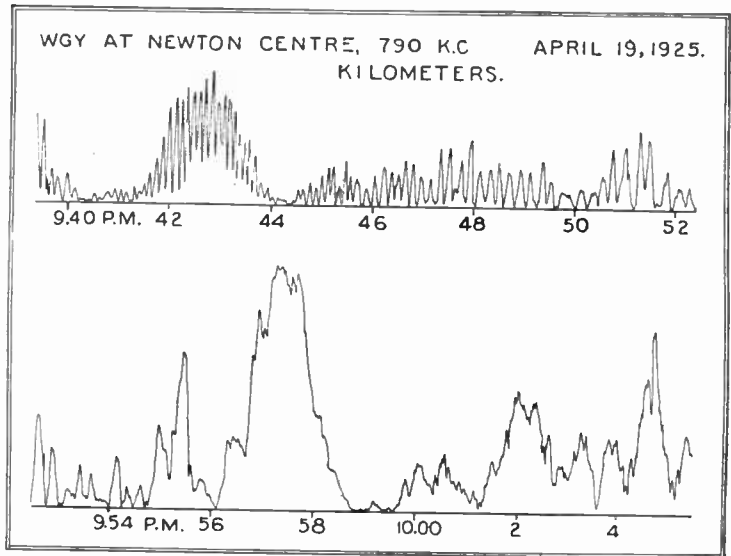
Another of Mr. Pickard's charts, from which he makes the present study of wave characteristics and propagation.
