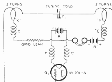
The receiver may be a separate set of instruments, or those of the transmitter can be used for reception with little extra wiring.
