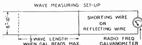
The "Lecher" method of measuring the length of radio waves is used to find accurately the frequency of the transmitter or receiver.
