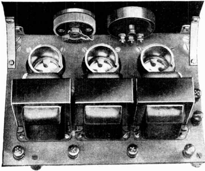
The top view of the amplifier unit shows the rheostat, potentiometer, the three vacuum tube sockets and the three impedances. The condensers and resistances are under the shelf, as shown in the photograph on the opposite page.
