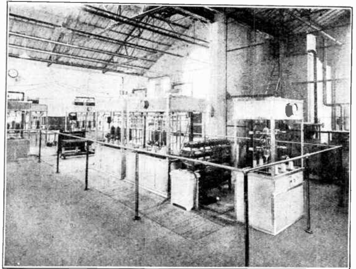
The main modulator tubes are shown on the left and the auxiliary modulator on the right. In the center is the dry battery for supplying the necessary grid bias.
