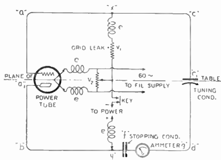
The transmitting circuit uses the connections between the parts as a loop antenna.
