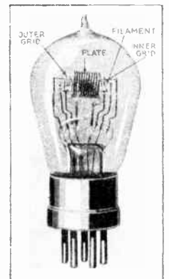
A double-grid vacuum tube that is manufactured in England. It has the same internal construction as that on the opposite page. A special socket is required for these tubes, as they have five connection prongs.
