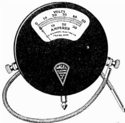
If you own a "Super-Het" or are operating your set with dry cells, you need this Nagel Voltmeter, a combination instrument for testing both A and B batteries.
