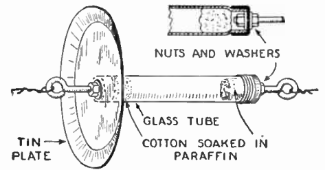
A pie-plate and a glass toothbrush holder are the essential materials for this antenna insulator.
