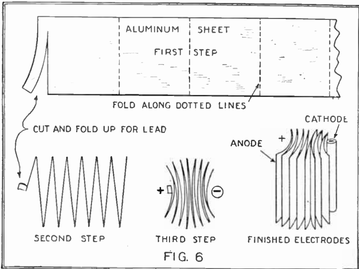
The method of folding the sheet aluminum for forming the element of the electrolytic condenser.
