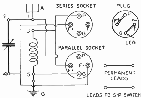
A series-parallel switch that can be constructed from two sockettes and a burnt-out tube.
