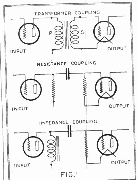
FIG. 1 Three Types of Audio Frequency Amplifiers
