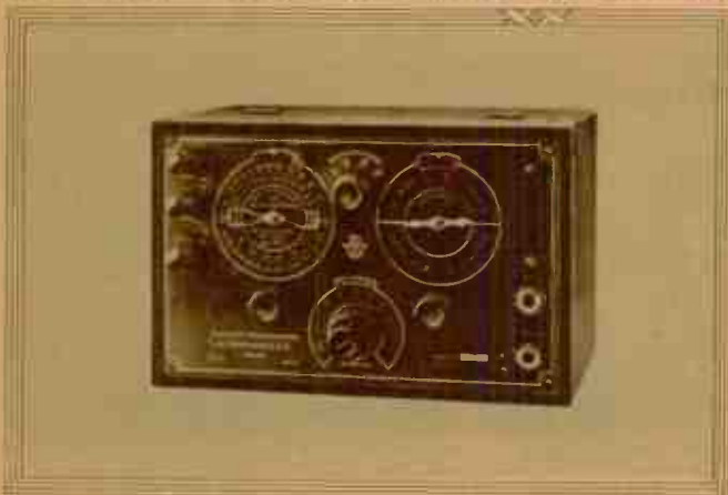
An idea which has never been exploited in the United States is incorporated in the set at the left. It is calibrated in wave-lengths at the factory.
