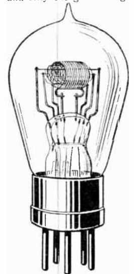
Fig. 4. The two inside spirals are the inner and the outer grid elements; the large spiral of heavier wire is the plate and the filament is the single straight wire stretched between the two outer supporting posts.
