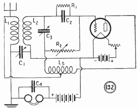
The parts for the Kaufman circuit, with the exception of the "active 20" coil, can be easily obtained and the circuit is an interesting one from an experimental viewpoint.
