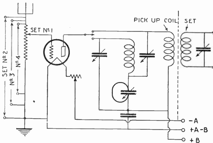
Dr. A. Hoyt Taylor's new multiple set device hook-up—through its use any number of receivers may operate from the same antenna.
