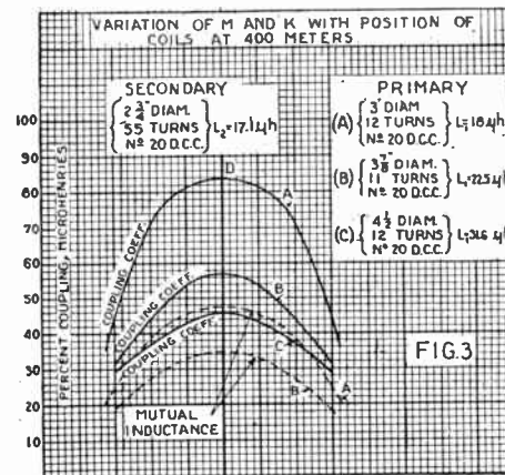
These curves show actual values obtained by measurements made on ordinary antenna coupling coils.
