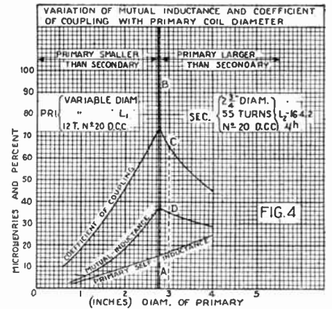
The coupling has its maximum value when the two coils have the same diameter.
