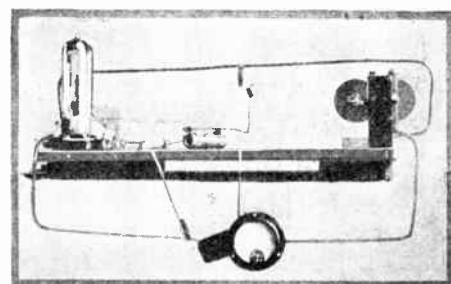
On the left is the transmitter using a 5-watt tube. Above is the top view of the receiving circuit. Copper tubing ¼ inch in diameter was used to form the 2-turn inductances. Note the arrangement of apparatus for shortness of connections. On the right is another transmitter that employs a 50-watt tube. ¼-inch copper tubing is used for the loop, which is also employed as connections for the instruments.
