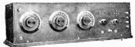
5-TUBE COCKADAY
