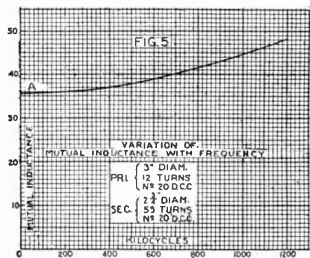
The point A, at zero frequency, agrees with the calculated point D of Fig. 4. Note that M increases with the frequency.
