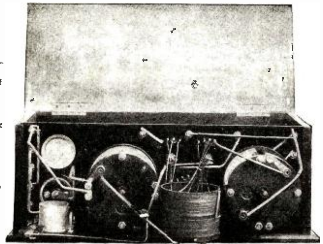
Two Views of the Reinartz Receiver Described in This Article. Instead of the Usual Spider-Web Coil, a Single Layer Inductance is Employed.
