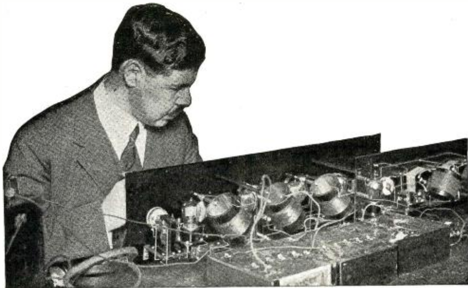
Professor L. A. Hazeltine Tuning a Neutrodyne Receiver. On the Right May Be Seen Another Neutrodyne Set of the Reflex Type Using Four Tubes Which Provides Two Stages of Radio Frequency, Detector and Two Stages of Audio Frequency Amplification.
