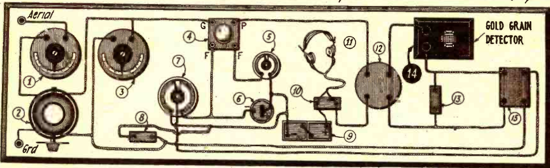
1= var. cond. .001 mfd. 43 plates. 2= variocoupler. 3= var. cond. .0005 mfd. 23 plates. 4= vacuum tube (amp) 14= NATIONAL AIRPHONE GOLD GRAIN DETECTOR 5= rheostat. 6 A' batt. (DRY CELL FOR WD-11) 7= 200-400 Ohm potentiometer. 8= fixed mica cond. .001 mfd. 9= batt. 45v. 10= fixed mica cond. .001 mfd. 11= phones. 12= mu rad. radio freq. transf. 13= .001 mfd. F.C. 15= federal audio freq. transf.
