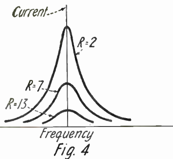
A Resonance Curve For Fig. 1 With Three Different Values of R. When the Resistance Is Low the Curve Is Very Sharp, As Shown in the Case Where R Equals 2.
