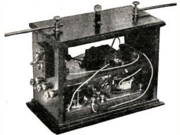
Left: Showing the Connections of the Instruments Mounted on the Baseboard. Above: The Relay. Right: Photo of the Complete Receiver.
