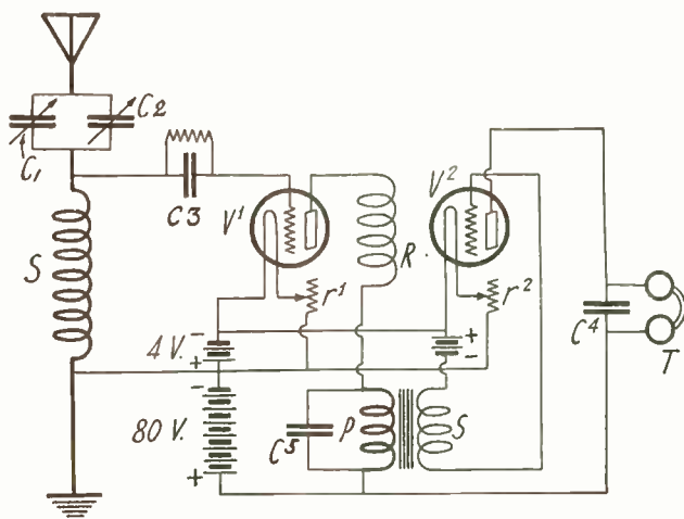
The Hook-up Employed by Mr. Thouvais During the Tests. It is of the Single Circuit Type and Has an Exceedingly High Factor of Selectivity in Comparison with Other Single Circuit Receivers. Having But Two Controls, it is Ideal for Amateur Work. The Instruments marked are: V 1 Detector Tube, V 2 Amplifier Tube, P and S Audio Frequency Transformer, R 1 and R 2 Filament Rheostats, C 1 .001 M.F. Variable Condenser, C 2 Vernier Variable Condenser, C 3 .00025 M.F. Fixed Grid Condenser, C 4 .002 M.F. Fixed Condenser, S Aerial Tuning Inductance (30 Turns for 200 Meters, 50 Turns for 360 Meters) R 30 to 50 Turn Tickler Coil Coupled to Aerial Tuning Inductance.
