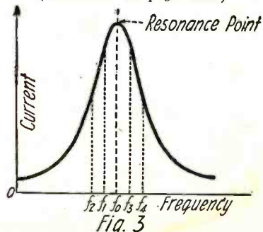
A Curve Illustrating the Current That Would Flow In the Circuit of Fig. 1 At Different Frequencies.
