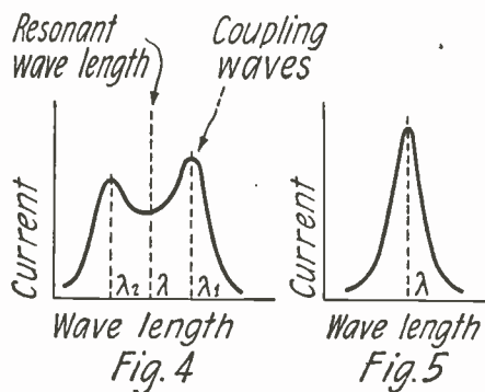
Fig. 4. Effect of Tight Coupling. Fig. 5. Effect of Loose Coupling.
