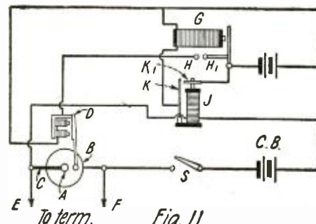
This Designates the Connections Between the Antenna, Coherer, De-cohering Device, Relay and Selector.
