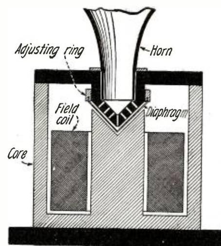
Sectional View of the New Type of Loudspeaker. Note the Small Gap in the Magnetic Circuit with the Cone-Shaped Diaphragm Upon Which is Stuck the Fine Wire Composing the Armature.
