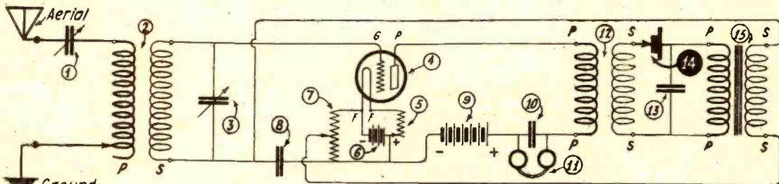
1= var. cond. .001 mfd. 43 plates. 2= variocoupler. 3= var. cond. .0005 mfd. 23 plates. 4= vacuum tube (amp) 14= NATIONAL AIRPHONE GOLD GRAIN DETECTOR 5= rheostat. 6 A' batt. (DRY CELL FOR WD-11) 7= 200-400 Ohm potentiometer. 8= fixed mica cond. .001 mfd. 9= batt. 45v. 10= fixed mica cond. .001 mfd. 11= phones. 12= mu rad. radio freq. transf. 13= .001 mfd. F.C. 15= federal audio freq. transf.
