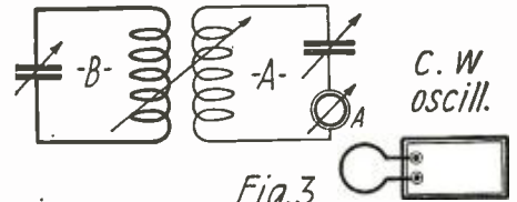
Method of Measuring the Coupling Coefficient of Two Circuits.
