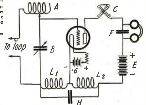
Two Views of Mr. Jones' Super-Regenerator. This Set Employs a Plate Variometer and a Tapped Inductance in Series with a Loop Aerial. The Circuit is Shown on the Right.
