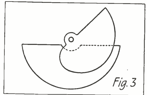
Fig. 3 Specially Shaped Plates for Wavemeter Condenser.
