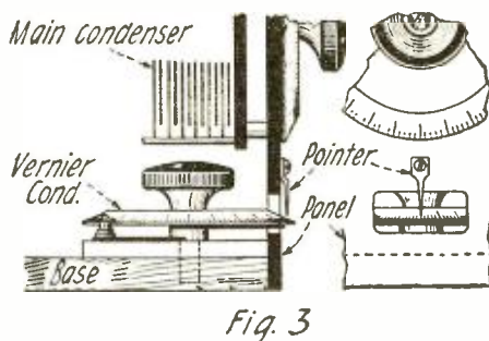
Method of Mounting the Novel Vernier Condenser. It is Adjusted from the Front of the Panel by the Thumb or Fore Finger.
