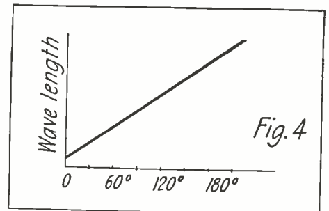
Fig. 4 Wave-Length Curve for Special Shaped Wave-meter Condenser.
