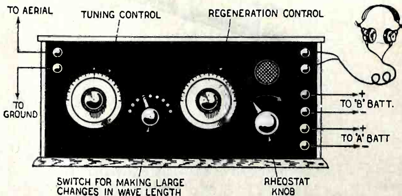
Fig. 8. Illustrating a Two-Control Regenerative Receiving Set with Connections for Aerial, Ground and Batteries
