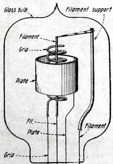
Schematic View of a Vacuum Tube Showing the Arrangement of Filament, Grid and Plate.
