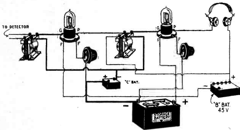
Fig. 6. Showing How the "C" Battery is Connected in a Two-Stage Amplifier Circuit
