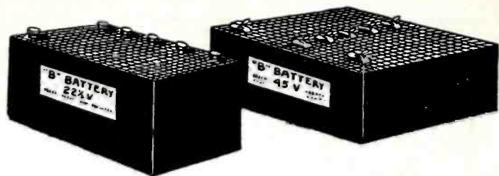
A 22½-Volt and a 45-Volt Battery with "Taps" or Terminals for Obtaining Various Voltages
