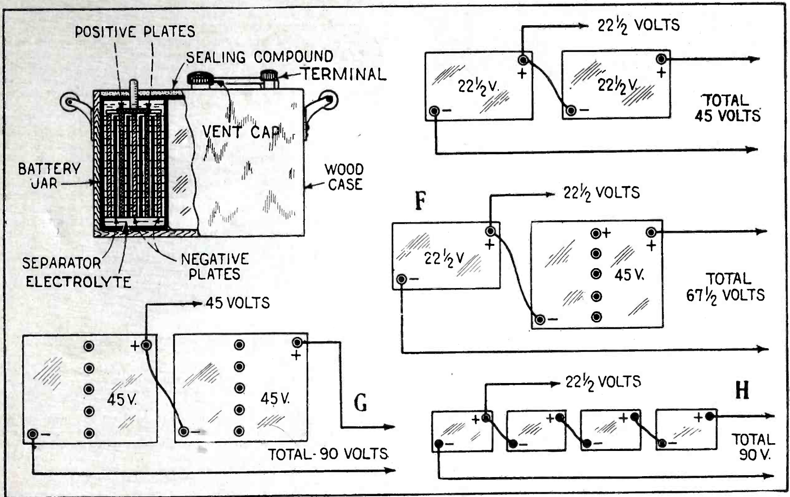
Fig. 4. A Cross-sectional View of a Storage Battery Showing How the Plates Are Arranged in One of the Cells. Also Methods of Connecting "B" Batteries Together in Order to Obtain Various Voltages
