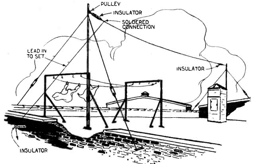
Fig. 7. A Typical Aerial Erected on Top of a House
