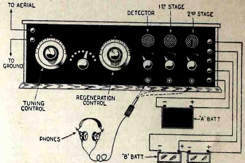
The Same Set as Shown in Fig. 8, but with the Addition of a Two-stage Audio Amplifier. The Proper Connections for the Batteries, Aerial and Ground Are Indicated
