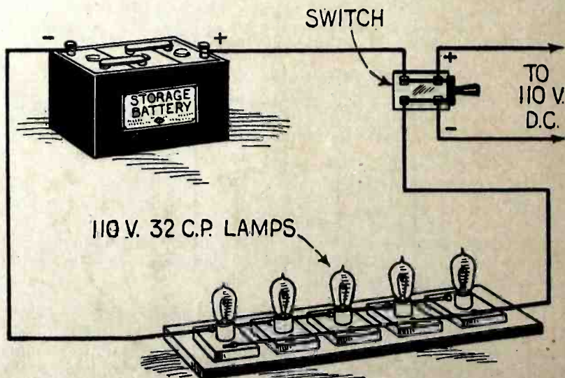
Recharging a Storage Battery with a Lamp-bank from Direct Current
