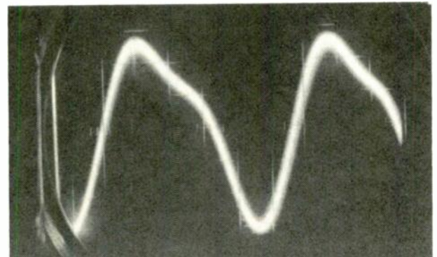
FIG.3—SQUAREWAVE AFTER RECORDING and being played back on a cassette recorder.
