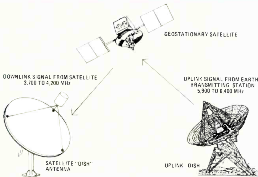
FIG. 3—C-BAND SIGNALS ARE UPLINKED at frequencies between 5.9 and 6.4 GHz, and downlinked at frequencies between 3.7 and 4.2 GHz.
