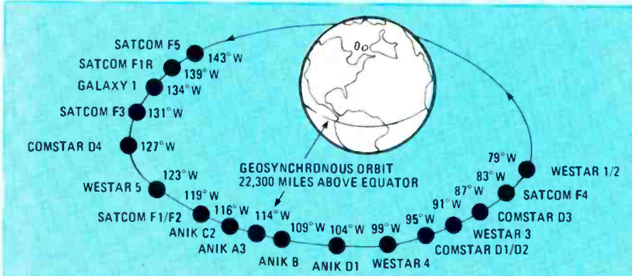
FIG. 2—ALL NORTH-AMERICAN SATELLITES orbit in the equatorial plane. They are located in that phase between 79° and 143° west longitude.
