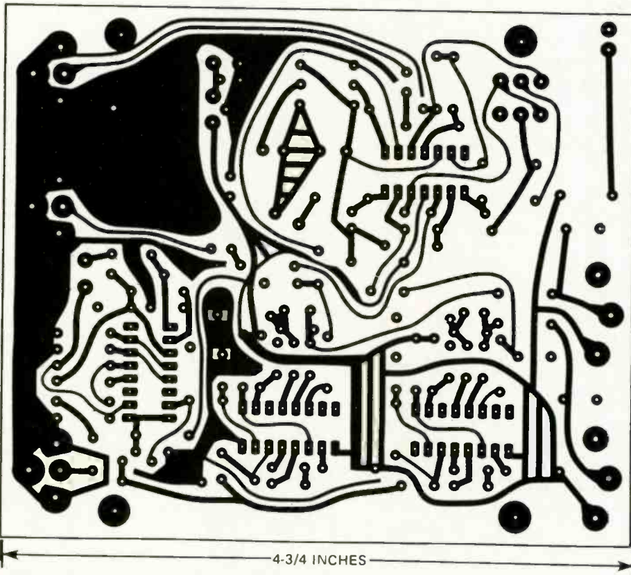
FIG. 6—SOLDER SIDE of the demodulator's circuit board.
