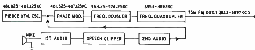
Fig. 1—Block diagram of the exciter. A reactance tube shifts the phase of the oscillator.
