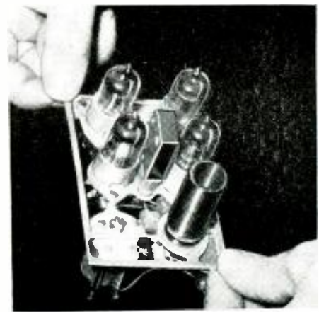
The AM transmitter. Metal sections are removed from the chassis to reduce weight.
