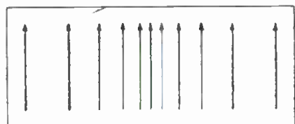
Fig. 5—Cross-section of guide, TE 01 mode.
