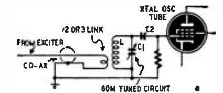
Fig. 3-a—This circuit can cause parasitics.
