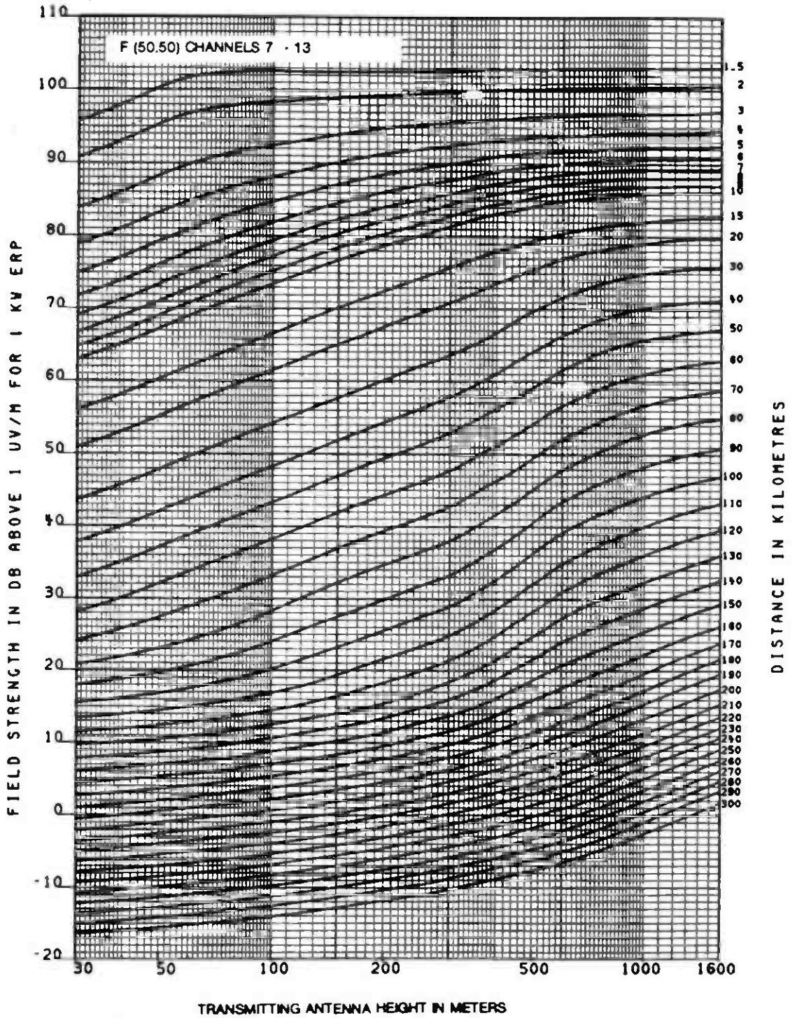
FCC 73.699 Figure 10
