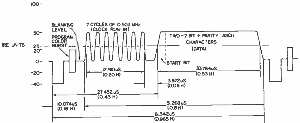
FIGURE 17 LINE 21 FIELD DATA SIGNAL FORMAT
