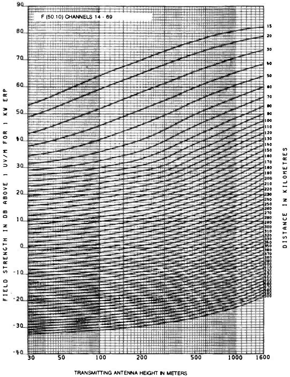
FCC 73.899 Figure 10c
