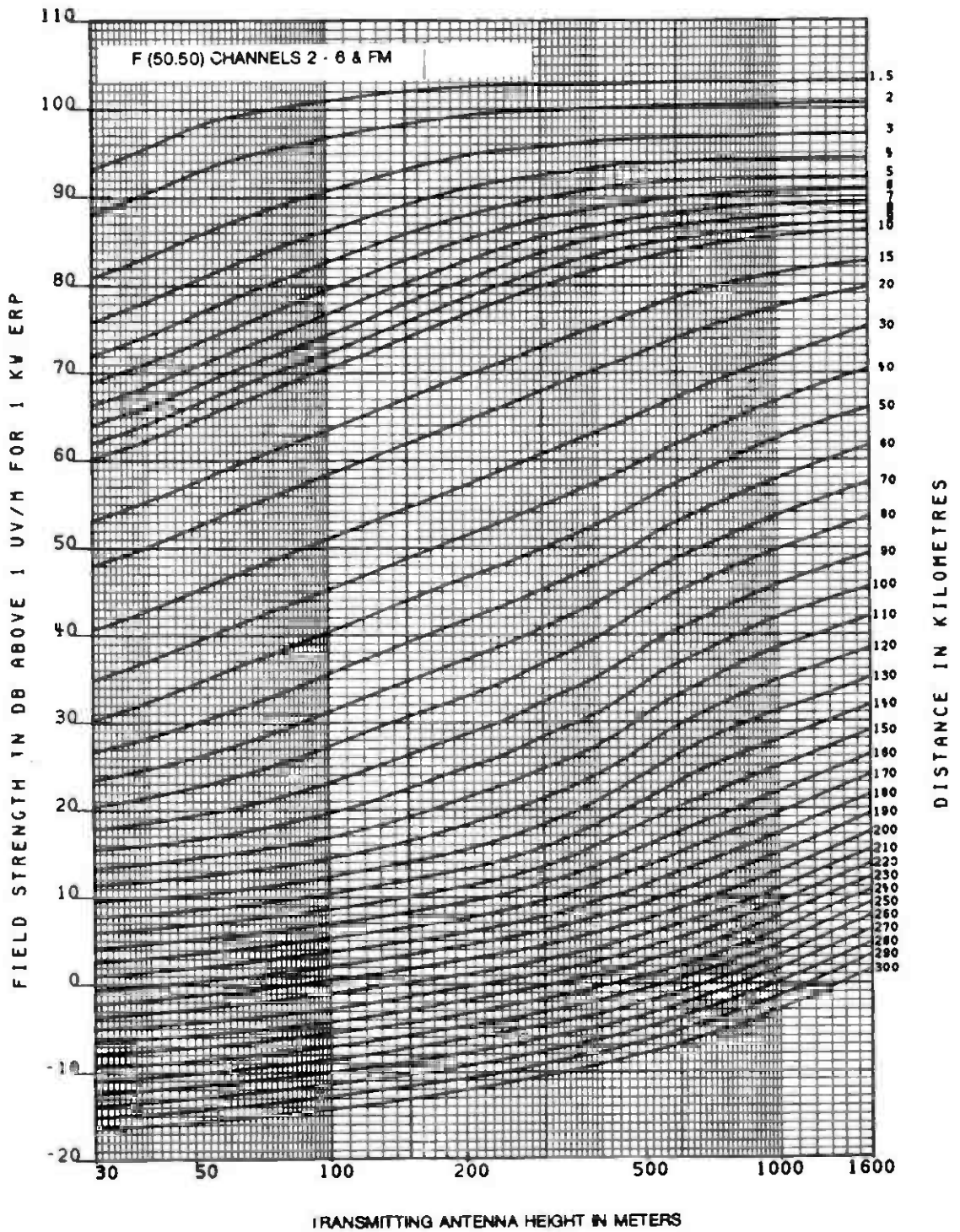
FCC 73.699 Figure 9
