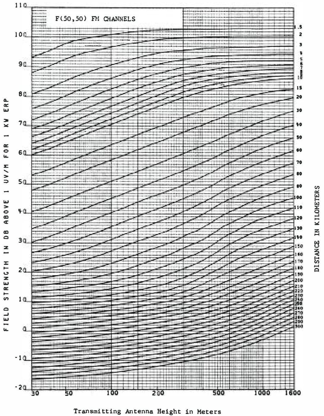
FCC §73.333 FIGURE 1
