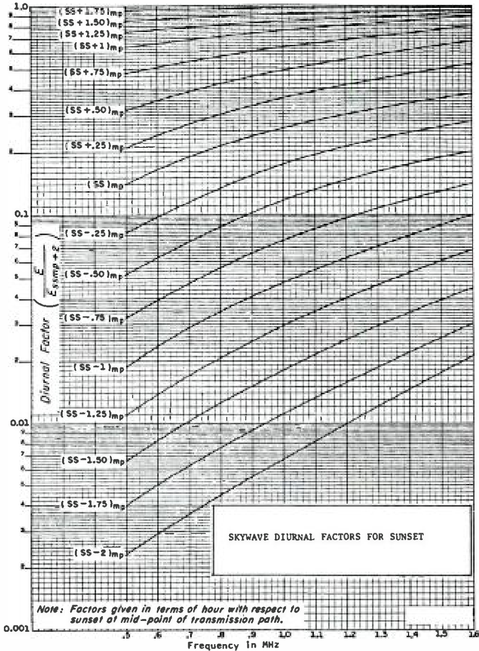
FCC §73.190 Figure 13
