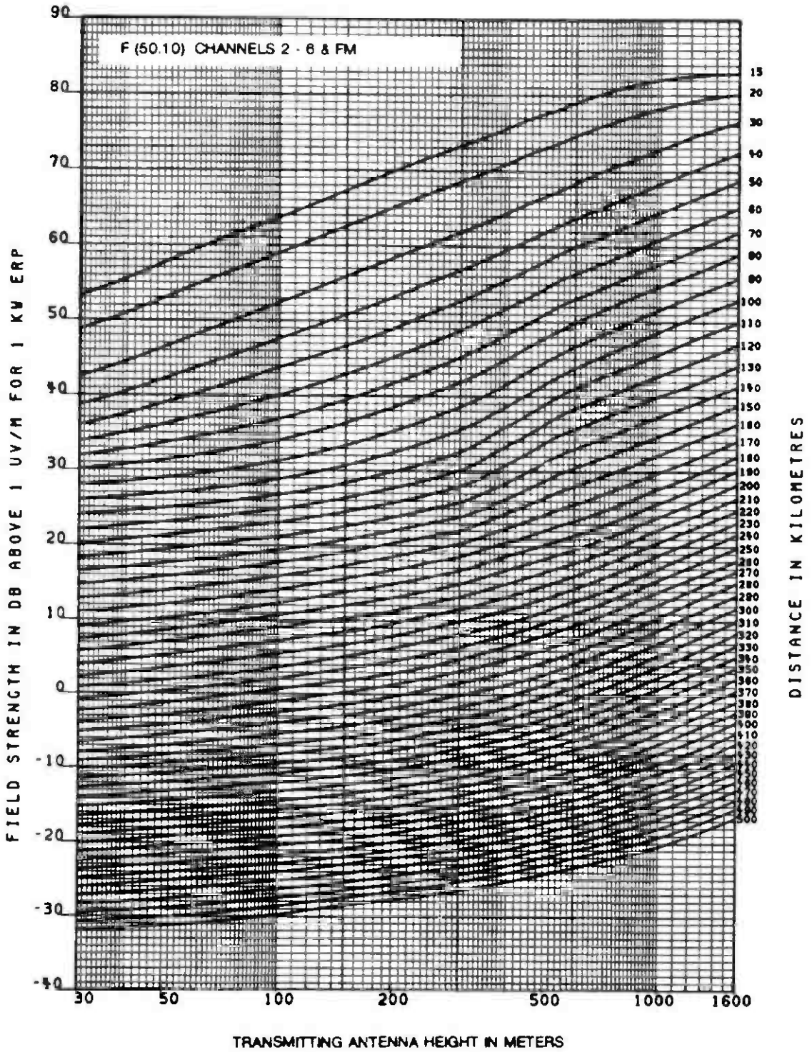
FCC 73.699 Figure 9a
