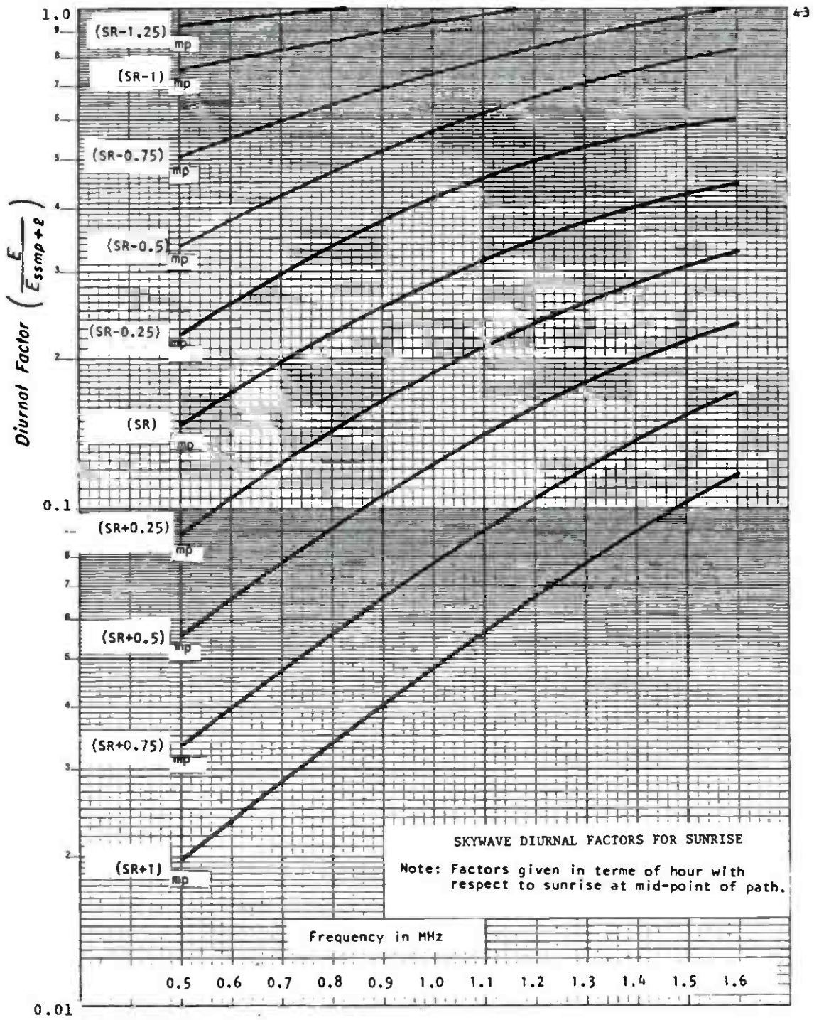
FCC §73.190 Figure 12
