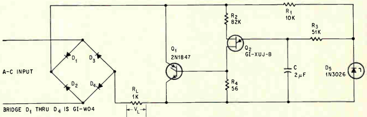
Firing angle of the silicon controlled rectifier varies with amplitude of the input a-c voltage; this variation maintains constant average voltage across load R_L . Load voltage can be adjusted by changing the value of R_1 .
