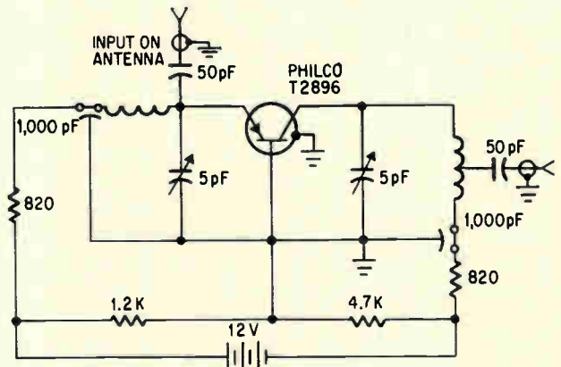
Amplifier in experimental 420-Mc slot antenna has 10 db gain and noise figure of 7.8 db; bandwidth is 100 Mc.
