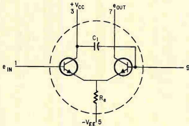
Simple differential r-f amplifier. Advantages of this single-ended circuit over a single-transistor tuned stage include higher power gain, negligible parasitic effects, symmetrical transfer characteristics, lower admittance, greater stability, easier alignment and fewer components. One circuit of this type provides a 26-decibel power gain and a 4-decibel noise figure at 100 megacycles. Automatic gain control is easily achieved by varying V_{EE} which in turn determines the current level.
