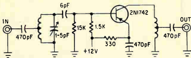
Vhf transistor, which forms the active portion of the dipole antennafier, in a test amplifier.
