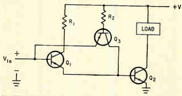
Modified Darlington switch has extra transistor.
