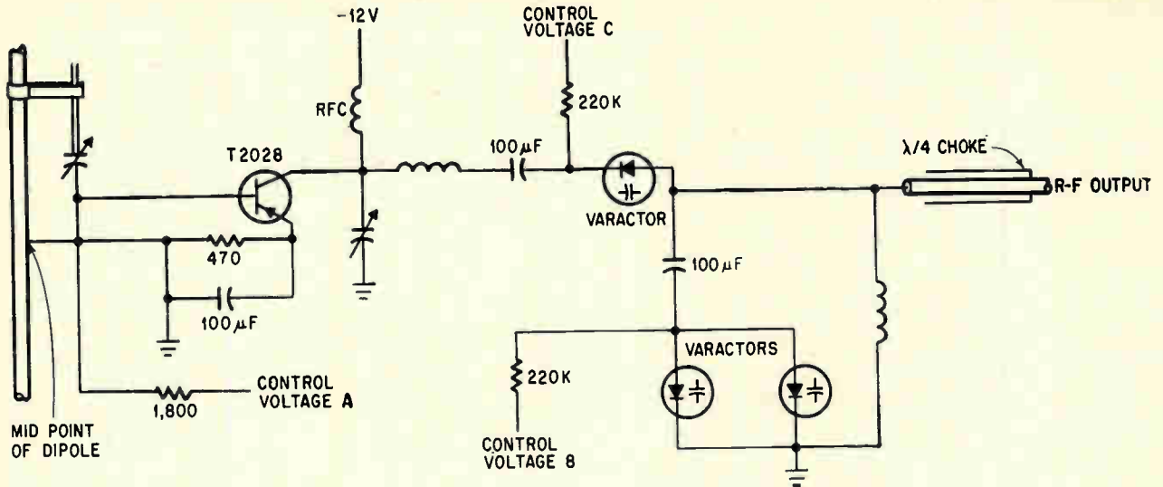
Dipole antenna with phase shifter is one element of steerable-beam array.
