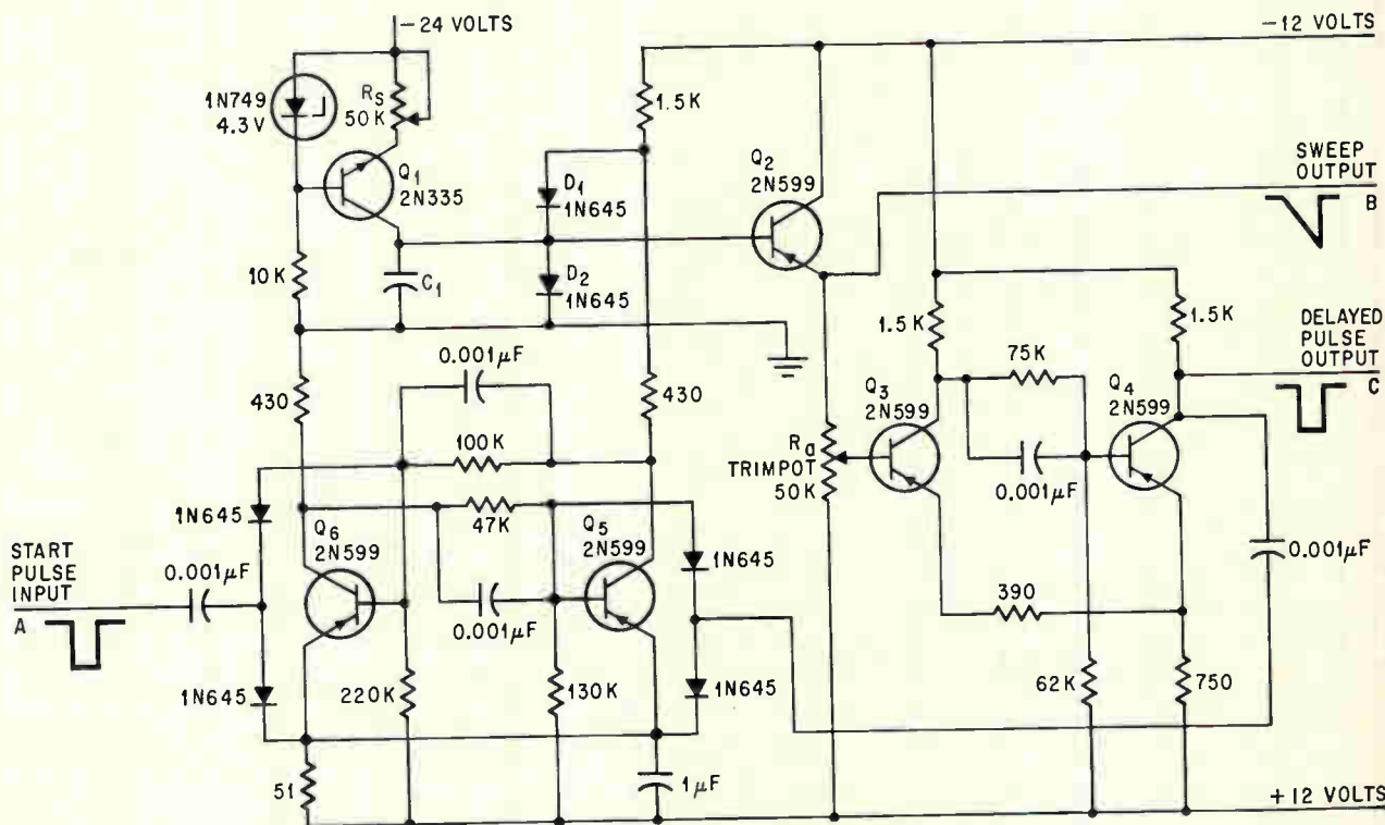
Slow speed sweep generator can be used to keep a camera shutter open to photograph radiation patterns on an oscilloscope. Speed of sweep is determined by R_a and C_1 .
