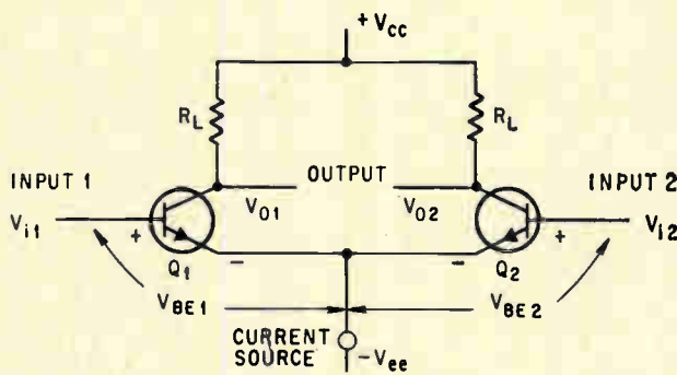
Typical differential amplifier circuit. Input signals are V_{i1} and V_{i2} ; differential output voltage is (V_{o1} - V_{o2}) .
