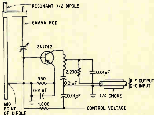
Transistorized dipole antennafiers. Fixed gain is shown at left; controllable gain by external voltage, at right.
