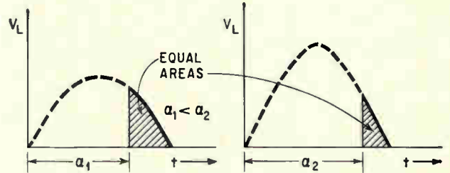
Voltage across load is represented by shaded areas. Equal shaded areas mean that average load voltage is constant.
