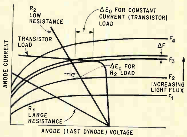
Multiplier phototube characteristics. Sensitivity is greater with a transistor load than with a resistor load.
