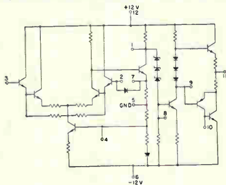
CASE INTERNALLY CONNECTED TO -12V
