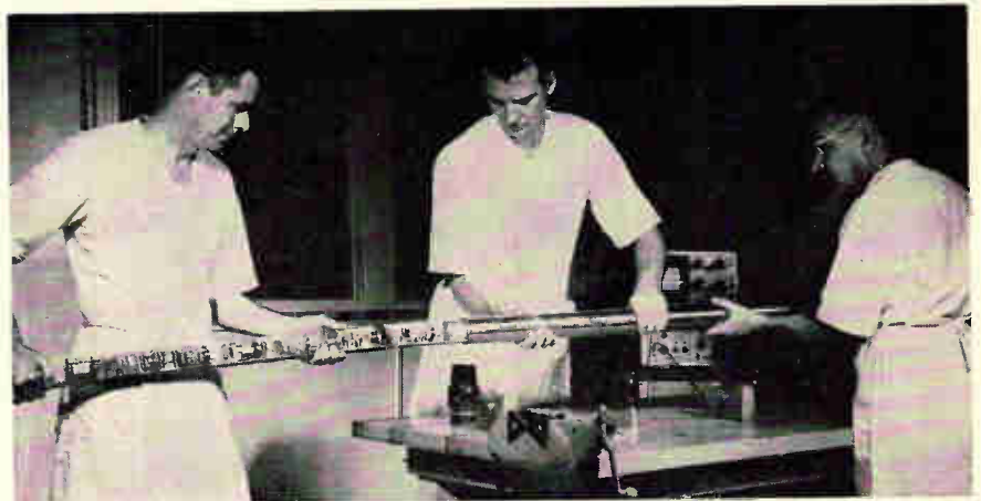
Logging cable for Mohole is jammed with instruments for measuring the properties of crustal and mantle rocks in place.
