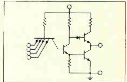
Single 4 input NAND/NOR gate
