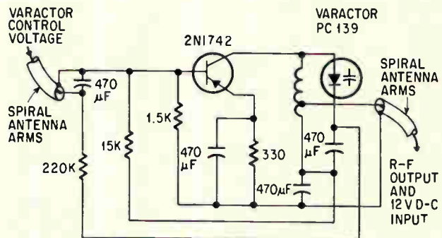
Varactor-tuned transistor amplifier is built into the tip of a conical spiral antenna. Antenna arms are formed by the external sheath of a coaxial cable.
