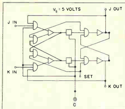
Block diagram of new commercial HLTTTL master-slave flip-flop.
