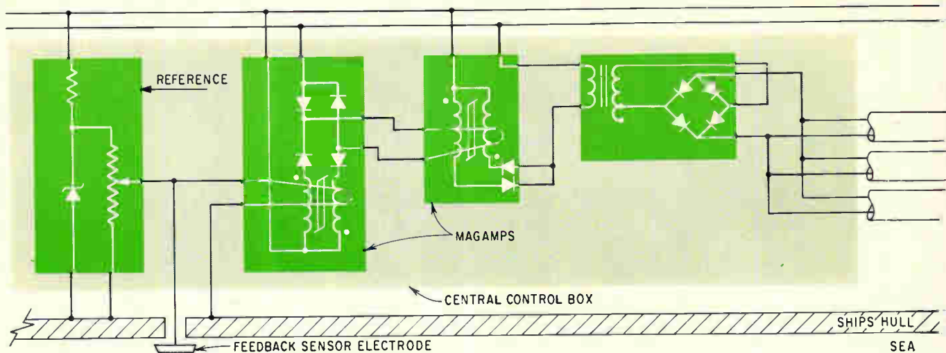
Anticorrosion system laid out partly as a pictorial representation of how the equipment would be installed on a ship and partly as the classic feedback control system diagram. The steel hull of the ship is the system signal and power ground. The reference voltage at the left commands the amount of voltage difference to be impressed on the hull. The
