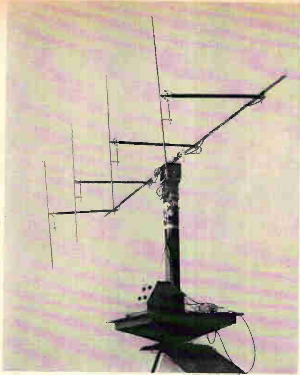
Steerable-beam array made up of four antenna elements spaced a half-wavelength apart. Beam position could be controlled by a series of four ganged potentiometers.
