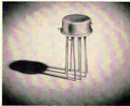
Commercial HLTTTL circuits are packaged in this hermetically-welded TO-5 can with 1/2" leads.
