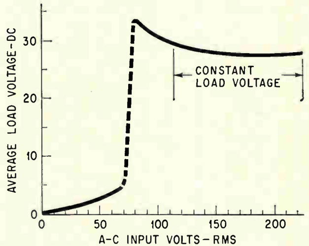
Regulation curve shows that the average load voltage is constant at about 30 volts, as the input a-c voltage varies from 100 to 200 volts rms.
