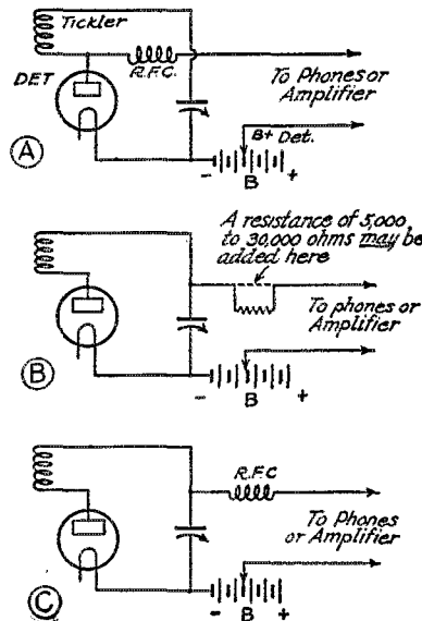
FIG. 4. VARIATIONS OF THE WEAGANT REGENERATION CONTROL
