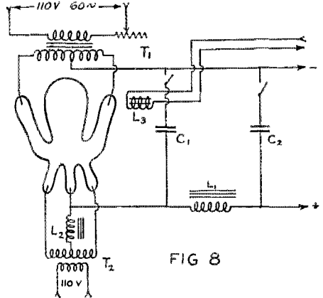
CIRCUIT OF MERCURY-ARC RECTIFIER AND FILTER
