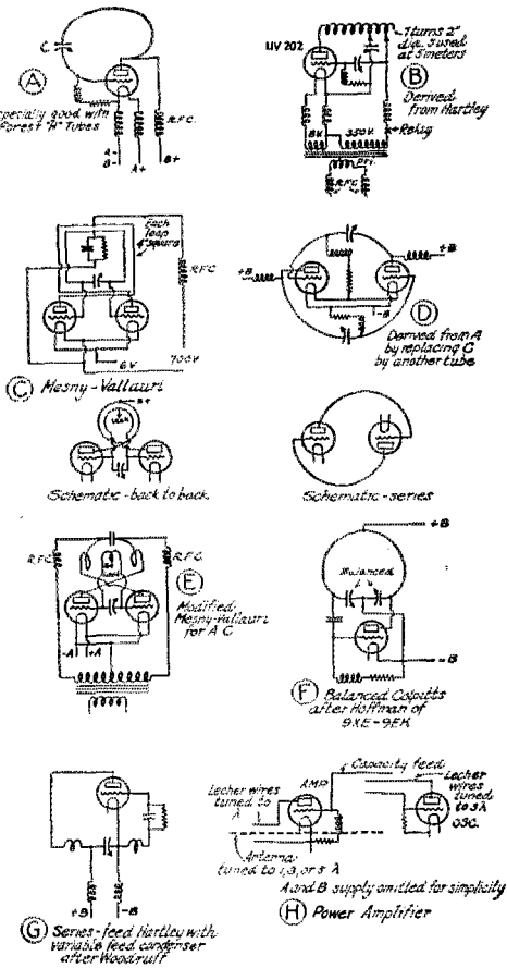
FIGURE 1 SENDING CIRCUITS
