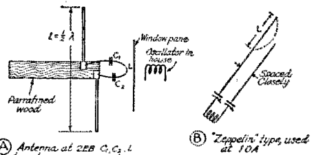
(A) Antenna at 2EB C 1 , C 2 , L tune to same wave as antenna, therefore do not load it.
