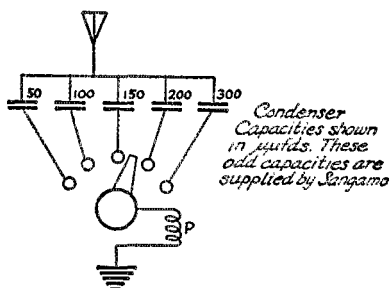
FIG. 9. ANOTHER SCHEME FOR SHIFTING THE ANTENNA TUNING RANGE TO AVOID DEAD SPOTS AND TO GIVE BEST RECEPTION IN EACH HAND
