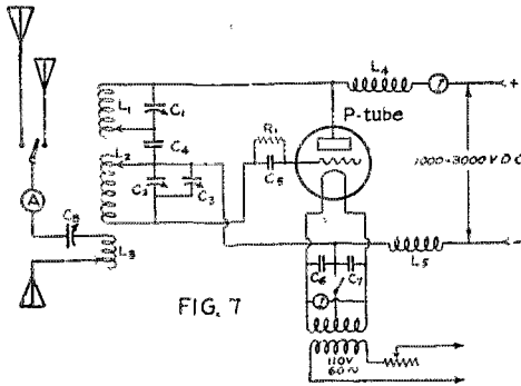
CIRCUIT OF STANDARD FREQUENCY TRANSMITTER AT 1XM
