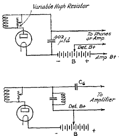
FIG. 5. RESISTANCE METHOD OF CONTROL-LING REGENERATION A With usual audio amplifier. B When using tuned audio trap.
