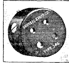
THE GENERAL RADIO ADAPTOR THAT FITS THE SMALL UX BASE IN A STANDARD NAVY SOCKET
