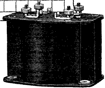
No. 3—A Transformer Ratio 4 to 1 Primary reactance, 125,600 ohms at 1000 cycles. Low core losses, thin laminations. Compact dimensions for sub panel or base board mounting. 2 3/4" long, 1-15/16" wide, 2-3/16" high. Shell type shielding.
