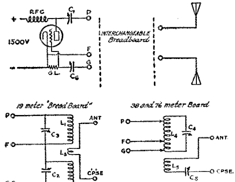
CIRCUIT AT 9CXX
