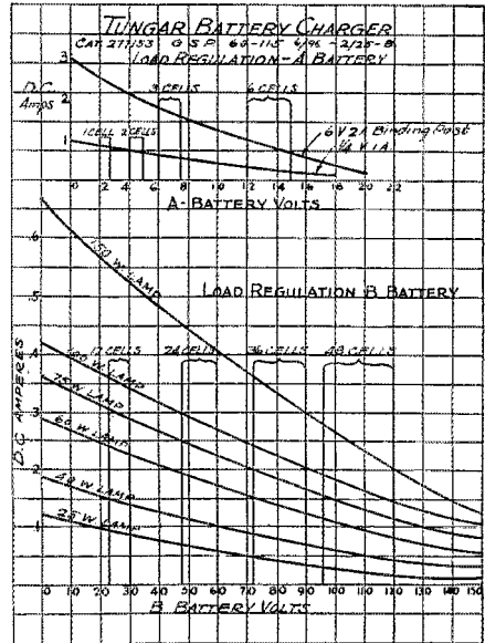
FIG. 2. A AND B BATTERY LOAD REGULATIONS
