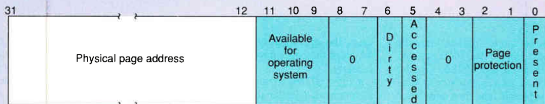
Figure 4: Twelve bits in the page-table entry provide information about the page to the processor and to the VM subsystem of the operating system. Four bits on the 80386 (2 on the 80486) are unused and reserved.
