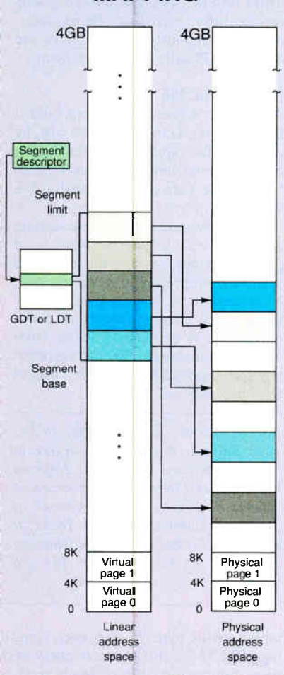
Figure 5: When combined, segmentation and paging result in a system that provides protection without causing memory fragmentation. Segments are used for program protection, and paging is used to map programs into physical memory in fixed-size chunks.
