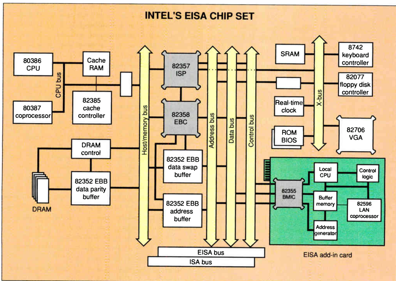
Figure 3: The Intel chip set for supporting EISA consists of the 82358 EISA Bus Controller, the 82357 Integrated System Peripheral, and the 82355 Bus Master Interface Controller.
