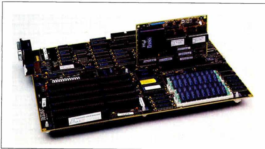
Photo 5: The PowerFlex 80486 CPU upgrade module, installed on the motherboard. The hardest part of installing this card is removing the 80287 math coprocessor, if necessary.
