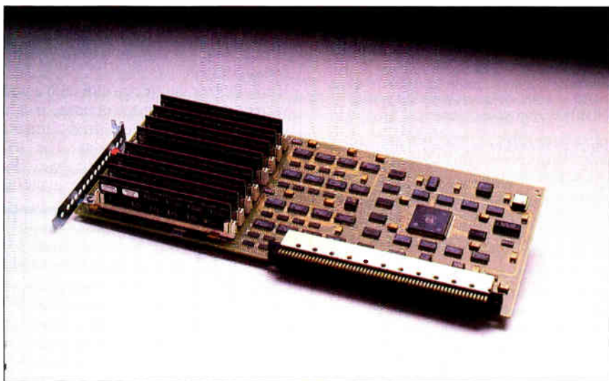
Photo 2: The Vectra 486 system memory board. Memory can be configured with 1-megabit or 4-megabit single in-line memory modules, allowing up to 64 megabytes of system memory. The large chip on the right side of the memory board is HP's custom memory controller (the bursting memory controller shown in the figure).
