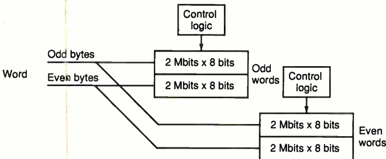
Case 4: Word interface, word interleave control
