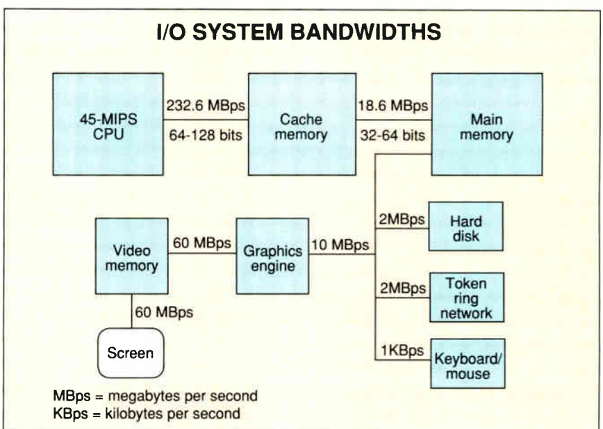
Figure 3: Different I/O devices have different bandwidth needs.
