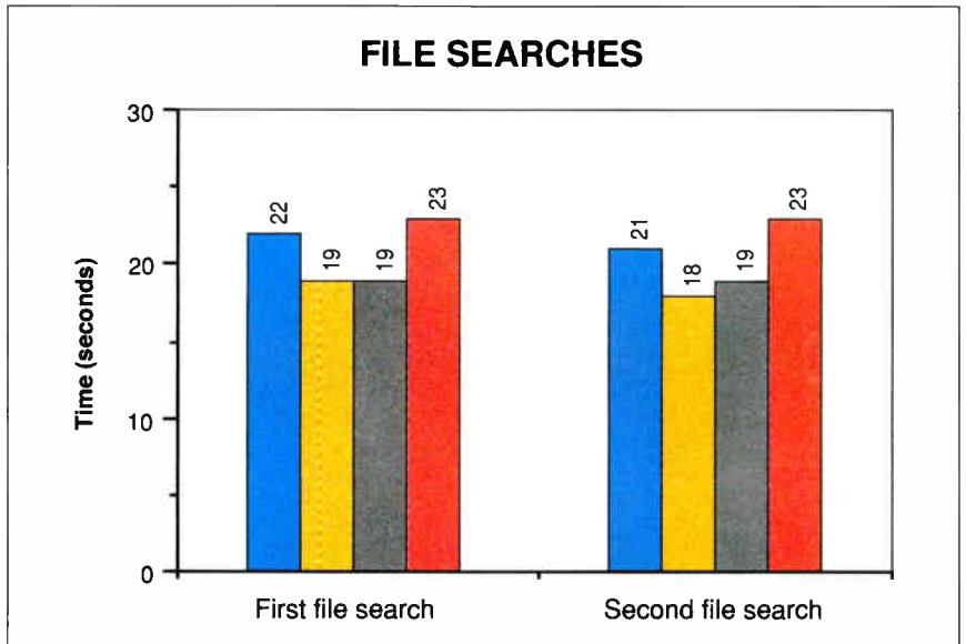
Figure 2: In searches for a file among lots of files, FlashTalk was slower than even standard LocalTalk.
