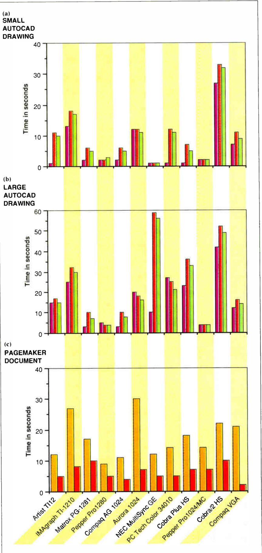
Figure 1: Graphs of our benchmark results: Each graph shows actual time in seconds, so smaller bars mean better performance. Times for Compaq's VGA card are included for comparison. (a) The small AutoCAD drawing, designed to require a display list of less than 512K bytes, tracks the effectiveness of each display-list processor. (b) Most boards couldn't hold the display list of the large AutoCAD drawing in memory, but boards with disk-overflow capability (Compaq 1024 and Pro1280) handled redraws gracefully. (c) PageMaker Zoom and Scroll tests reflect the effectiveness of a card's Windows driver.
