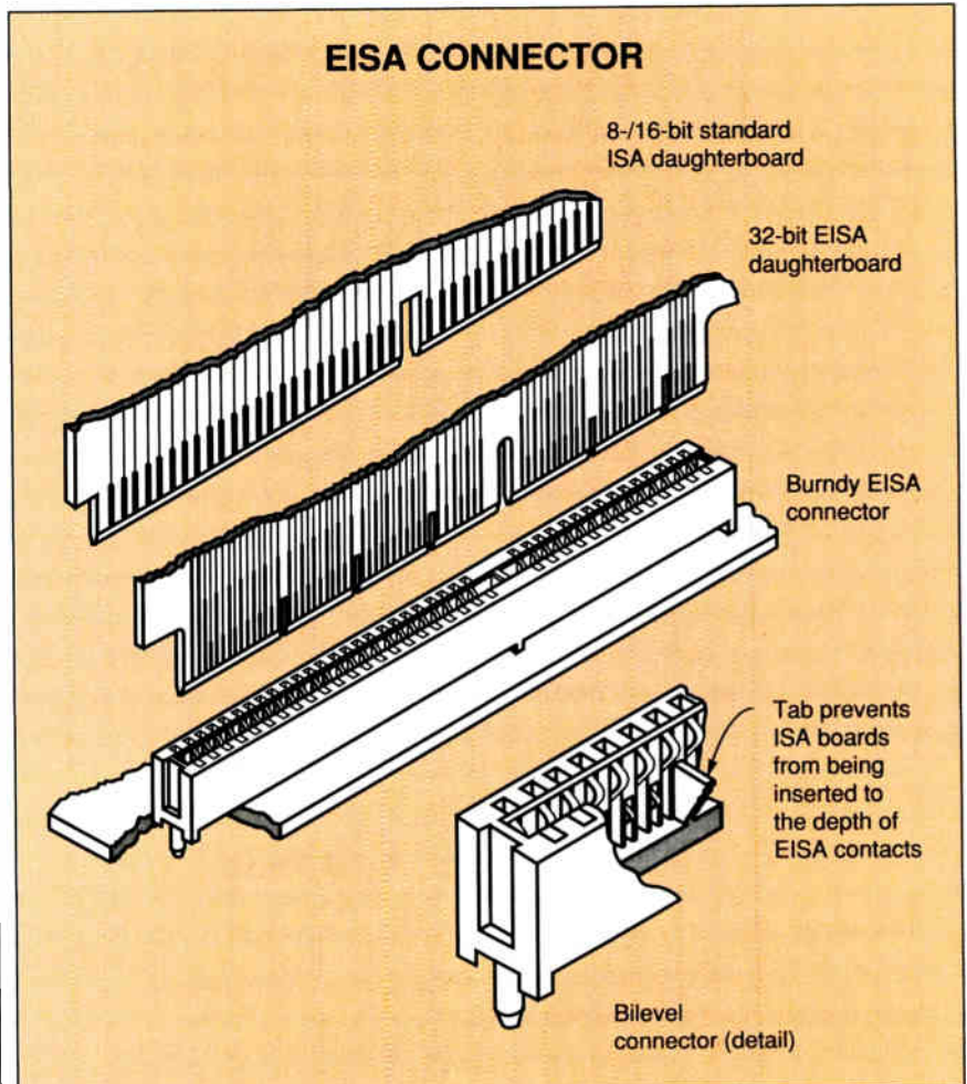
Figure 2: The EISA two-level expansion card connector allows backward compatibility with the ISA card in the same slot, while letting EISA cards have twice as many signal lines.
