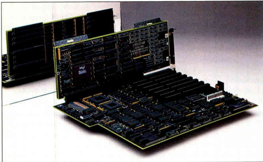
Photo 3: The GPX-486 CPU board, burst-memory-array memory board, and main system board. The system design supports up to 33-MHz 80386 or 80486 operation.
