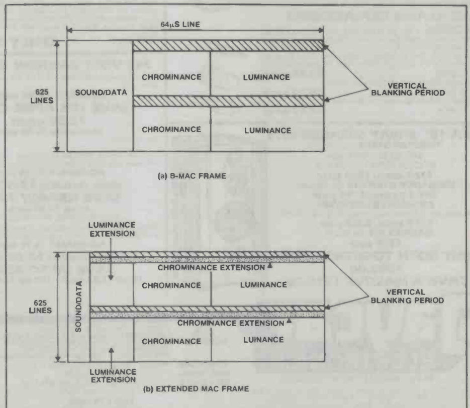
Figure 6. How BMAC can be used to widen the picture.
