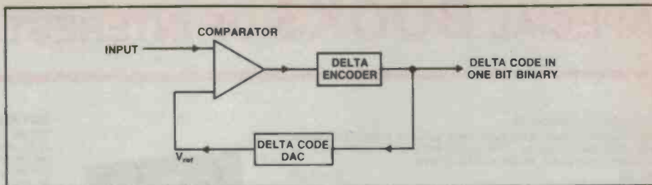
Figure 8. Block diagram for a delta conversion system. Note that the DAC must have knowledge of past conversions in order to produce V_{ref} .
