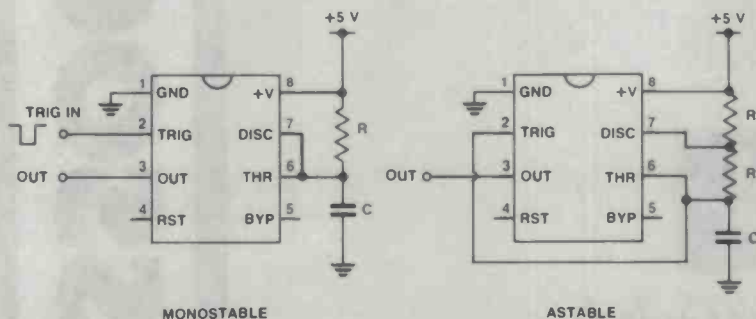
Figure 9. The 555 timer.
