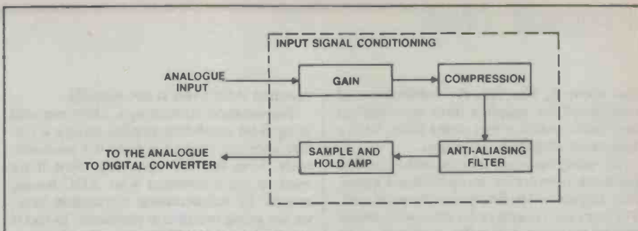
Figure 4. Steps that can be taken to prepare the input signal for the ADC.
