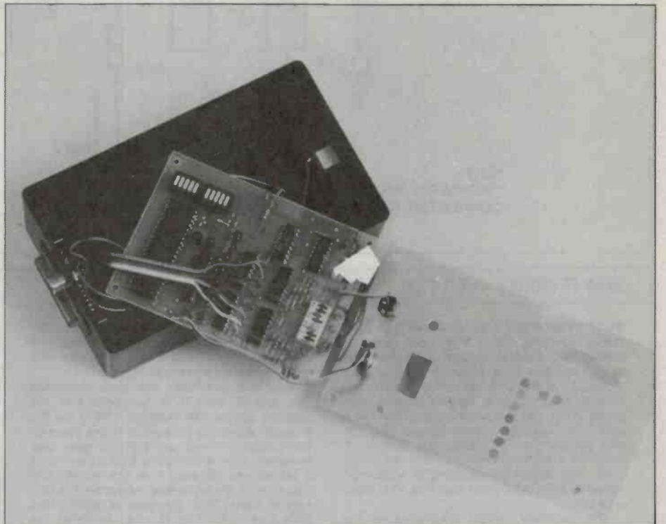
Placement of components on the pc board.
