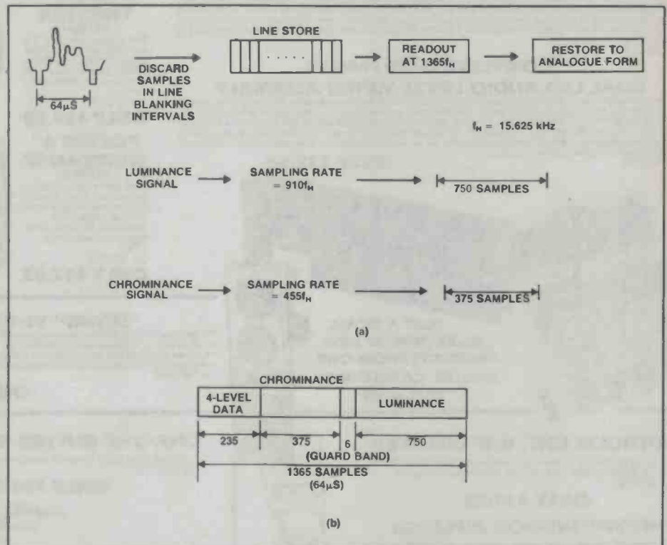
Figure 5. Formation of a BMAC line; a) time compression; b) complete line format.
