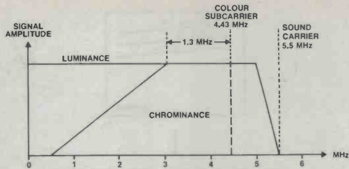
Figure 2. PAL baseband frequency. Note how colour and brightness are mixed in the shaded region.
