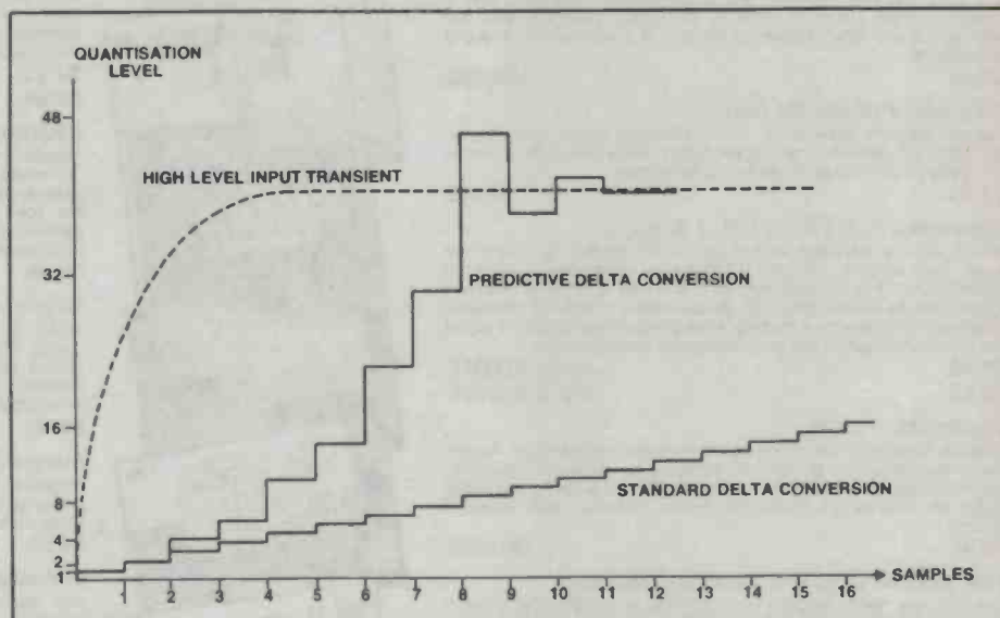
Figure 9. The response to fast changing inputs is much better for predictive delta conversions.
