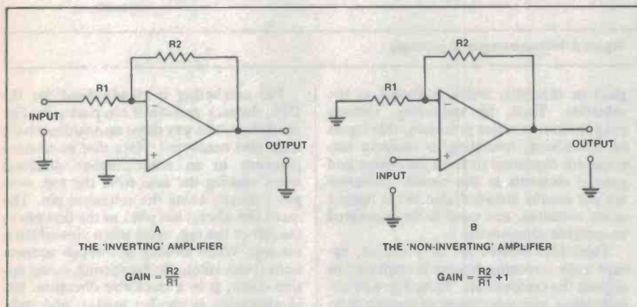
Figure 5. Op-amps as amplifiers.
