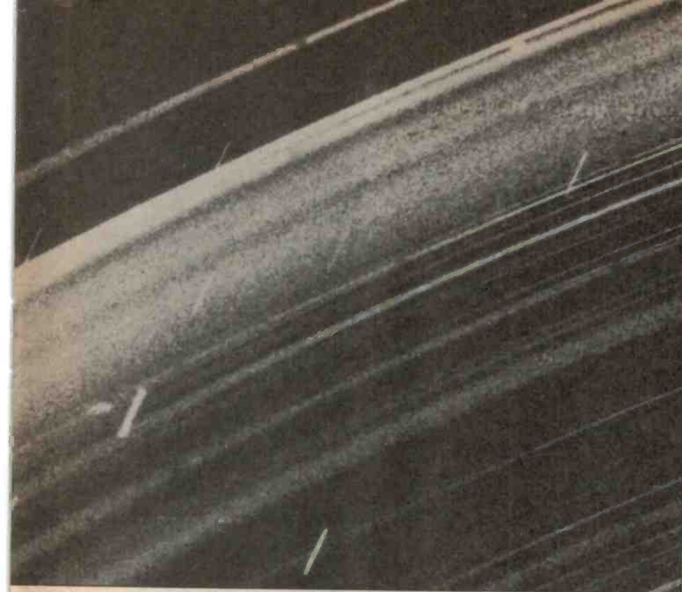
Left. The rings of Uranus. Voyager 2 was 236,000 km from the planet, looking back at sunlight refracted by small dust particles in the rings when this was taken. The streaks are stars, caused by panning the camera during the 96 second exposure.
