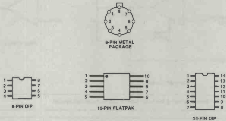
Figure 3. Pin numbering of IC packages.
