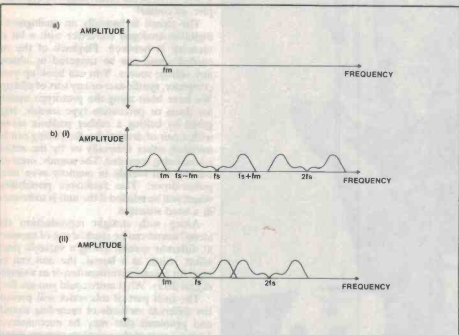
Figure 3(a). The spectrum of the original system; (b) the spectra of pulses representing sample values of the original signal at (i) f_s > 2f_m and (ii) f_s < 2f_m .
