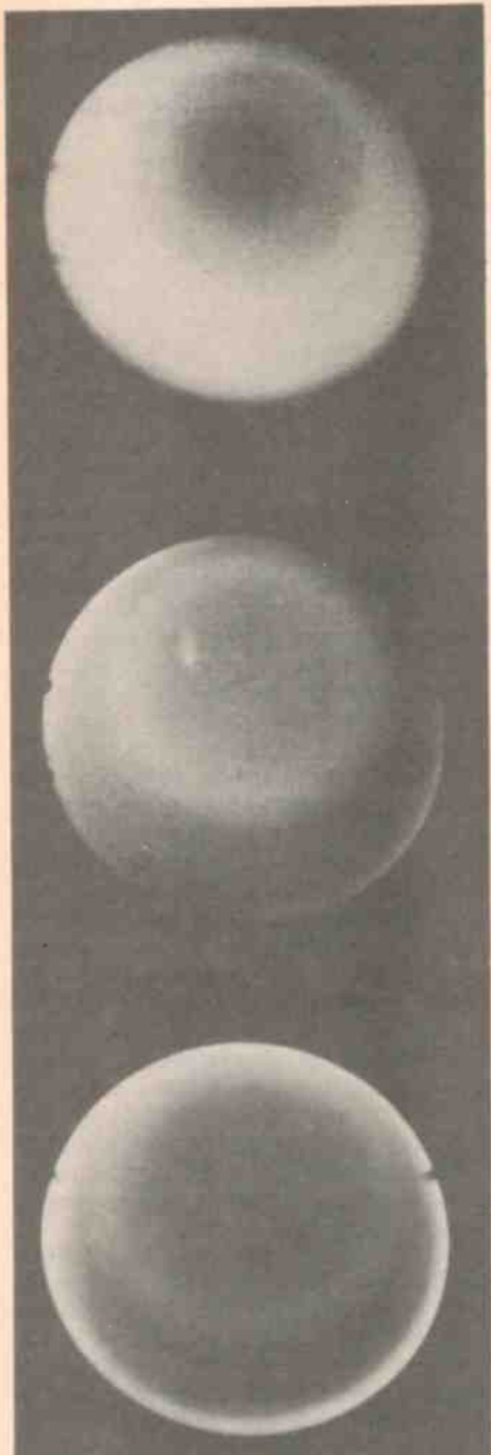
Colour Imaging from Voyager. These three computer enhanced images of Uranus, taken from 2.1 million km, show the view through violet, orange and methane filters. Later they can be combined to provide a composite colour image. These images are themselves quite removed from the originals received at Parkes. JPL uses a correlation technique, in which each picture is broken up into its discrete pixels, and then copied time and time again.
