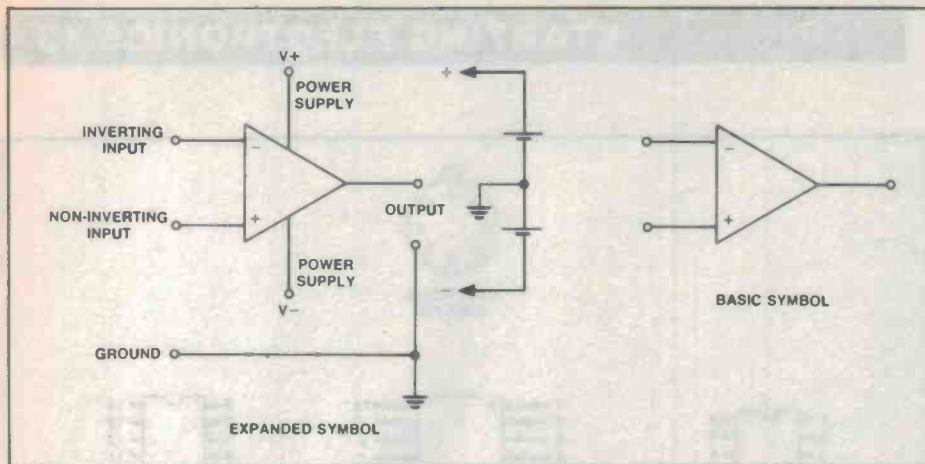
Figure 4. The op-amp, showing the basic symbol and an expanded symbol.
