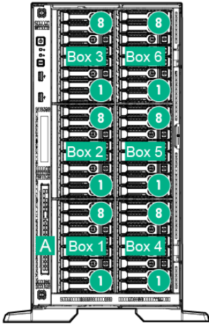
48 SFF hot-plug drive model (Tower)
