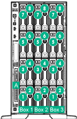
24 LFF hot-plug drive model (Tower)
