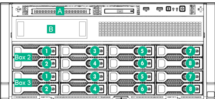
16 LFF hot-plug drives with LFF media cage
