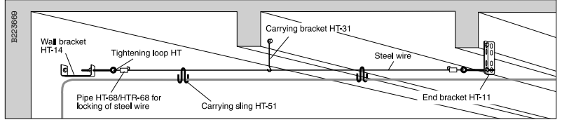
Steel wire installed in ceiling with beams.
