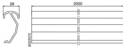
Profile protection 28P
