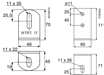
Angle bracket 5L
