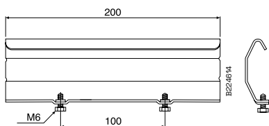
Joint 21 in stainless steel
