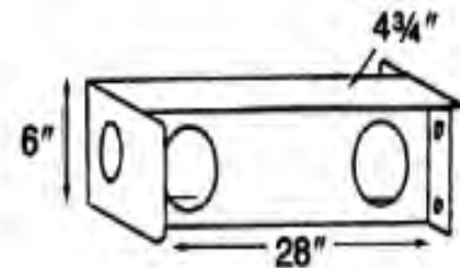
HEIL ALUMINUM #1513508 CURBSIDE #1513509 ROADSIDE
