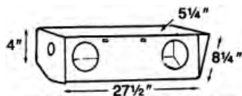
HEIL OR BUTLER STAINLESS STEEL #151381965 CURBSIDE #151381966 ROADSIDE
