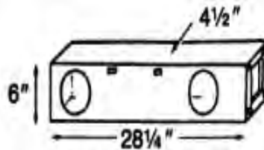
HEIL ALUMINUM #1512935 LEFT OR RIGHT
