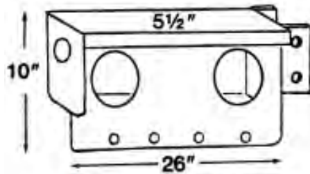
FRUEHAUF ALUMINUM #TKG00531 ROADSIDE #TKG00532 CURBSIDE
