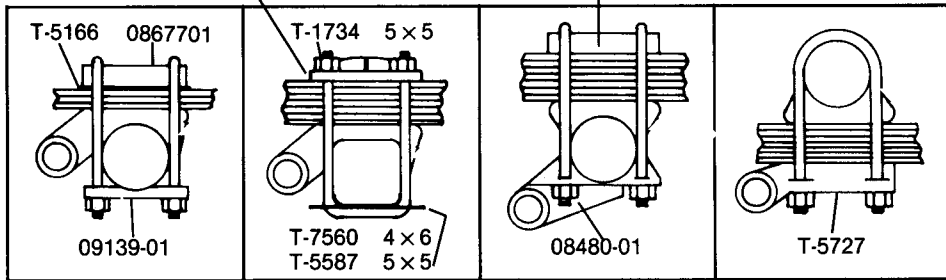
INVERTED U-BOLTS
