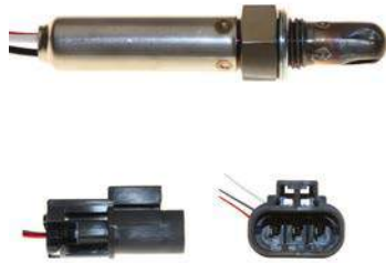
250-23502 NISS (4,6) 1986-96 Heated Sensor, 240mm 3wire
