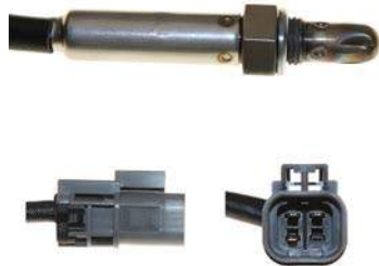
250-23504 NISS (6) 1987-89 Heated Sensor, 430mm 3wire
