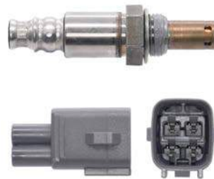
250-54006 LEXUS (8) 2007-14 / PONT (4) 2005-10 SCION (4) 2008-09 / TOY (4,6,8) 2001-21 Air/Fuel Sensor, 400mm 4wire
