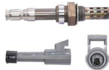
250-21029 SAT (4) 1991-94 Unheated Sensor, 130mm 1wire
