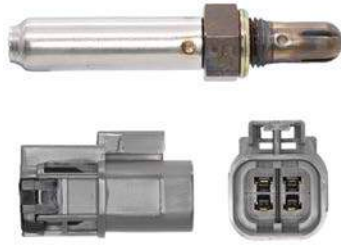
250-24506 NISS (6) 1987-88 Heated Sensor, 1160mm 4wire
