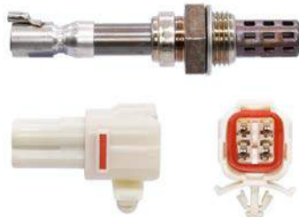
250-22069 LEXUS (6) 1990-91 / TOY (6) 1990-91 Unheated Sensor, 325mm 2wire
