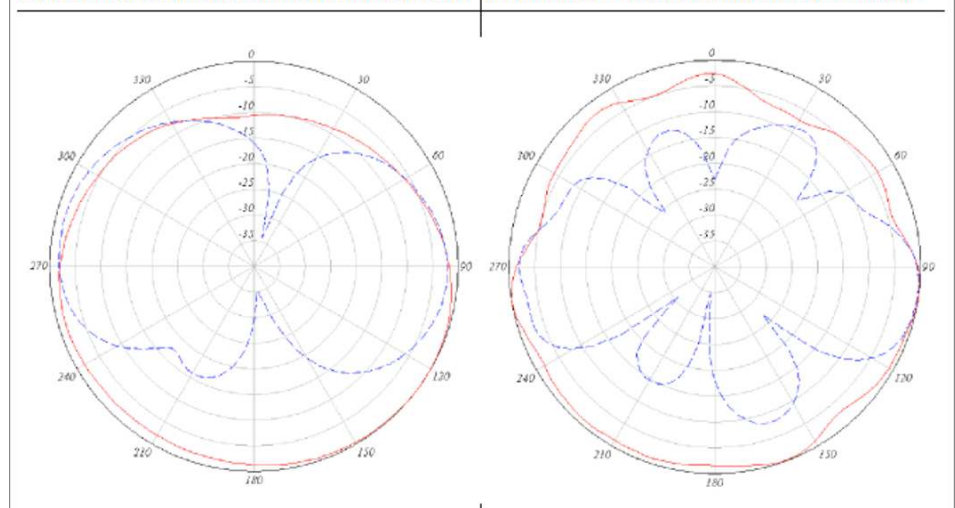
2.4-GHz Antenna 2 Azimuth and Elevation Plane Patterns | 5-GHz Antenna 2 Azimuth and Elevation Plane Patterns
