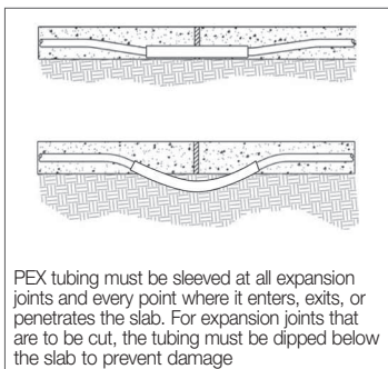
Installing PEX under a slab
