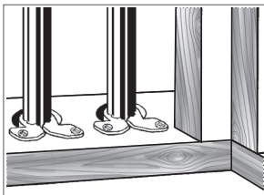
Suspension clip fasteners used at floor plate
