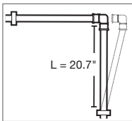
Corner Expansion Example
