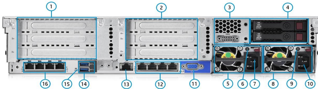
Rear view
