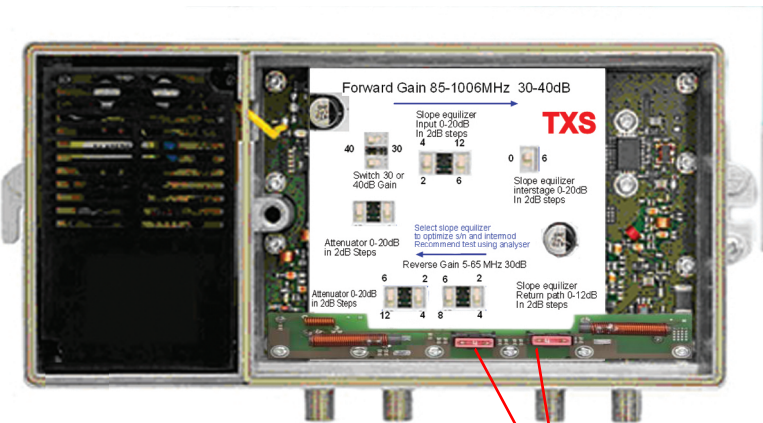
Links to route line power via input or output or through
