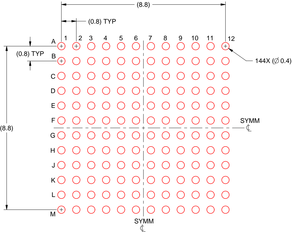
SOLDER PASTE EXAMPLE BASED ON 0.15 mm THICK STENCIL SCALE:8X
