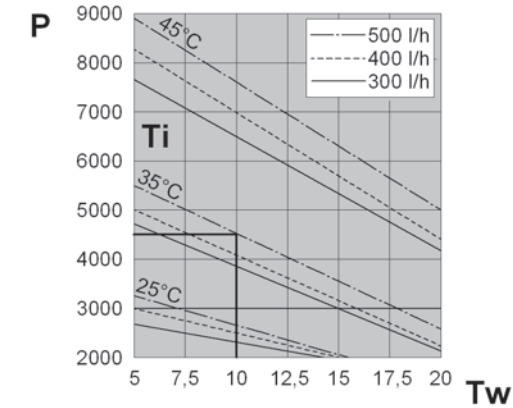
PERFORMANCE
