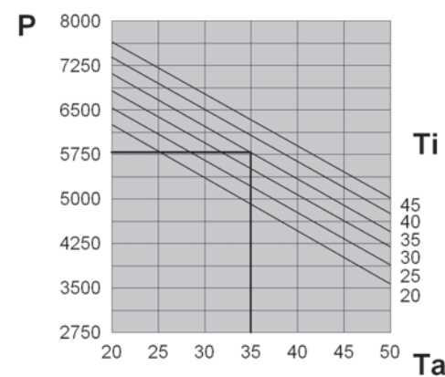
PERFORMANCE (EGO60MTEB)
