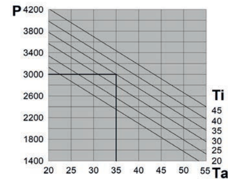
PERFORMANCE
