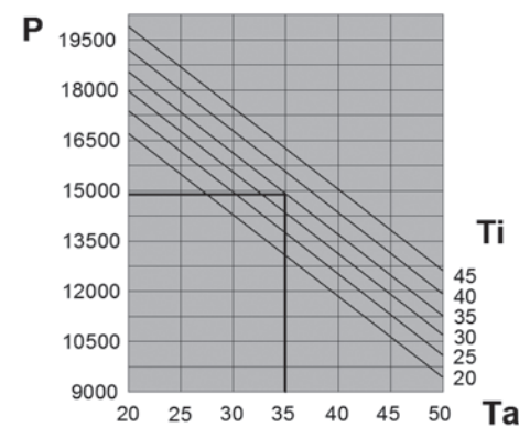
PERFORMANCE (EGOA5MTEB)
