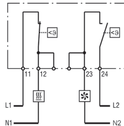
CONNECTION DIAGRAM
