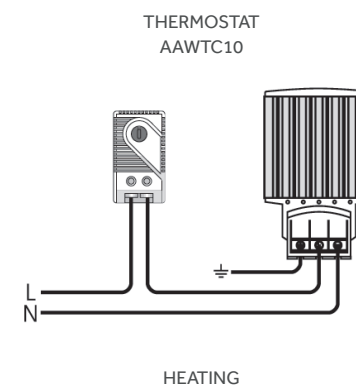
HEATING
