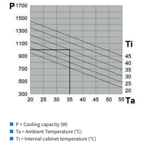
PERFORMANCE
