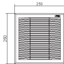
DRILLING TEMPLATE
