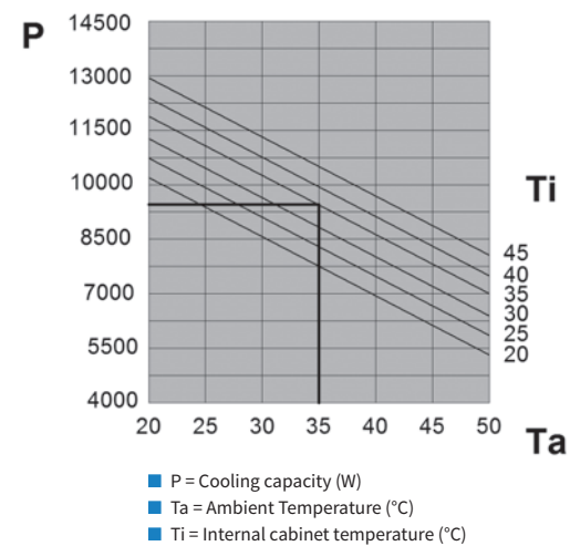
PERFORMANCE (EMOA0MMEB)
