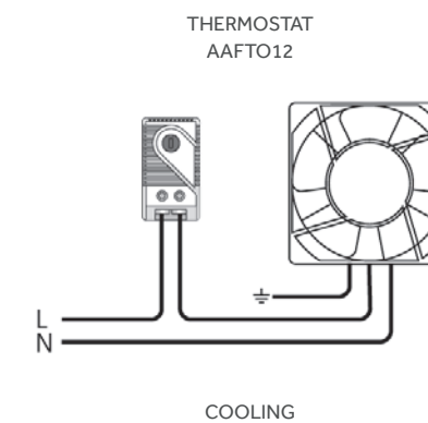
COOLING
