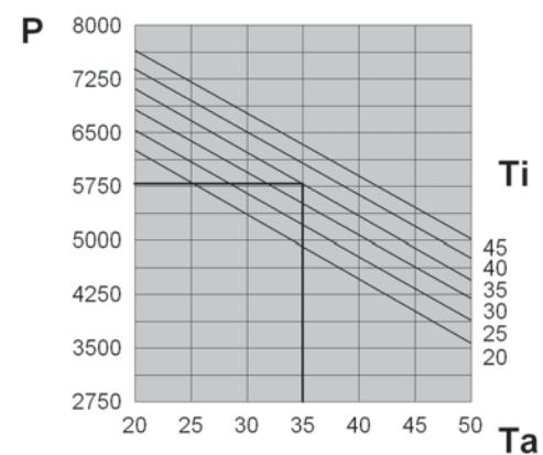
PERFORMANCE (EMO60MMEB)
