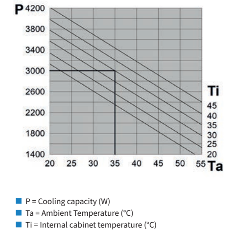
PERFORMANCE
