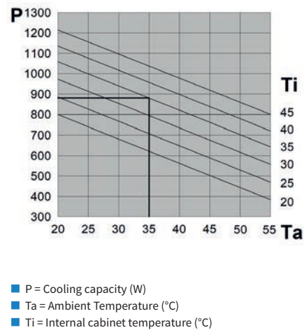
PERFORMANCE
