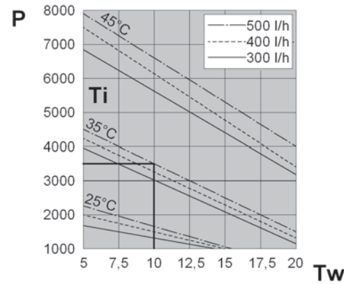
PERFORMANCE
