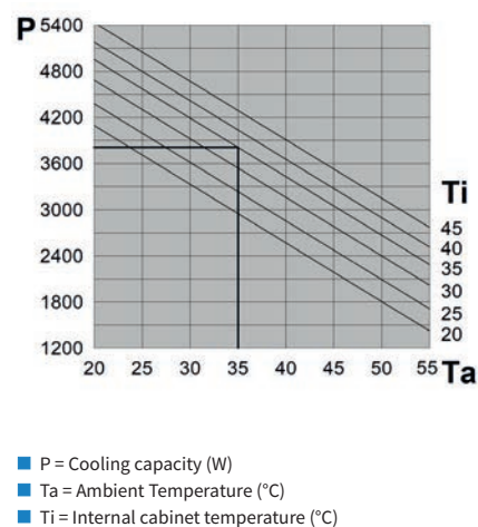
PERFORMANCE
