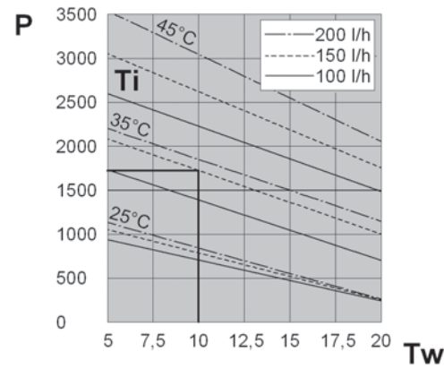
PERFORMANCE
