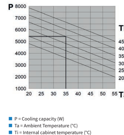
PERFORMANCE
