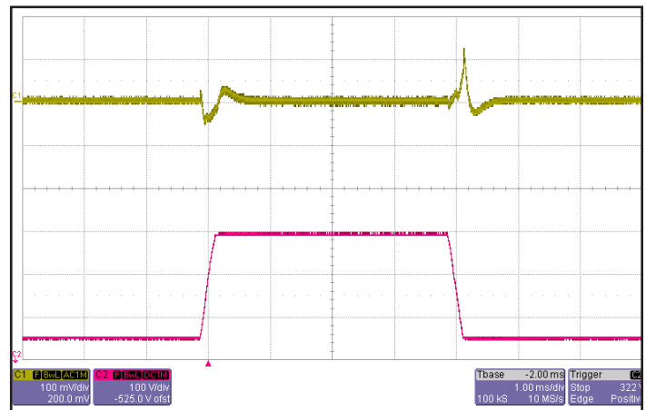
Figure 6: Output voltage response to step-change in input voltage (180 V - 425 V - 180 V) with 250 μs rise/fall time. Load cap: 15μF, 100 mΩ ESR tantalum cap and 1μF ceramic cap. Ch 1: V out (100mV/div). Ch 2: V in (100V/div).
