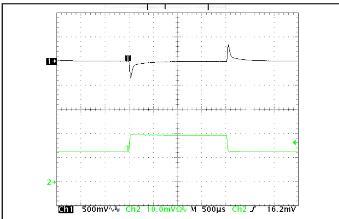
Figure 5: Output voltage response to step-change in load current (50%-75%-50% of Iout(max)); dI/dt = 0.1A/μs. Load cap: 15μF, 100 mΩ ESR tantalum cap and 1μF ceramic cap. Ch 1: Vout (500mV/div), Ch 2: Iout (5A/div).
