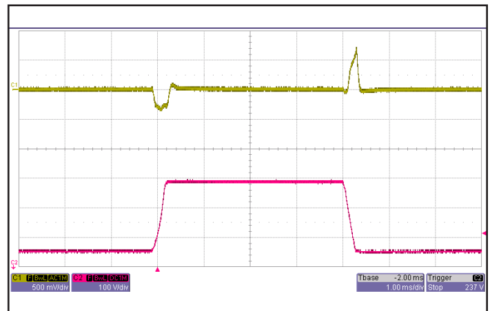
Figure 6: Output voltage response to step-change in input voltage (180 V - 425 V - 180 V) with 250 μs rise/fall time. Load cap: 15μF, 100 mΩ ESR tantalum cap and 1μF ceramic cap. Ch 1: V out (500mV/div). Ch 2: V in (100V/div).
