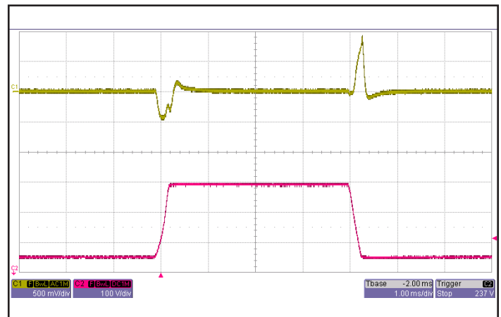
Figure 6: Output voltage response to step-change in input voltage (180 V - 425 V - 180 V) with 250 \mu s rise/fall time. Load cap: 15 \mu F , 100 m \Omega ESR tantalum cap and 1 \mu F ceramic cap. Ch 1: V_{out} (500mV/div). Ch 2: V_{in} (100V/div).
