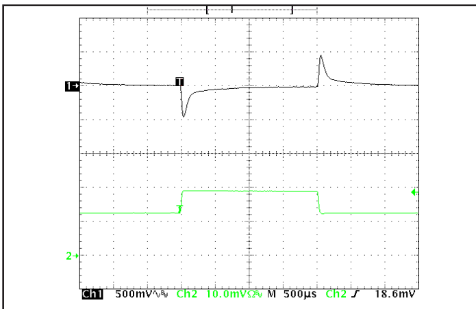
Figure 5: Output voltage response to step-change in load current (50%-75%-50% of I out (max); dI/dt = 0.1A/μs). Load cap: 15μF, 100 mΩ ESR tantalum cap and 1μF ceramic cap. Ch 1: V out (500mV/div), Ch 2: I out (1A/div).
