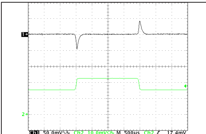
Figure 5: Output voltage response to step-change in load current (50%-75%-50% of I out (max); dI/dt = 0.1A/μs). Load cap: 15μF, 100 mΩ ESR tantalum cap and 1μF ceramic cap. Ch 1: V out (50mV/div), Ch 2: I out (10A/div).
