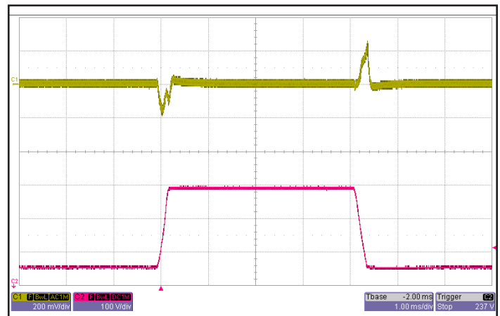
Figure 6: Output voltage response to step-change in input voltage (180 V - 425 V - 180 V) with 250 µs rise/fall time. Load cap: 15µF, 100 mΩ ESR tantalum cap and 1µF ceramic cap. Ch 1: Vout (200mV/div). Ch 2: Vin (100V/div).
