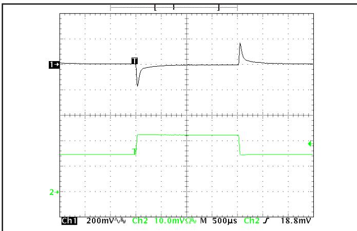
Figure 5: Output voltage response to step-change in load current (50%-75%-50% of Iout(max); dI/dt = 0.1A/us). Load cap: 15µF, 100 mΩ ESR tantalum cap and 1µF ceramic cap. Ch 1: Vout (200mV/div), Ch 2: Iout (10A/div).
