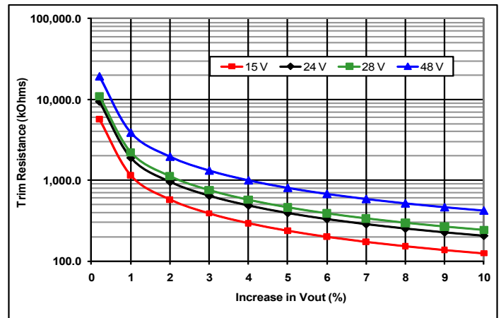
Common Figure 4: Trim-Up Graph for 15 to 48V outputs.
