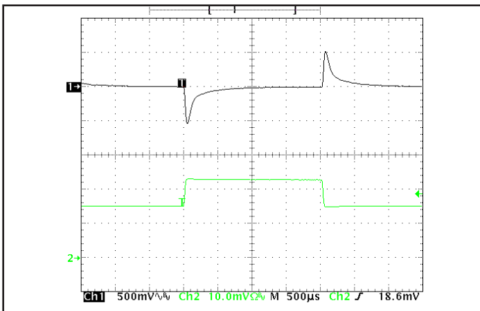
Figure 5: Output voltage response to step-change in load current (50%-75%-50% of I_{out(max)} ; dI/dt = 0.1A/\mu s ). Load cap: 15 \mu F , 100 m \Omega ESR tantalum cap and 1 \mu F ceramic cap. Ch 1: V_{out} (500mV/div), Ch 2: I_{out} (2A/div).
