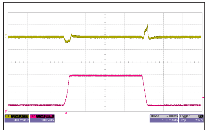
Figure 6: Output voltage response to step-change in input voltage (180 V - 425 V - 180 V) with 250 μs rise/fall time. Load cap: 15μF, 100 mΩ ESR tantalum cap and 1μF ceramic cap. Ch 1: Vout (500mV/div). Ch 2: Vin (100V/div).
