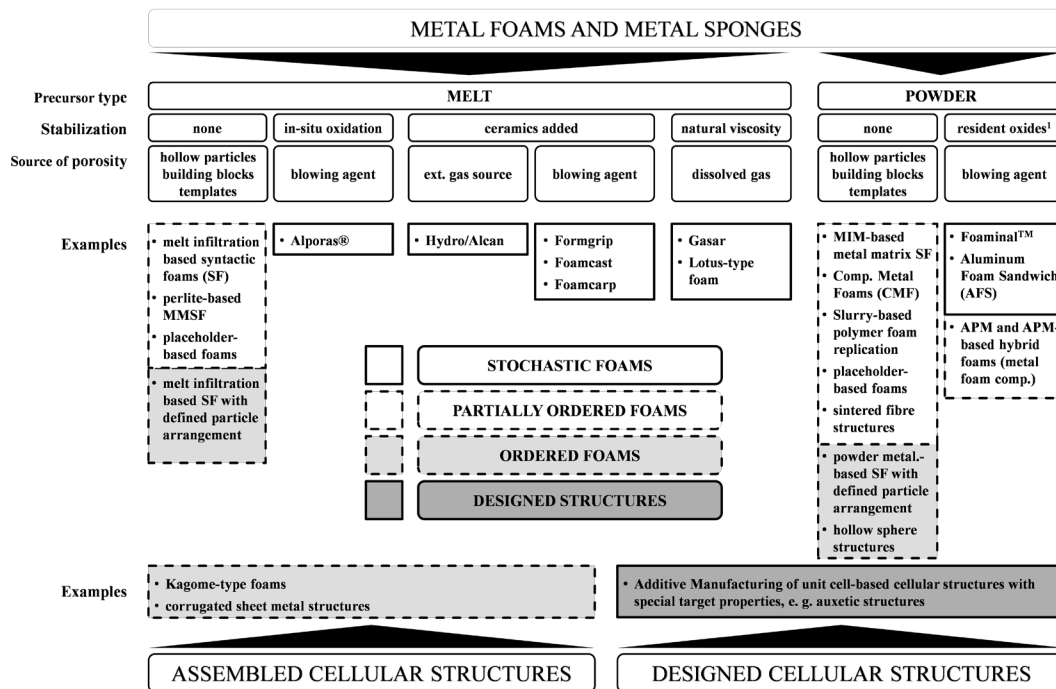
Fig. 2. Overview of manufacturing processes and cellular metals [12]
