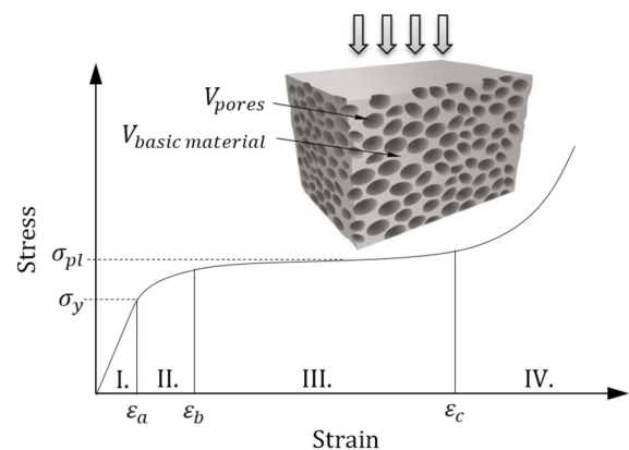
Fig. 1. Characteristic response of the cellular structure under compression loading [5]
