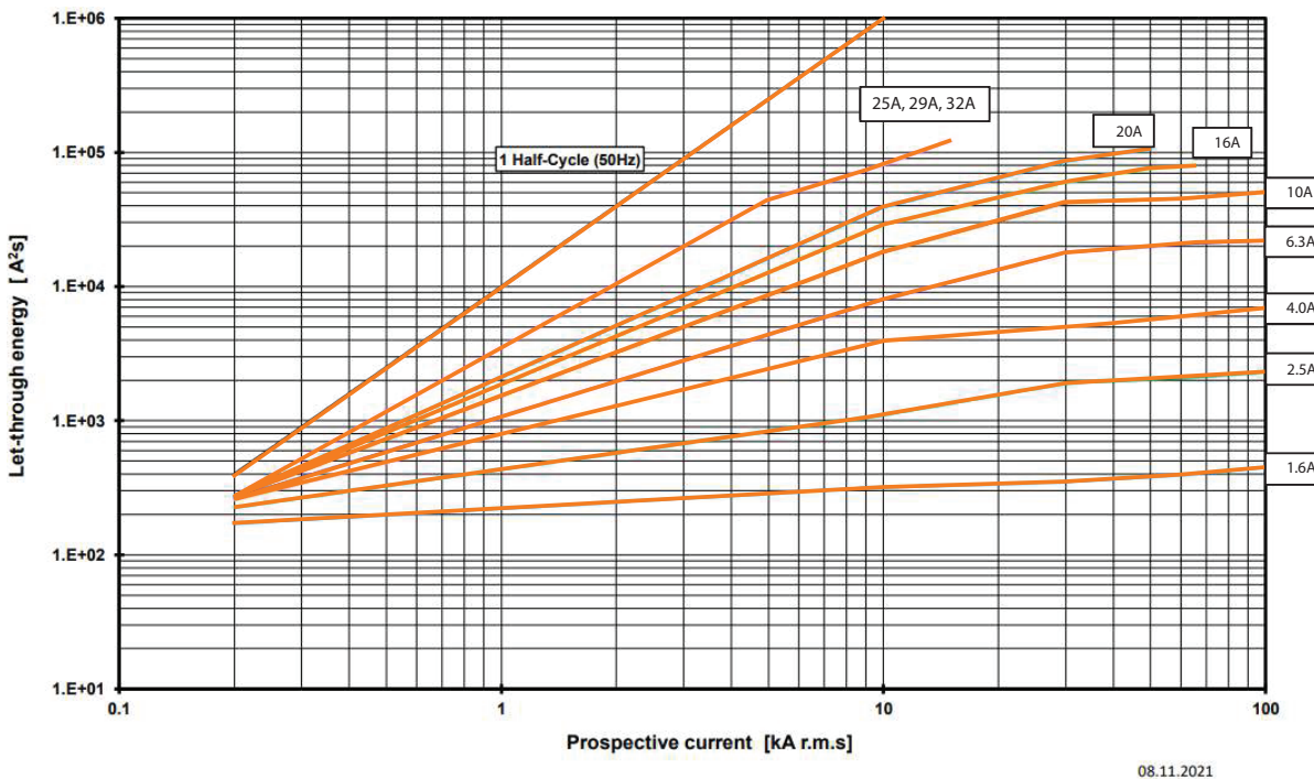
KTA9-32S-* Max. Let-Through-Energy at U_o = 400V / 415V, 50Hz
