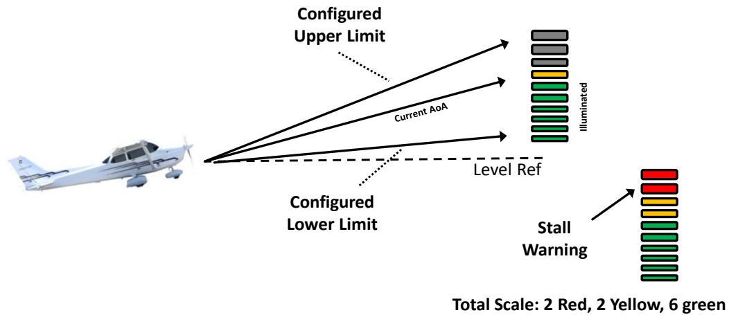
Figure 33 – AoA Upper and Lower Limits
