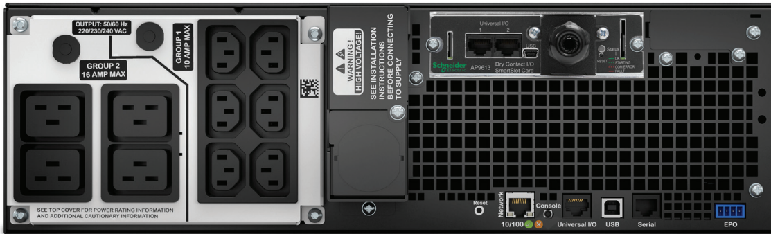
SRT5KRMXLIM UPS in rackmount configuration
