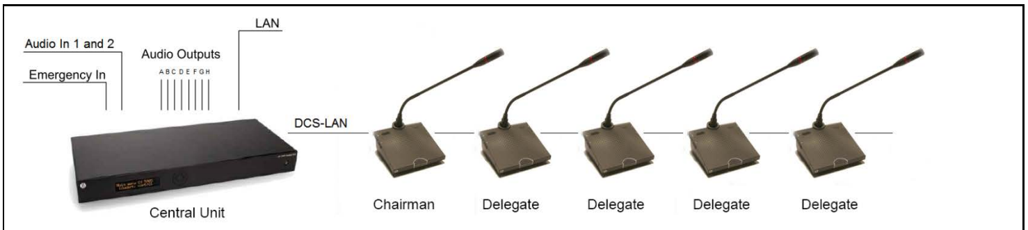
Figure 0-A Connecting DCS 6000 conference units.
