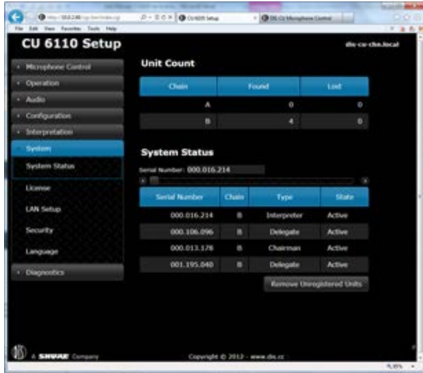
Figure 0-E CU6110 Setup Tab selected
