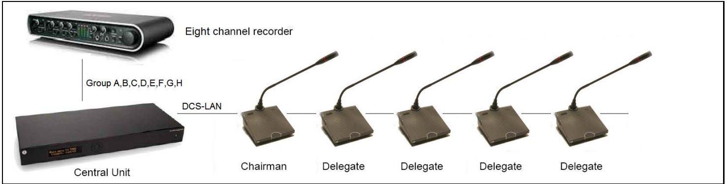
Figure 0-E Connecting the DCS 6000 Digital Conference System to an audio recorder.
