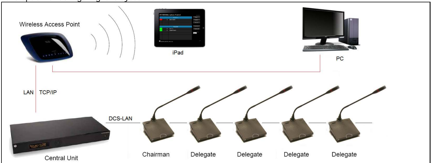
Figure 0-D Connecting the DCS 6000 Digital Conference System to a PC and an iPad
