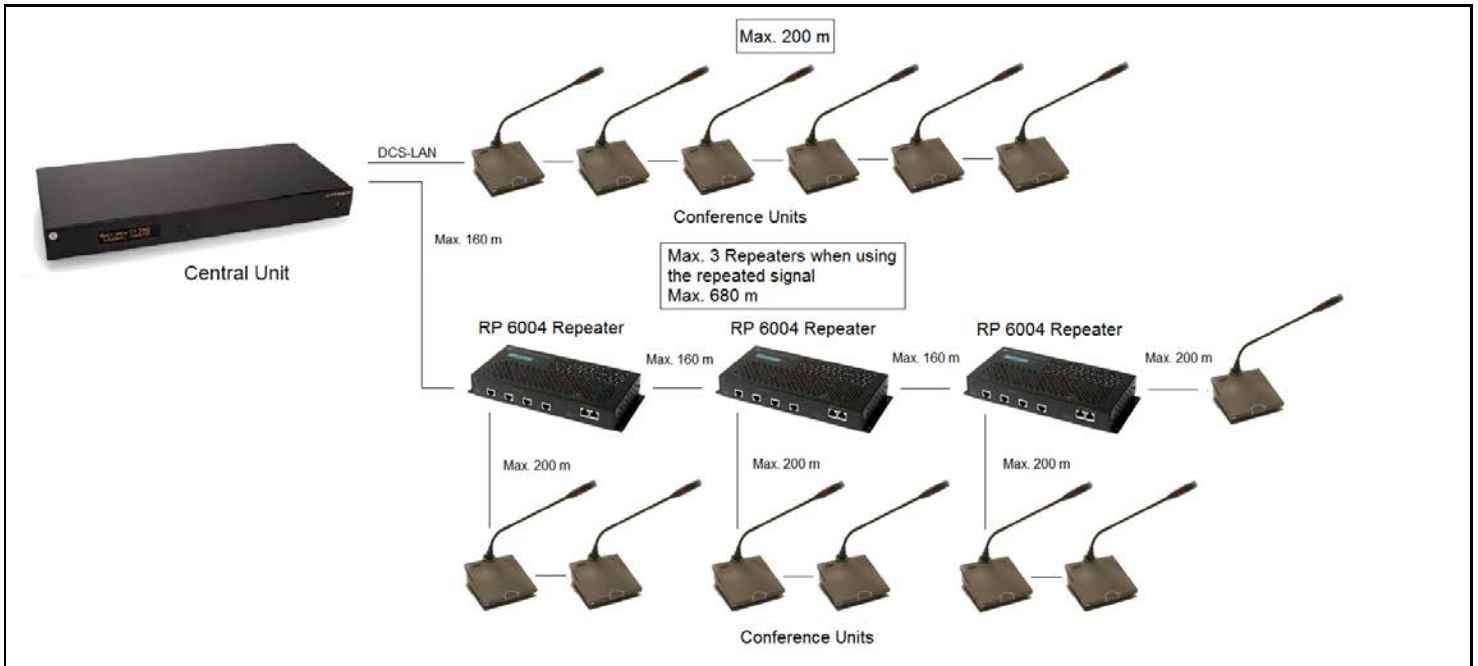
Figure 0-I DCS 6000 Digital Conference System with RP 6004 Repeater.
