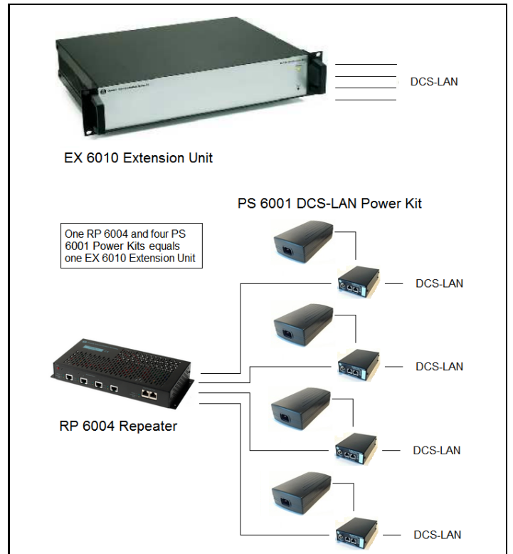
Figure 0-J DCS 6000 Digital Conference System with PS 6001.
