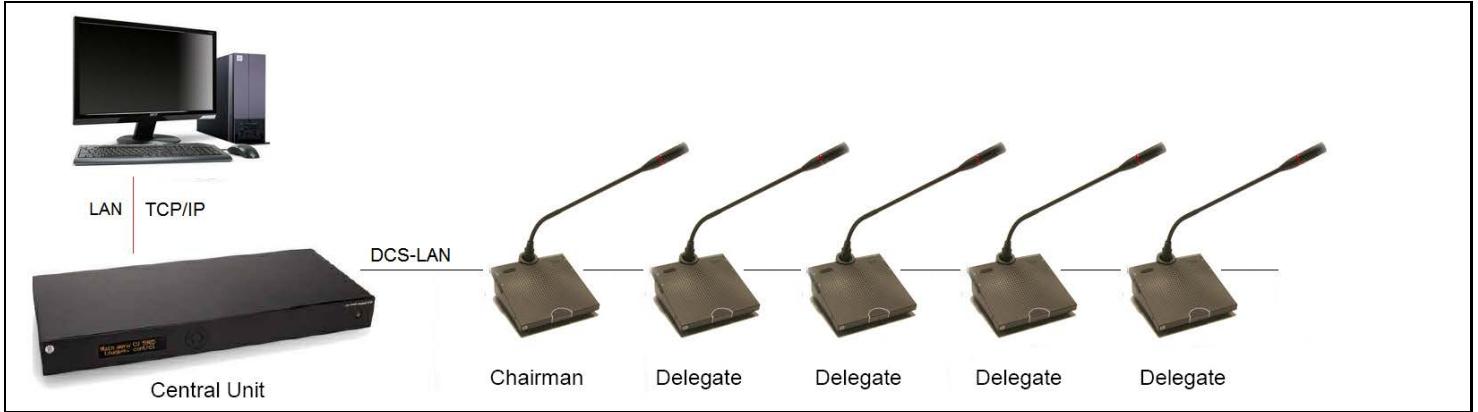
Figure 0-C Connecting the DCS 6000 Digital Conference System to a PC
