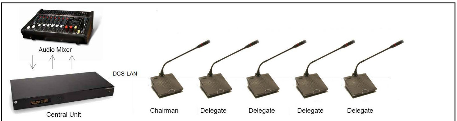
Figure 0-F Connecting the DCS 6000 Digital Conference System to an audio mixer.
