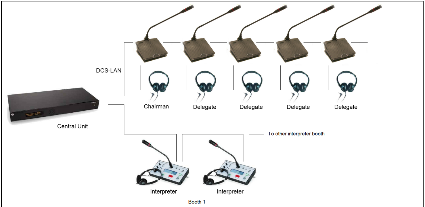
Figure 0-G DCS 6000 Digital Conference System with interpretation functionality.
