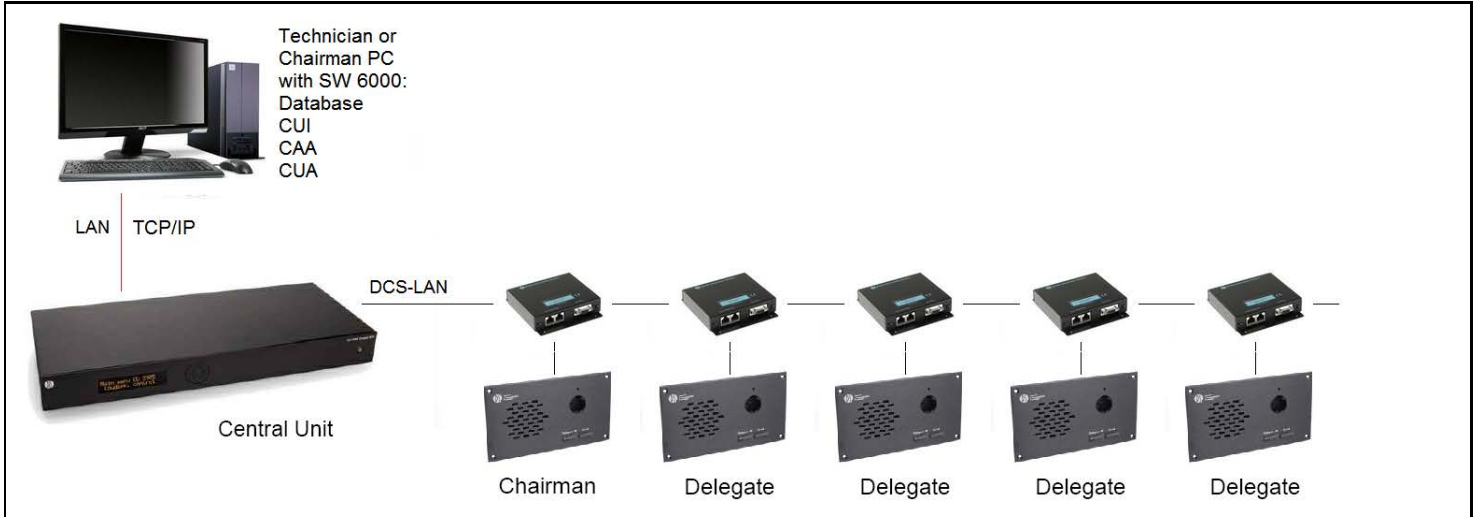
Figure 0-K DCS 6000 Digital Conference System with basic SW 6000 setup
