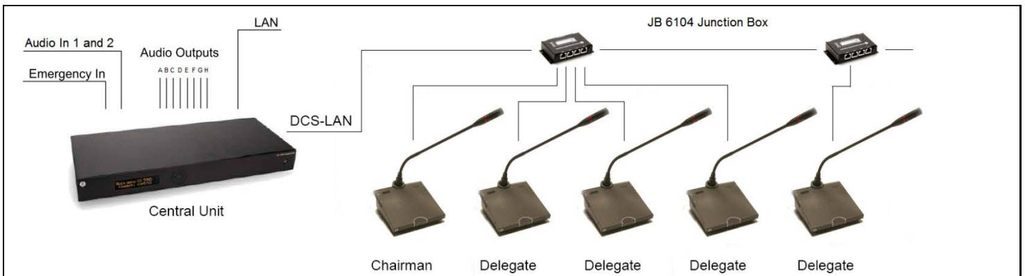
Figure 0-B Connecting DCS 6000 conference units using JB 6104 Junction Boxes.
