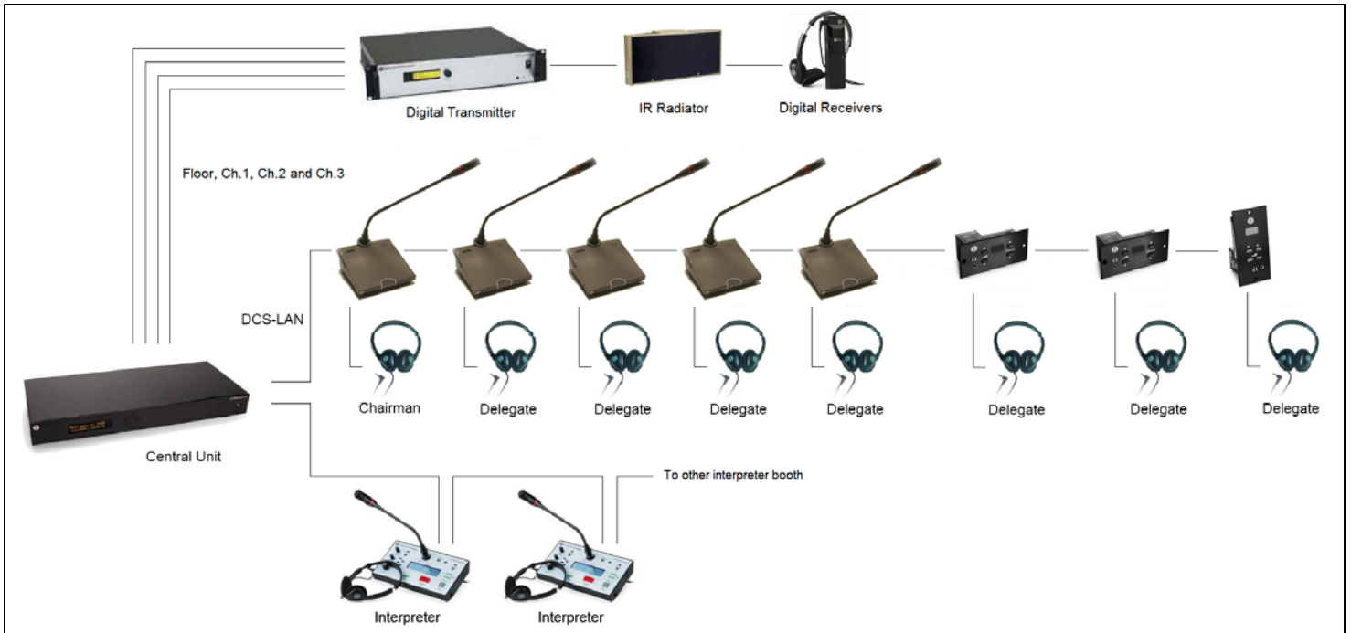
Figure 0-H DCS 6000 Digital Conference System with interpretation and wireless distribution, Floor, Ch.1 to Ch.7
