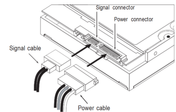
Figure 1 Attaching SATA cabling
