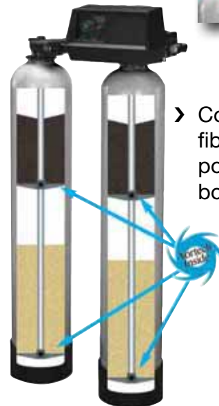
Twin Tank-Dual Chamber
