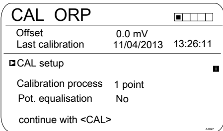
Fig. 50: [ORP] calibration menu
