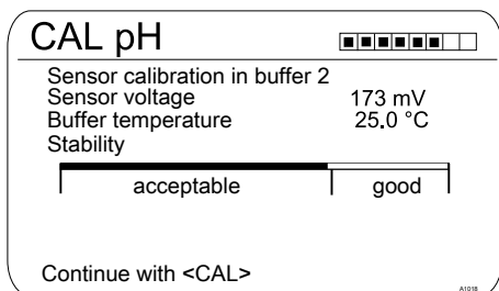
Fig. 44: Display of the sensor stability achieved
