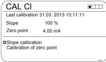
Fig. 63: [Chlorine] calibration menu
