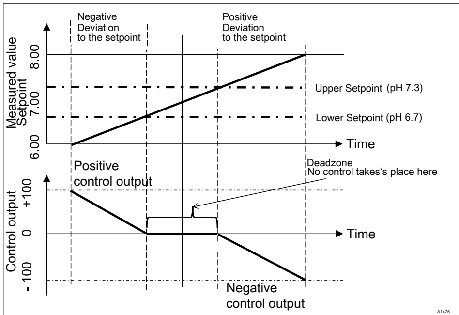
Fig. 87: Control type PID bidirectional, with neutral zone
