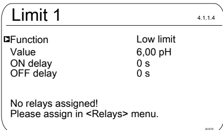
Fig. 98: Setting Limit 1
