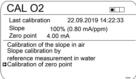
Fig. 80: Introduction: Calibration of the zero point
