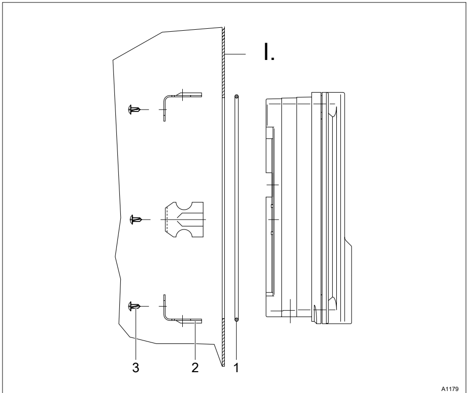
Fig. 14: Order number for the DAC control panel fitting kit (included with the scope of supply): 1041095.
