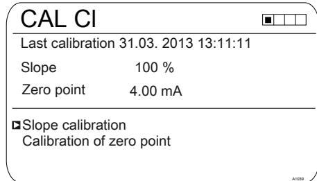
Fig. 37: [Calibration] display with the example of [Chlorine].
