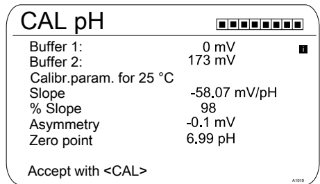
Fig. 38: Display of the calibration result
