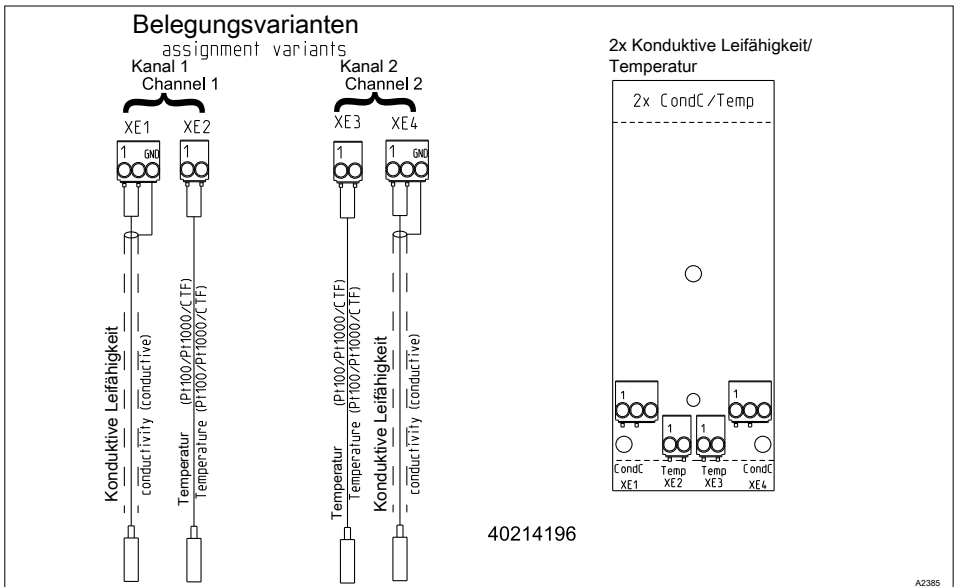
Fig. 26: Module: 2x conductive conductivity/temperature sensors. Part number 734223
