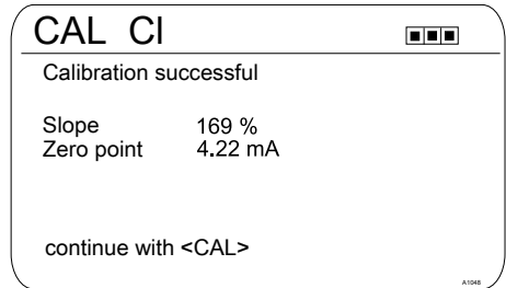
Fig. 68: Calibration of zero point
