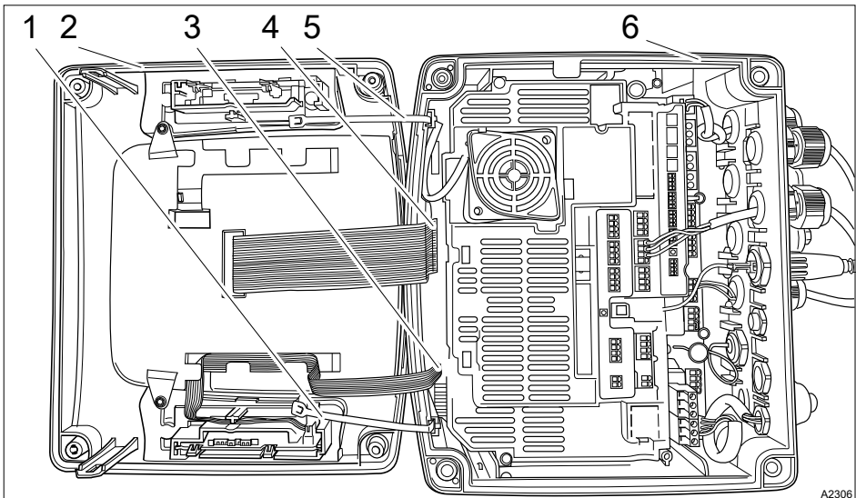
Fig. 129: Replacement of spare parts units
