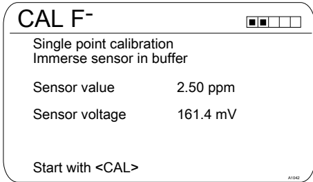
Fig. 61: Fluoride sensor calibration (CAL)
