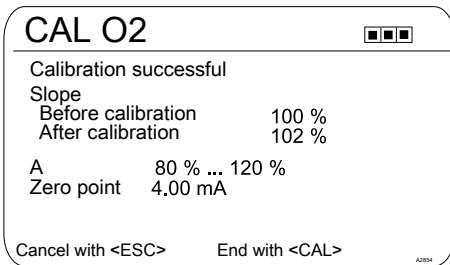
Fig. 78: Successful calibration
