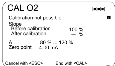
Fig. 83: Unsuccessful calibration
