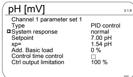
Fig. 85: for the example of pH [mV]: Continuous display → → or [Control] → [Control] → or [Channel 1 parameter set 1] → [Channel 1 parameter set 1]
