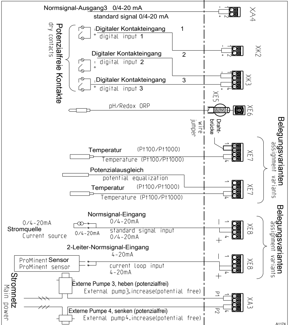
Fig. 20: Terminal diagram for the extension unit (channel 3) with assignment options (module C, optional)
