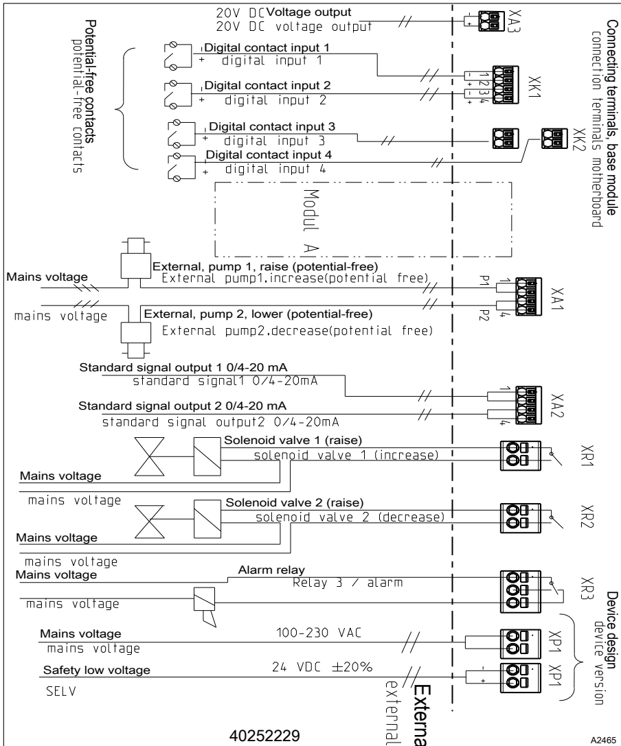
Fig. 19: Terminal diagram with assignment options.
