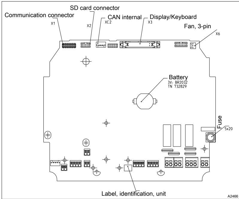
Fig. 23: Service interfaces
