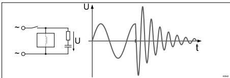
Fig. 28: Switching-off process shown on the oscillogram.
