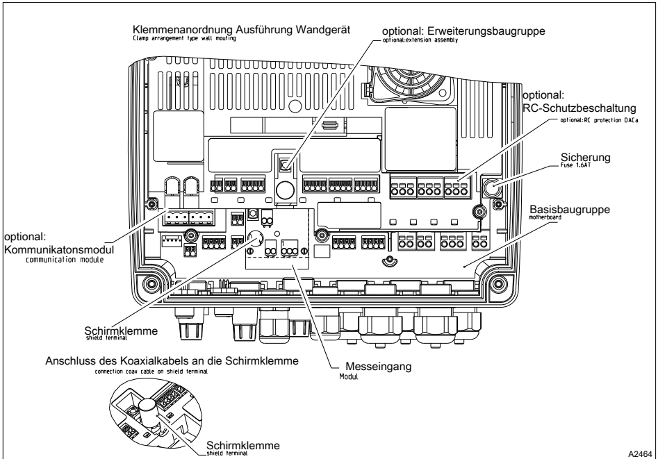
Fig. 18: Terminal layout
