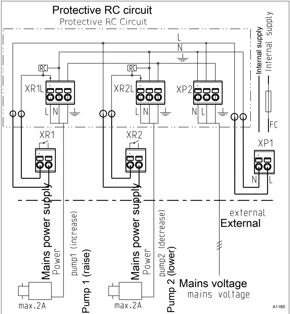
Fig. 21: Terminal diagram with protective RC circuit (module D, optional). The RC unit is only permitted in conjunction with the 230 V design.
