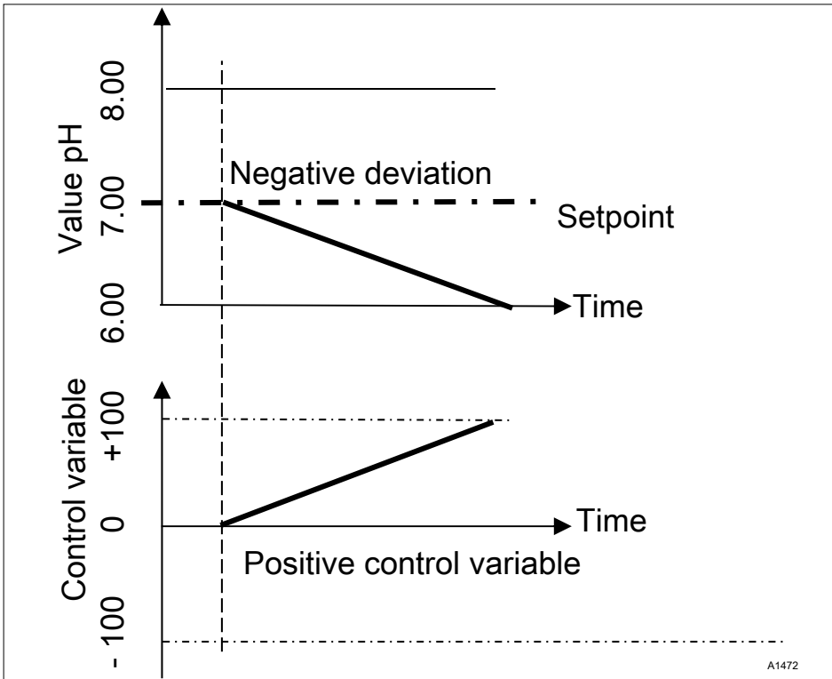
Fig. 89: Control type PID monodirectional, pH-raising direction
