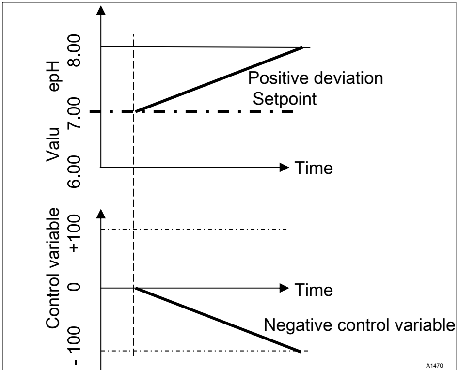
Fig. 88: Control type PID monidirectional, pH-lowering direction
