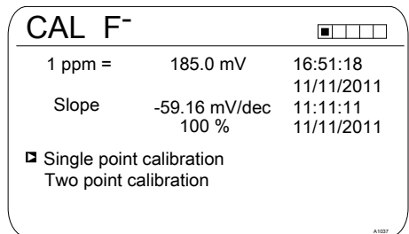
Fig. 57: Calibration menu [Fluoride]
