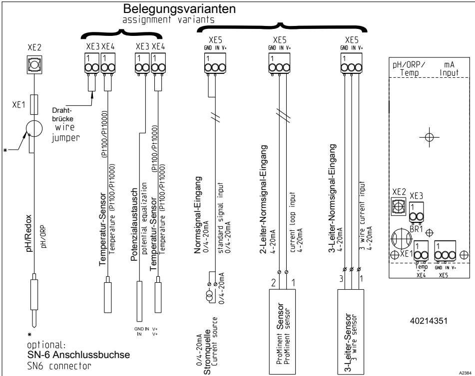
Fig. 24: Module: mV temperature/mA input. Part number 734355
