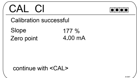
Fig. 66: Calibrating the reference value
