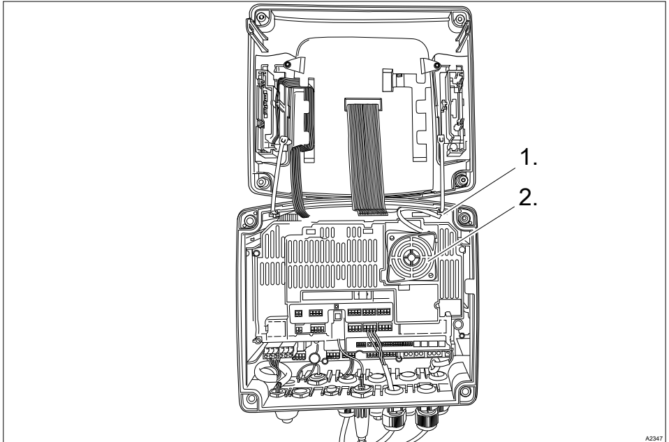
Fig. 130: Replacing fan, part no. 733328
