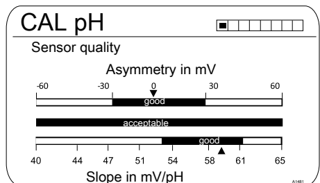
Fig. 39: Displayed after the \blacktriangleright key has been pressed
