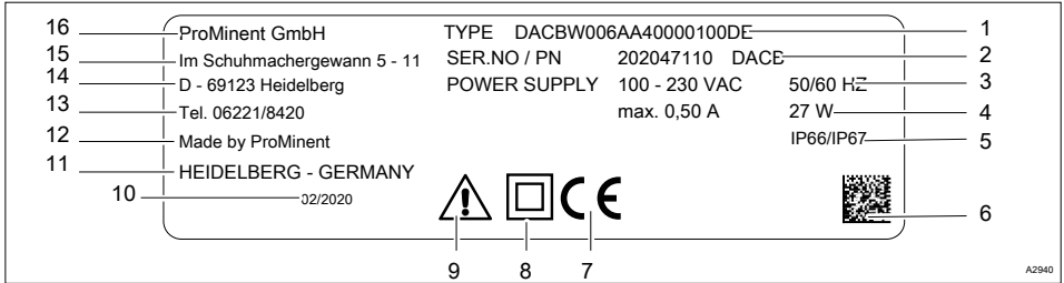
Fig. 9: Nameplate, CE
