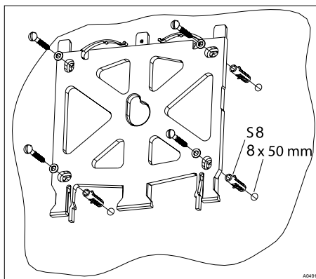
Fig. 12: Fitting surface mount
