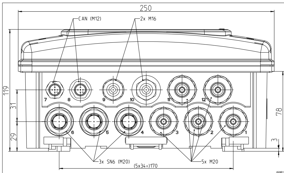
Fig. 16: All dimensions in millimetres (mm).
