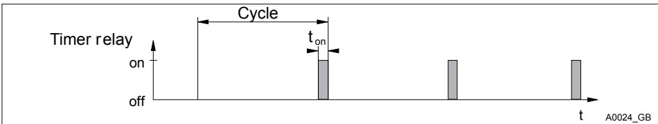
Fig. 106: Timer relay
