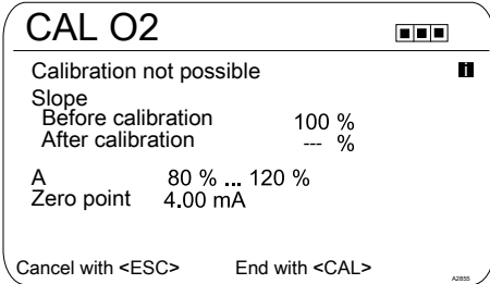
Fig. 73: Unsuccessful calibration
