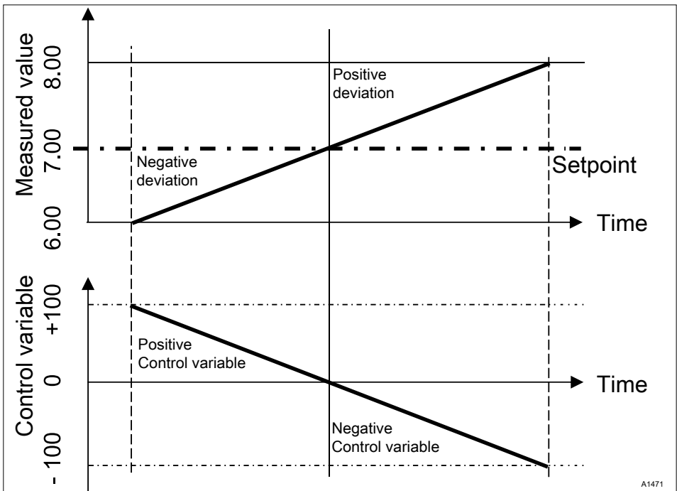
Fig. 86: Control type PID bidirectional. Control characteristic without neutral zone
