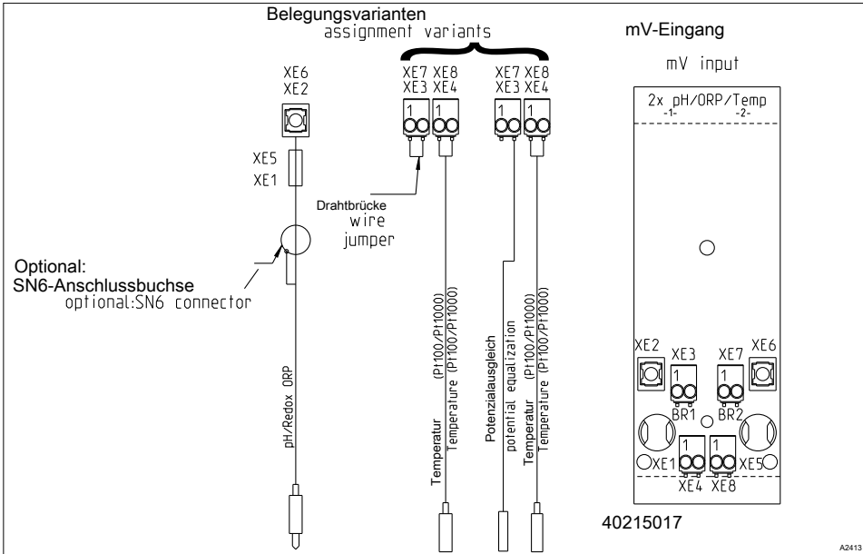
Fig. 25: Module: 2x mV inputs/temperature input. Part number 734131
