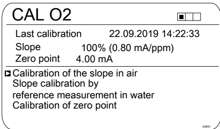
Fig. 69: Calibration of the slope in air
