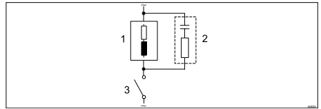
Fig. 29: RC protective circuit for the relay contacts
