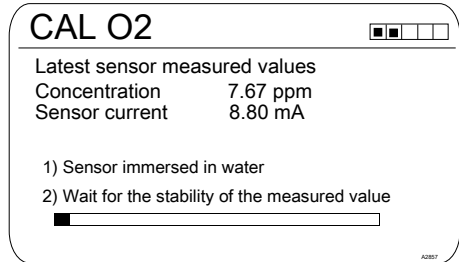
Fig. 75: Latest sensor measured values
