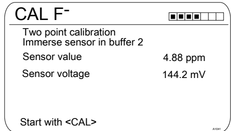
Fig. 60: Fluoride sensor calibration (CAL)
