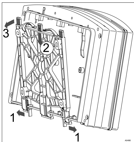
Fig. 12: Fitting surface mount
