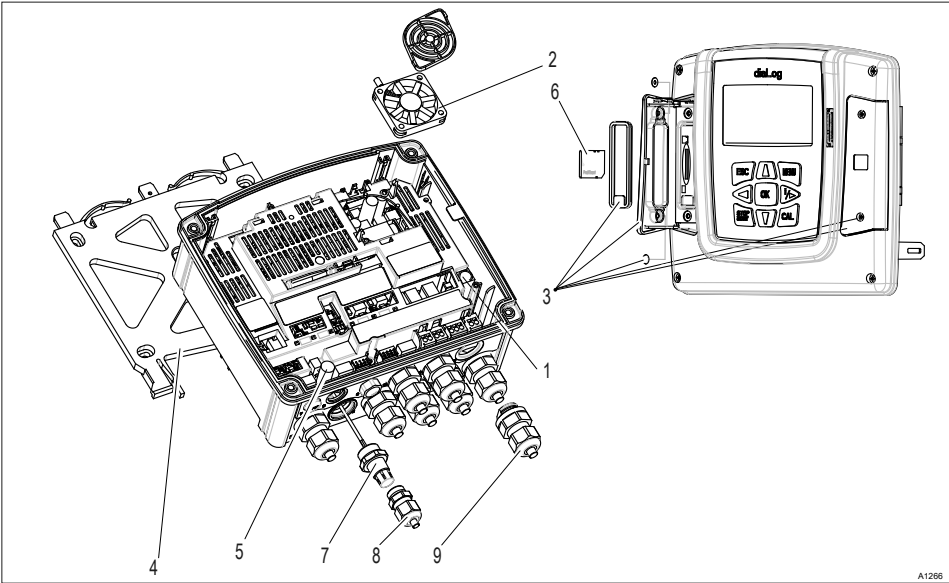
Fig. 127: Spare parts
