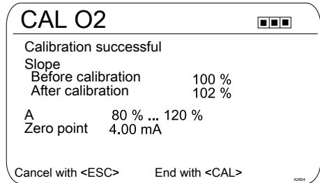
Fig. 82: Successful calibration
