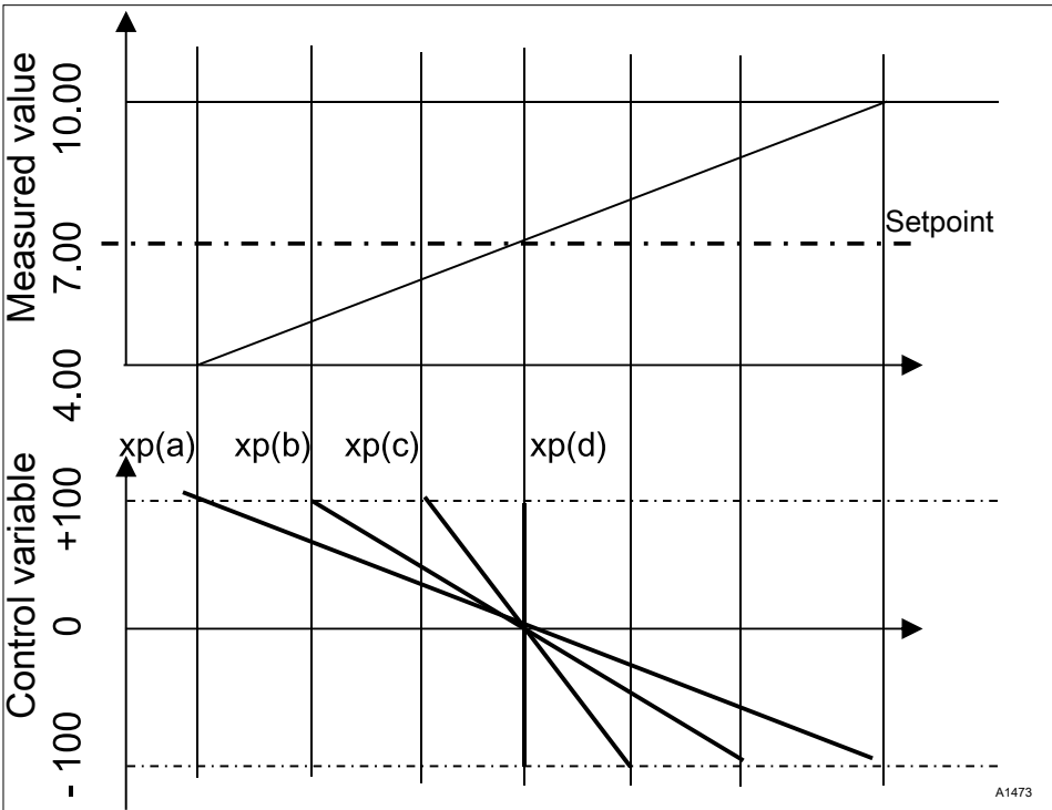
Fig. 90: The smaller the xp value, the more "forcefully" the control reacts.
