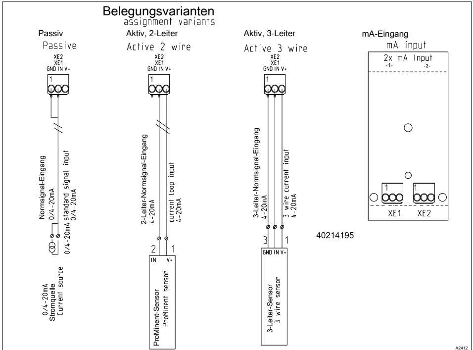
Fig. 27: Module: 2x mA inputs. Part number 734126
