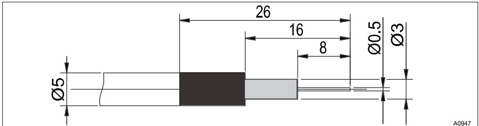
Fig. 31: Coaxial cable construction
