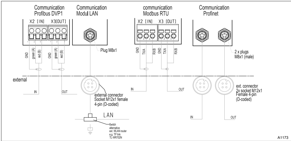
Fig. 22: Terminal diagram for the DAC communication unit (module B, optional)
