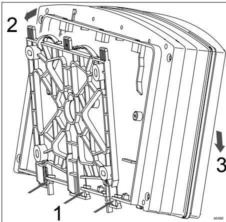
Fig. 13: Mounting surface mount
