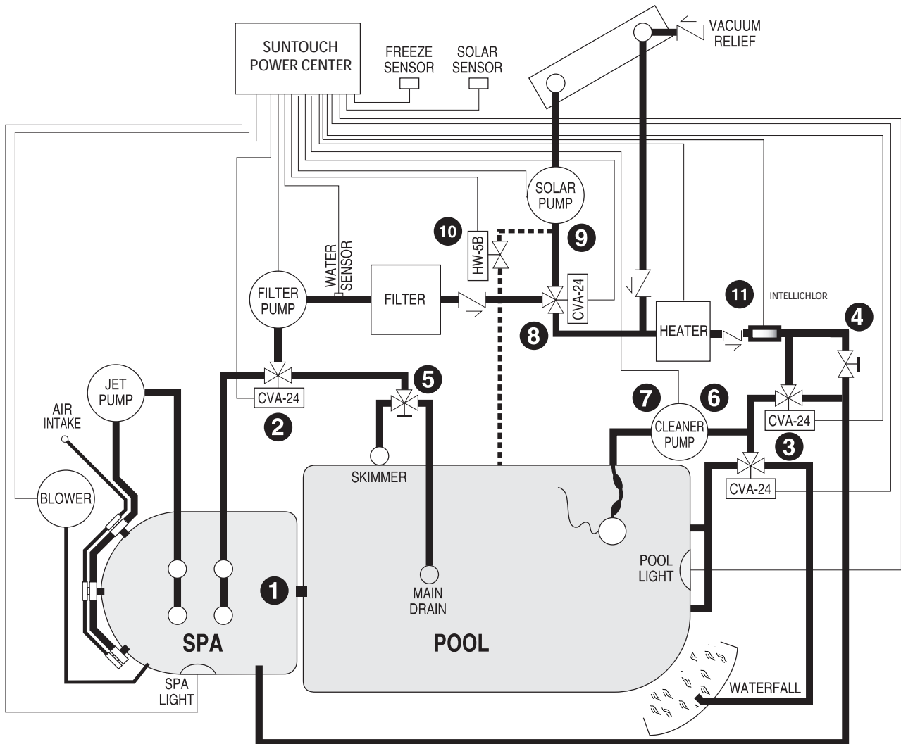
Recommended Hydraulic Schematic for Shared Equipment System
