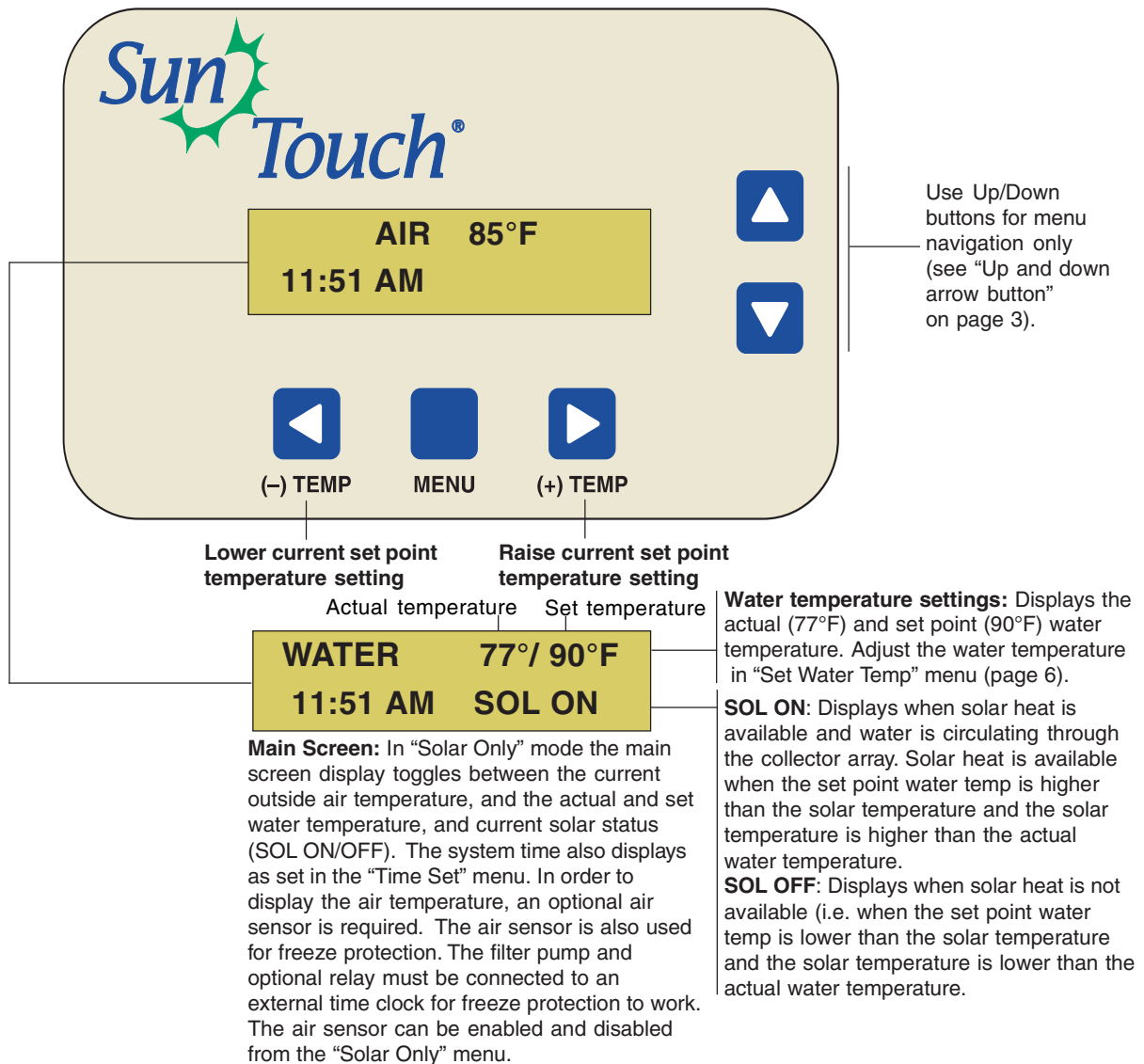
SunTouch Control Panel (Solar Only mode)
