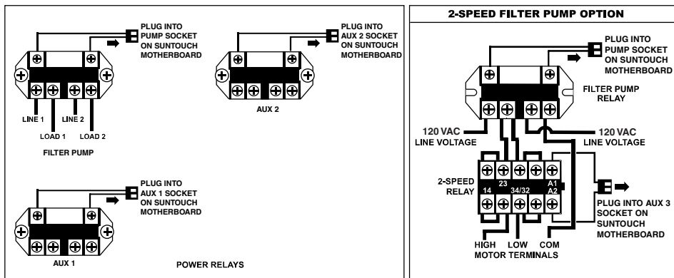
SunTouch Motherboard Connections
