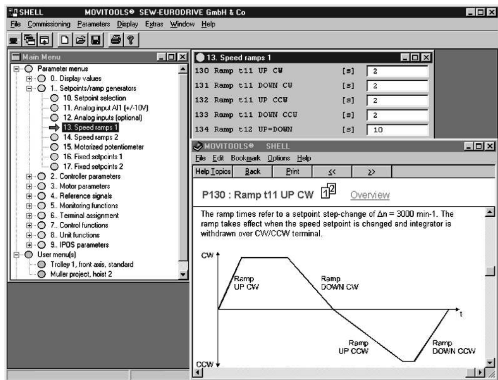
Figure 7: MOVITOOLS® window
