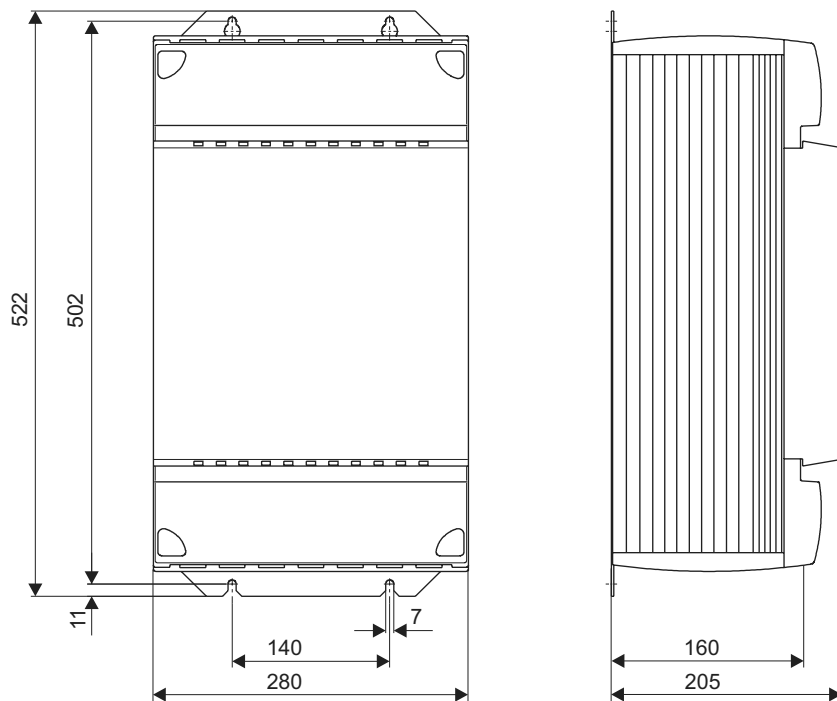
Figure 13: Dimension drawing for MDR60A size 4, dimensions in mm
