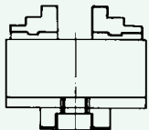
3-Jaw Lathe Chuck Self Centering Threaded Back Mount
