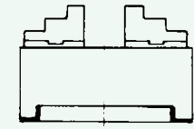
3-Jaw Lathe Chuck Self Centering Plain Recess Back
