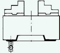
3-Jaw Lathe Chuck Self Centering "D-1" Camlock Mount
