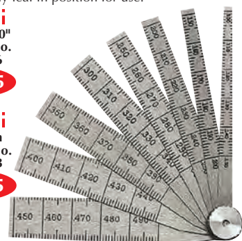
Starrett .001" Graduations
