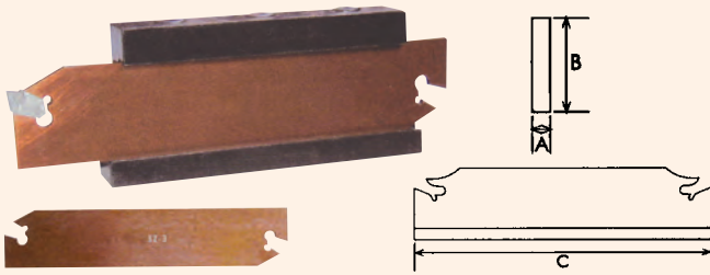
Individual Blades
