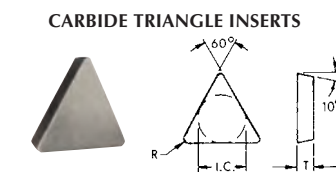
Positive Rake
