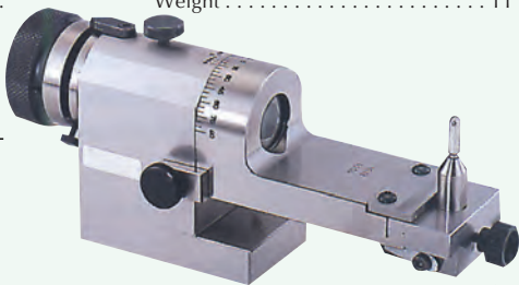
Grinding Wheel Dressing Application
