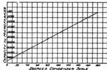
Calibration Curve of Condenser
