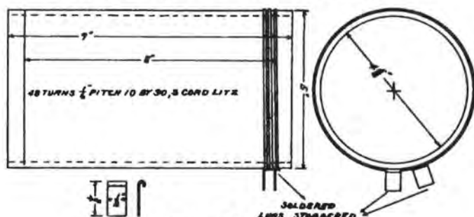
Fig. 36. Details of Variable Inductance.
