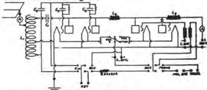
Fig. 33. Diagram of 10-Watt Phone Set.
