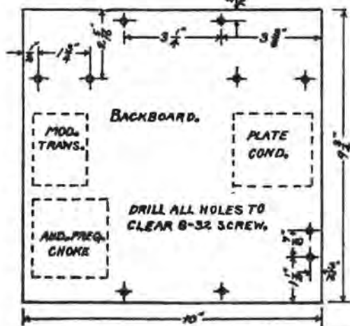
Fig. 37. Main Panel and Backboard Layout.
