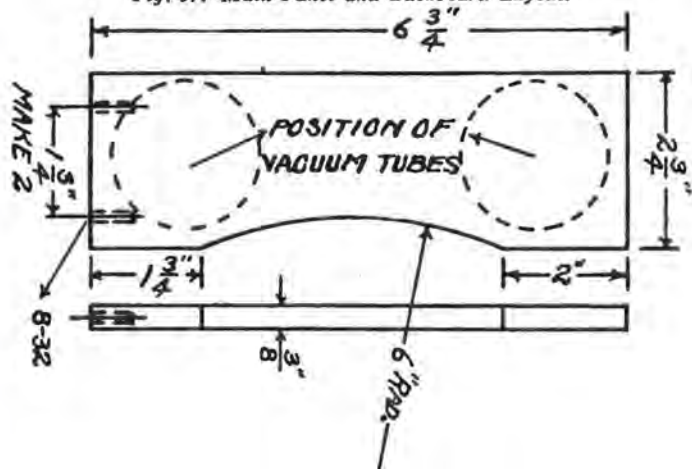
Fig. 38a. Layout of Sub-panel
