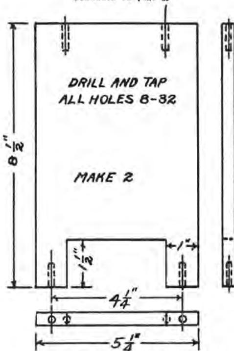
Fig. 38b. Layout of Sub-panel
