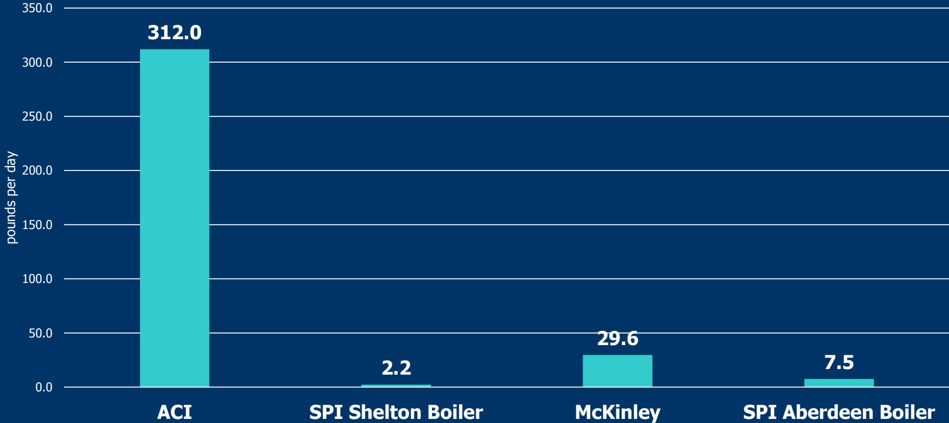
Air Curtain Incinerator Compared to Biomass Boilers in ORCAA's Region
