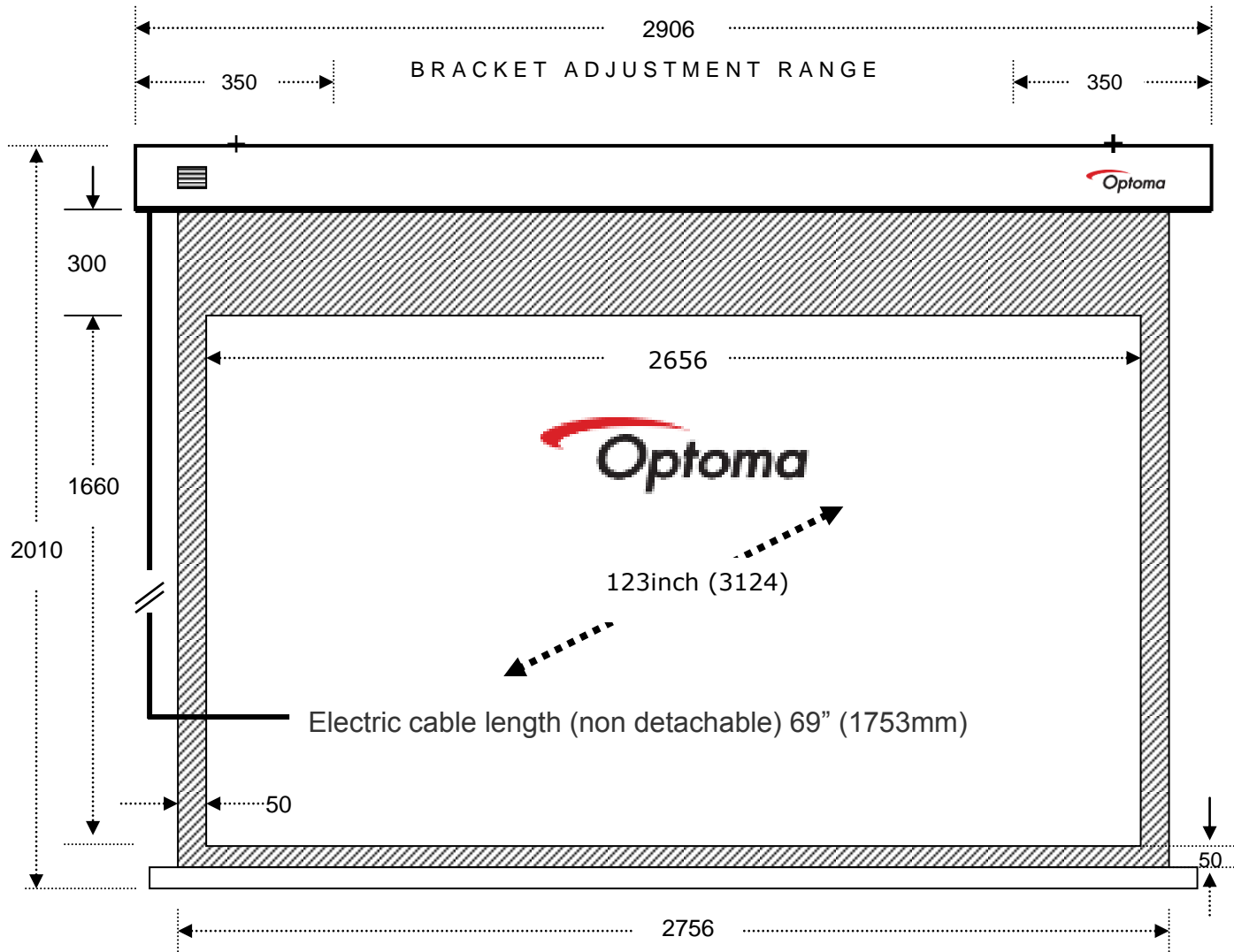
Optoma DE-1123EGA 16:10 ELECTRIC Measurements in Milimetres
