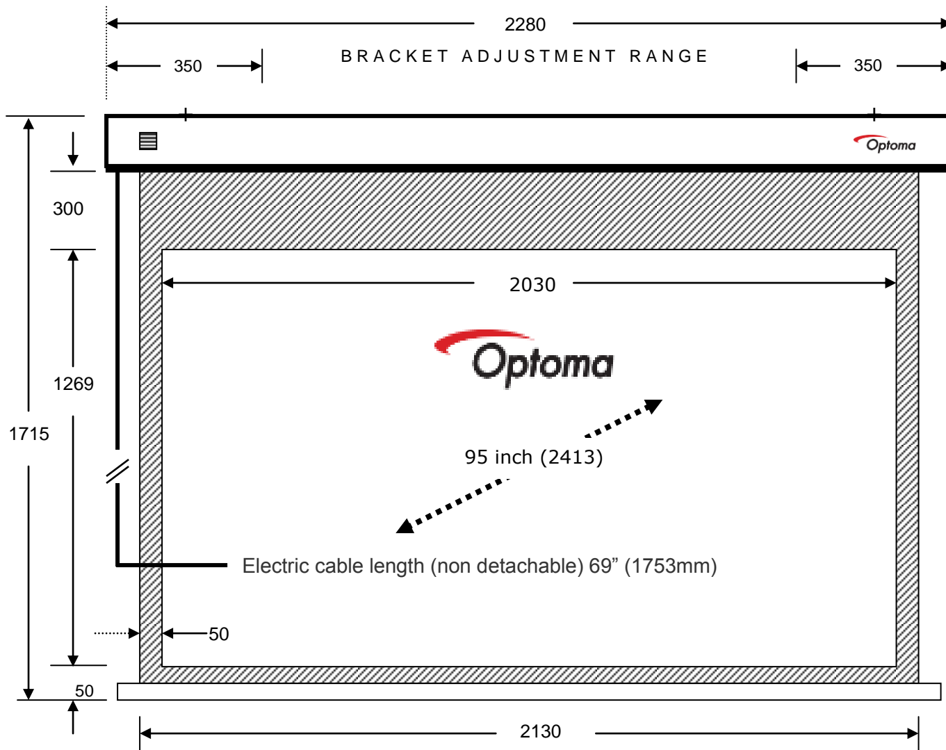
Optoma DE-1095EGA ELECTRIC Screen 16:10 Measurements in Milimetres
