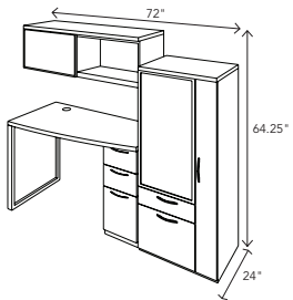
SH.T.001 Glass (above) or Laminate 72W 24D 64.25H
