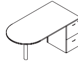
Two-Drawer Sales Desk 700_-3435 (R/L) 71W 35.5D 29H Consists of: -620 Exec Bullet Desk Shell -630 Bullet Support Base -832 F/F Pedestal
